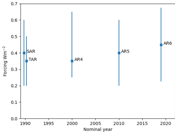
230 Figure 2. The tropospheric ozone radiative forcing from “pre-industrial” (1850 for SAR to AR4, 1750 for AR5 and AR6) to a nominal year assessed by the second (SAR) to sixth (AR6) IPCC Assessment Reports. Both SAR and TAR used ozone concentrations representative of 1990, but have been offset in the figure for clarity. For data and references see Table S1.
