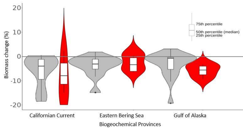
Figure 9: Biomass change associated with the Northeast Pacific MHW (2013-2016) per biogeochemical province. Grey violin plots correspond to results from Cheung & Frölicher, (2020), while the red ones corresponds to our hindcasted EcoTroph-Dyn simulation with \alpha=0.2 scenario. (Figure adapted from Cheung & Frölicher, (2020)).
