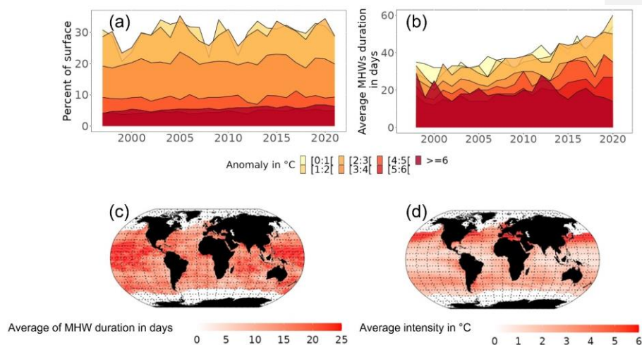
Figure 3: Temporal and spatial characteristics of MHWs identified for the period 1998 to 2021. (a) Changes in the percentage of the oceans' total surface area with MHW in each year. Evolution of spatial extent of MHWs categorised by their intensity, (b) Evolution of MHWs averaged duration categorised by their intensity, and (c) Average duration of each MHW event in days that occurred over the period 2015-2021. (d) Average intensity of each MHW event over the period 2015-2021. Average intensity of MHWs over the period 2015-2021. (d) Average number of MHWs over the period 2015-2021.
