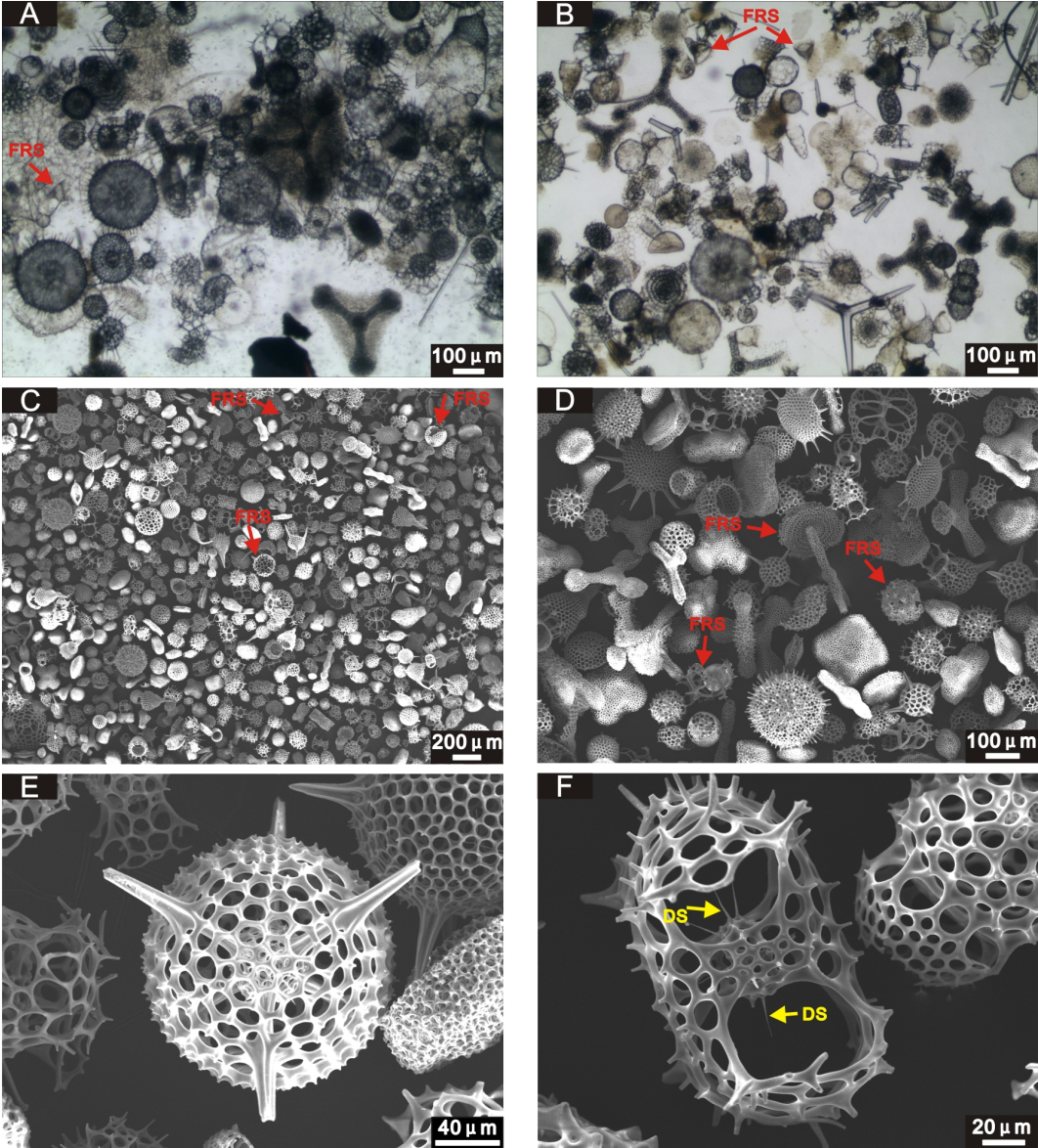
Figure 4. Observations of radiolarian shell preservation at station 12 (water depth: 3,497 m) in the plankton sample (100-300 m) (A and C) and surface sediments (B, D, E, and F) using optical microscope and the SEM. FRS=Fractured radiolarian shells; DS=Delicate skeletons.
