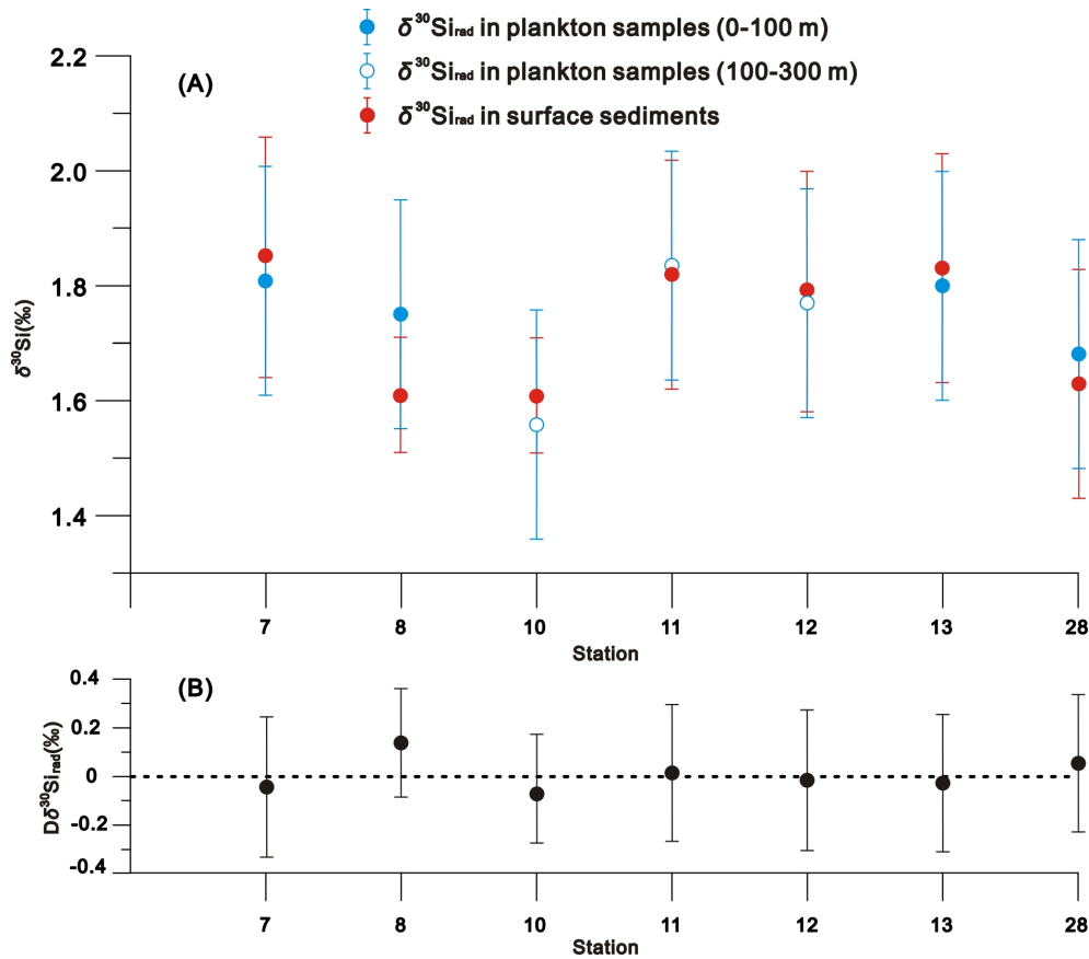
Figure 6. Comparison (A) and differences ( D\delta^{30}\text{Si}_{\text{rad}} ) (B) of \delta^{30}\text{Si}_{\text{rad}} values between plankton samples and surface sediments at each sampling station. The vertical bar denotes the analytical uncertainty ( 2\sigma ) of \delta^{30}\text{Si}_{\text{rad}} compositions in (A), and the combined uncertainty ( 2\sigma ) of D\delta^{30}\text{Si}_{\text{rad}} in (B). The horizontal dashed line in (B) represents the zero line, indicating no differences in \delta^{30}\text{Si}_{\text{rad}} compositions between plankton samples and surface sediments.
