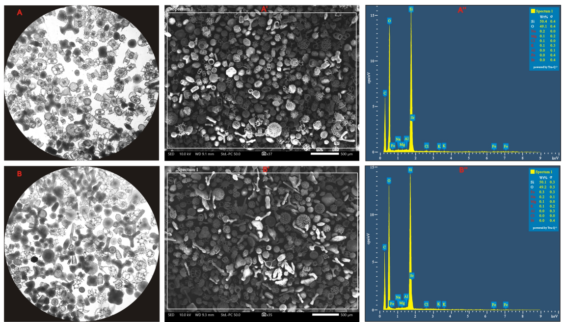
Figure 5. Pure radiolarian tests extracted from the plankton sample at station 8 (A) and the surface sediment at station 28 (B) under an inverted microscope at x100 magnification, as well as their SEM (A' and B') and EDS (A'' and B'') spectrum images.
