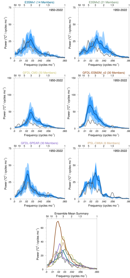
Figure 6. ENSO (nino3.4) monthly power spectrum for Set 2 models. The dark blue curve shows the model's ensemble mean timeseries power spectrum , and the dark (light) blue shading around this curves depicts the 25th-75th (10th-90th) percentile spread across the ensemble members and the grey/brown line is the observations. The bottom right shows the ensemble mean from each model and the observations on a single panel. Computations are completed over the period 1950-2022. Power spectra are computed in variance preserving format from the linearly detrended December Nino3.4 SST Index (SST anomalies averaged over the region 5N-5S, 170W-120W). Observations are detrended using a quadratic fit, while LEs are detrended by removing the ensemble mean. Set 1 & 3 can be found here: https://webext.cgd.ucar.edu/Multi-Case/MMLEA_v2/MMLEA_Set1_quadrmEM_1950-2022/nino34.powspec.summary.png & https://webext.cgd.ucar.edu/Multi-Case/MMLEA_v2/MMLEA_Set3_quadrmEM_1950-2022/nino34.powspec.summary.png
