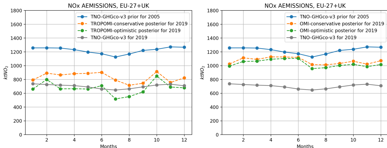
Figure 10. Left) January to December 2019 times series of monthly estimates of anthropogenic NO x prior emissions from the TNO-GHGco-v3 inventory for the year 2005 (in blue), posterior anthropogenic NO x emission estimates from the TROPOMI-conservative (in orange) and TROPOMI-optimistic (in green) inversions, in kteqNO 2 , for the EU-27+UK area. Right) same as left, but for posterior anthropogenic NO x emission estimates from the OMI-conservative (in orange) and OMI-optimistic (in green) inversions.
