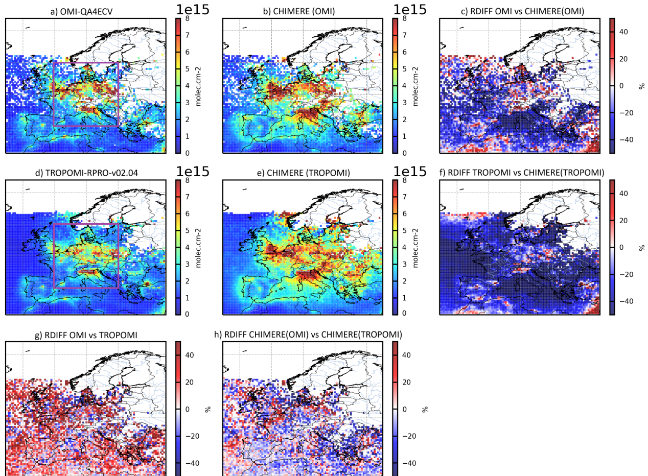
Figure 7. Monthly averages of NO 2 a) super-observations based on OMI and b) the CHIMERE-OMI simulation, where and when OMI-QA4ECV super-observations are available; d) super-observations based on TROPOMI-RPRO-v02.04 and e) CHIMERE-TROPOMI simulations, where and when TROPOMI super-observations are available, in molec.cm -2 . Monthly averages for January 2019 of the relative differences between c) the super-observations from OMI-QA4ECV NO 2 TVCDs and the CHIMERE-OMI simulation, f) the super-observations from TROPOMI NO 2 TVCDs and the CHIMERE-TROPOMI simulation, g) the OMI and TROPOMI super-observations and h) the CHIMERE-OMI and the CHIMERE-TROPOMI simulations, in %. The prior TNO-GHGco-v3 anthropogenic emission for the year 2005 are used to simulate the NO 2 TVCDs. The purple box shows Western and Central Europe (0°E-20°E; 40°N-60°N).
