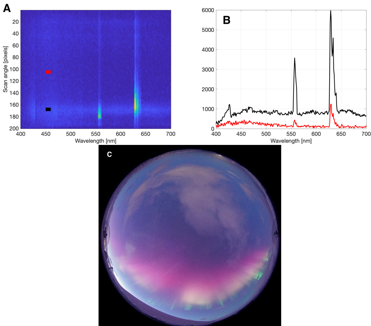
Figure 12. A: MISS spectrogram data at 05:46 UT on 11 February 2024 with the meridian locations of the reference spectrum (red) and the continuum spectrum (black). B: Continuum spectrum (black) and an empty sky reference spectrum (red) measured at 05:46 UT. The y-axis values are summed counts over scan angles of 163–173 for the continuum and over scan angles of 100–110 for the reference. C: ASC image taken at 05:46:03 UT. North is to the top and east to the left of the image. The solar elevation angle was -12^\circ relative to the horizon with an azimuth of 102^\circ (ESE) and the sunlit boundary of the ionosphere was at 142 km.
