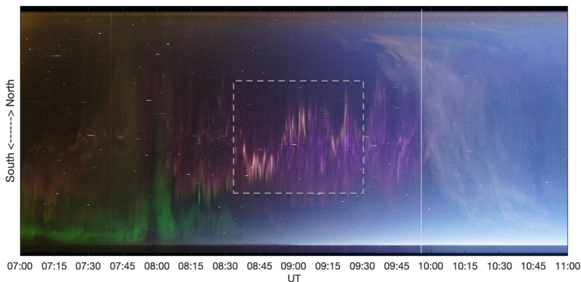
Figure 2. Keogram of Sony images at 07–11 UT on 3 January 2020. The y-axis is a slice through the sky from magnetic South (bottom) to magnetic North (top). The most intense pale pink continuum emission is seen in the time period of 08:30–09:30 UT indicated by the rectangle. Appearance of a thin cloud layer is marked by vertical line.
