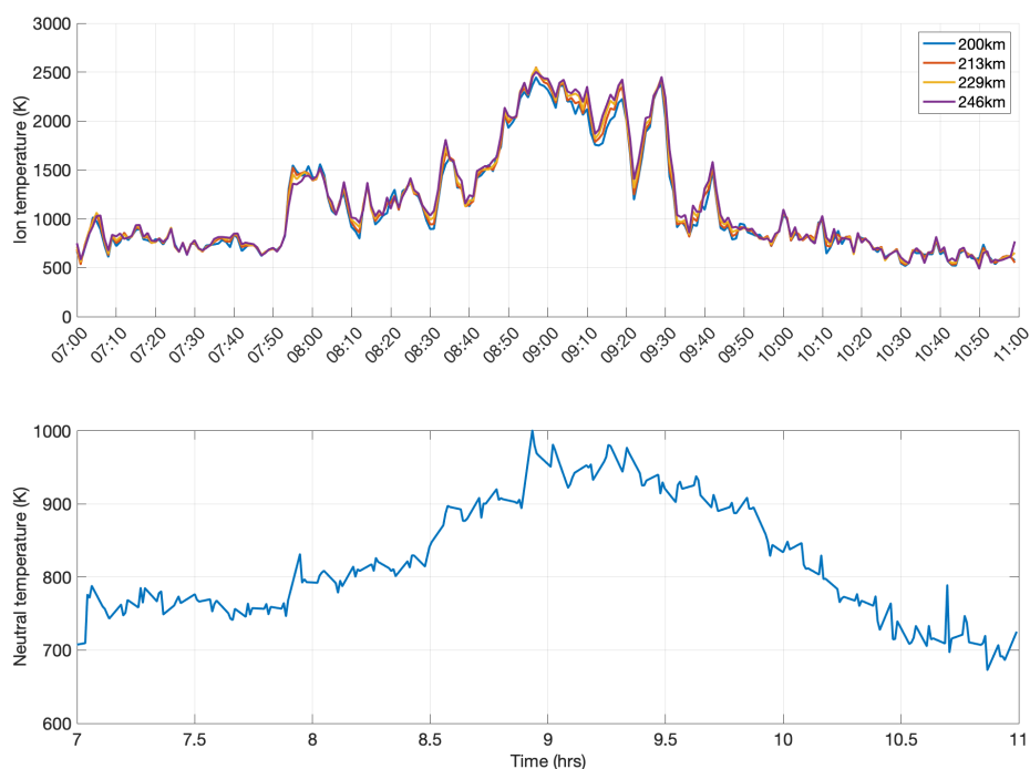
Figure 9. F region ion temperature measurements by ESR (top panel) at the heights of 200, 213, 229 and 246 km on 3 January 2020. Thermospheric neutral temperature measured by FPI (bottom).
