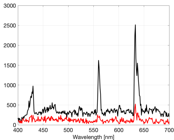
Figure 4. Continuum spectrum (black) and an empty-sky reference spectrum (red) measured by MISS at 08:49 UT on 3 January 2020. The y-axis values are counts summed over scan angles around the continuum maximum (118–128) and scan angles of 80–90 for the reference spectrum. The solar elevation angle was about -13^\circ and the ionosphere above about 160 km altitude was sunlit.
