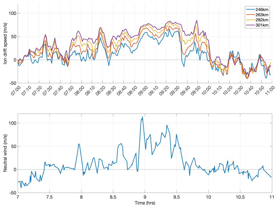
Figure 10. F-region ion drift speed measurements by the ESR (top panel) at the heights of 246, 263, 282 and 301 km on 3 January 2020. Thermospheric neutral upflow speed (vertical line-of-sight) measured by the FPI (bottom). Positive speed is upwards in both measurements.
