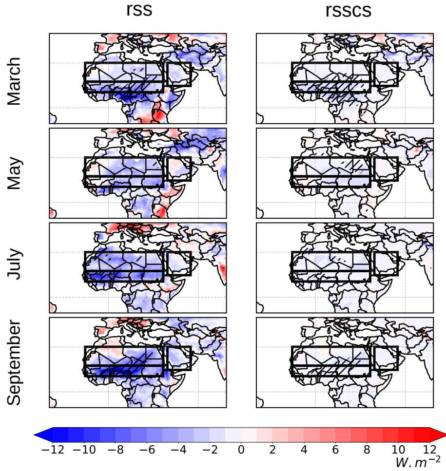
Figure A4. Same as Figure A3 but for rss (net downward SW surface radiation, rss = r_{sds} - r_{sus} , W m^{-2} ) and rsscs (net downward SW surface radiation in clear-sky conditions, W m^{-2} ).
