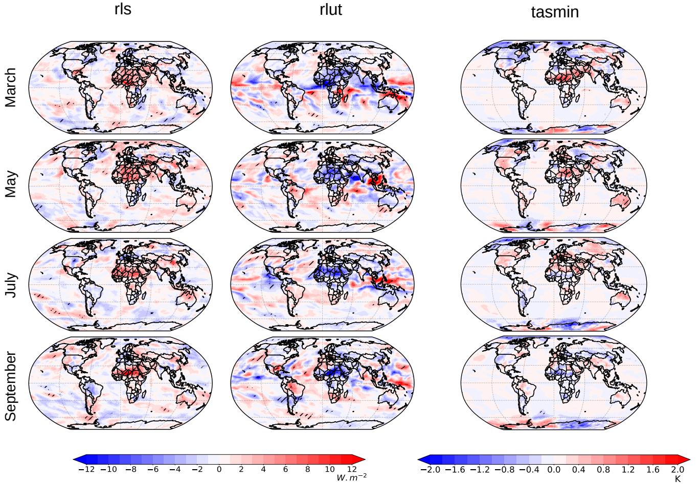
Figure A2. Changes (1985-2014), at the global scale, between the LWAS and NOLWAS simulations (LWAS minus NOLWAS) in rls (net downward LW surface radiation, rls = rlds - rlus , W \cdot m^{-2} ), rlut (TOA outgoing LW radiation, W \cdot m^{-2} ) and tasmin (minimum surface temperature, K) for the months of March (1st line), May (2nd line), July (3rd line) and September (4th line). Hatching indicates regions with a significant effect at the 0.05 level (Student's t-test).
