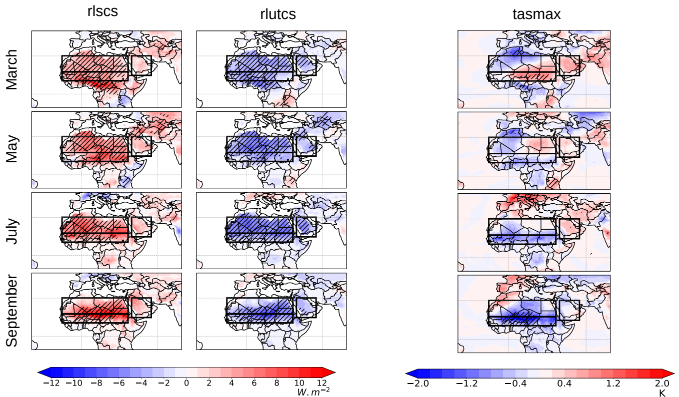
Figure A3. Same as Figure 4 for rlscs (net downward LW surface radiation in clear-sky conditions, W m^{-2} ), rlutcs (TOA outgoing LW radiation in clear-sky conditions, W m^{-2} ) and tasmax (maximum surface temperature, K) for the months of March (1st line), May (2nd line), July (3rd line) and September (4th line). Hatching indicates regions with a significant effect at the 0.05 level (Student's t-test).
