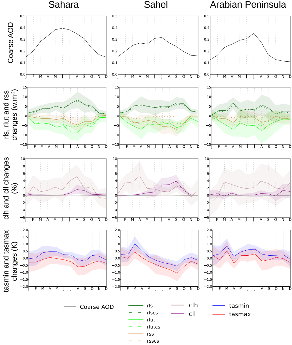
Figure 5. Annual cycle in coarse AOD (550 nm) and annual (1985-2014) cycles of changes in rls (net downward LW surface radiation, \text{rls} = \text{rlds} - \text{rlus} , \text{W m}^{-2} ), rlut (TOA outgoing LW radiation, \text{W m}^{-2} ), rss (net downward SW surface radiation, \text{rss} = \text{rlds} - \text{rsus} , \text{W m}^{-2} ), clh and cll (high, above 440 hPa, and low, below 640hPa, troposphere cloud area fraction, %) changes and tasmax and tasmin changes (maximum and minimum surface temperature, K) between the LWAS and NOLWAS simulations (LWAS minus NOLWAS) over three regions: Sahara, Sahel and Arabian Peninsula. Confidence intervals indicated in light color (Student's t-test, 0.05 level).
