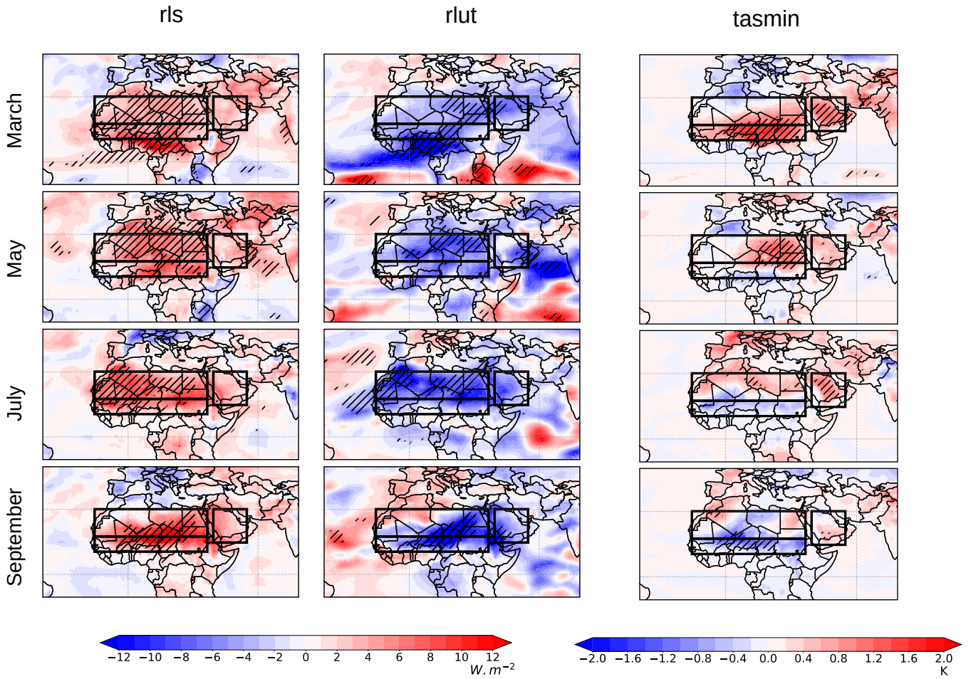
Figure 4. Same as in Figure 3 for rls (net downward LW surface radiation, rls = rlds - rlus with rlds the downward LW surface radiation and rlus the upward LW surface radiation, W m^{-2} ), rlut (TOA outgoing LW radiation, W m^{-2} ) and tasmin (minimum surface temperature, K).
