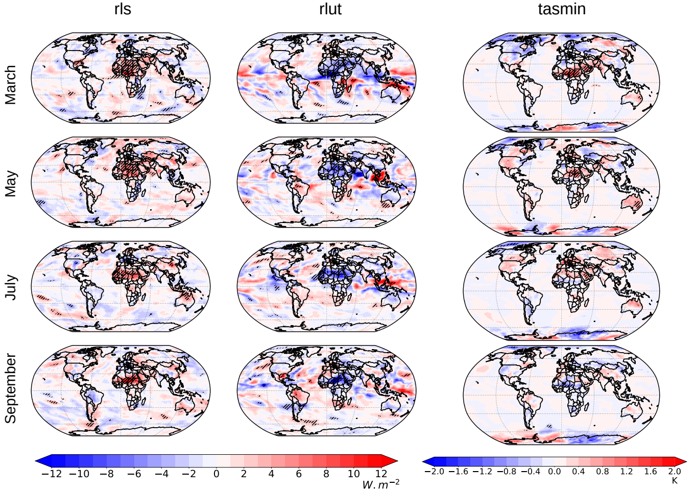
Figure A2. Changes (1985-2014), at the global scale, between the LWAS and NOLWAS simulations (LWAS minus NOLWAS) in rls (net downward LW surface radiation, \text{rls} = \text{rlds} - \text{rlus} , \text{W m}^{-2} ), rlut (TOA outgoing LW radiation, \text{W m}^{-2} ) and tasmin (minimum surface temperature, K) for the months of March (1st line), May (2nd line), July (3rd line) and September (4th line). Hatching indicates regions with a significant effect at the 0.05 level (Student's t-test).
