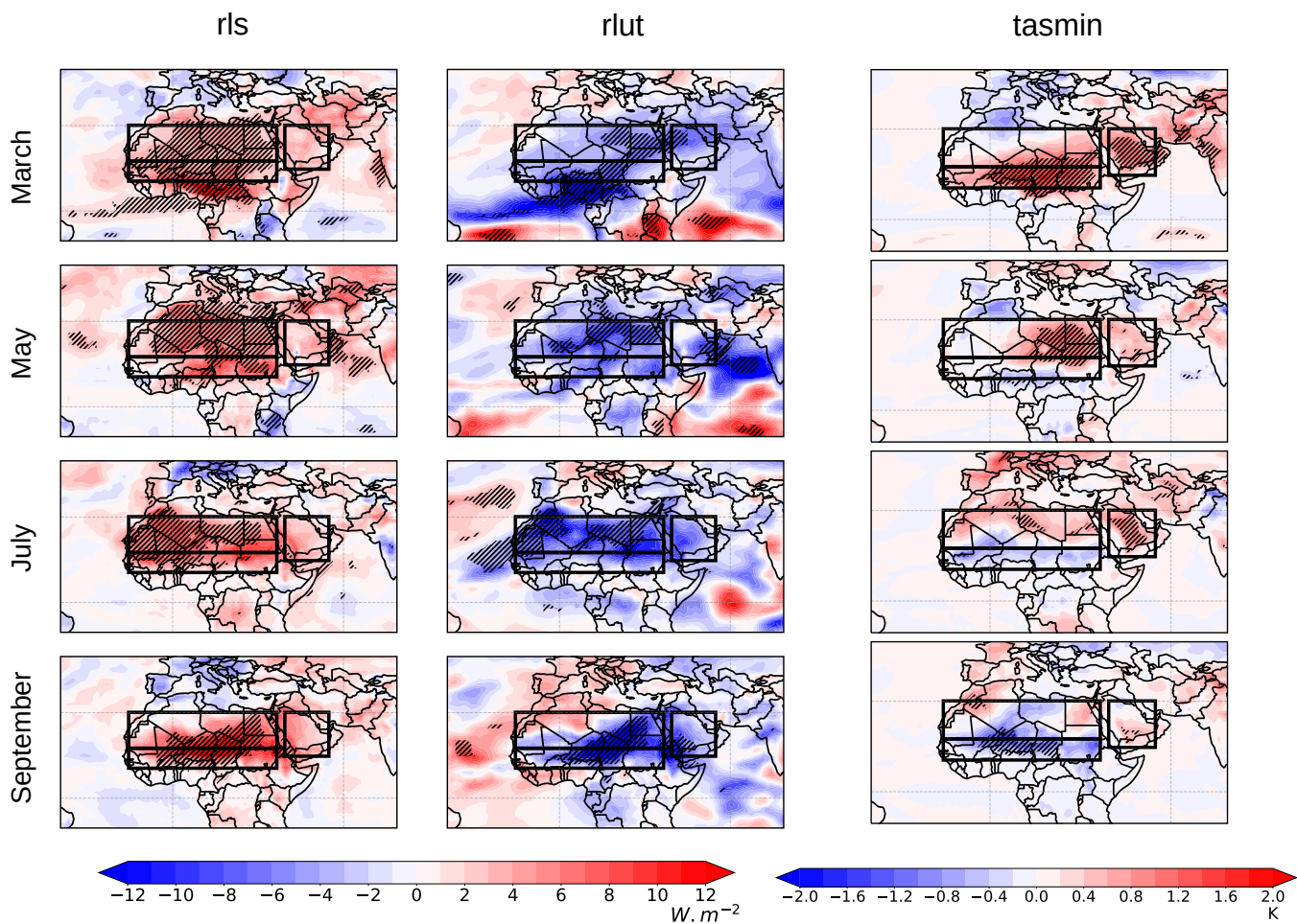
Figure 4. Same as in Figure 3 for rls (net downward LW surface radiation, \text{rls} = \text{rlds} - \text{rlus} with rlds the downward LW surface radiation and rlus the upward LW surface radiation, \text{W m}^{-2} ), rlut (TOA outgoing LW radiation, \text{W m}^{-2} ) and tasmin (minimum surface temperature, K).
