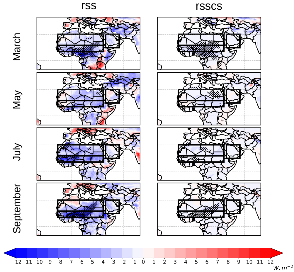
Figure A4. Same as Figure A3 but for rss (net downward SW surface radiation, rss = r_{sds} - r_{sus} , W m^{-2} ) and rsscs (net downward SW surface radiation in clear-sky conditions, W m^{-2} ).
