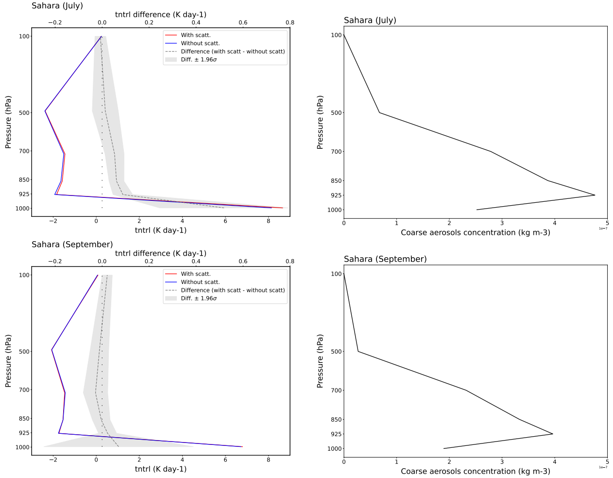
Figure A7. LW heating rate (tntrl) vertical profiles over the Sahara region in July and September for the LWAS (red) and NOLWAS (blue) simulations. Difference between these two simulations (LWAS minus NOLWAS) is shown in grey. Confidence intervals for no significant changes indicated in grey light color (Student's t-test, 0.05 level). Associated coarse aerosols concentration vertical profiles are shown on the right.
