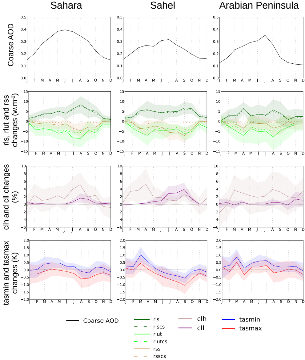
Figure 5. Annual cycle in coarse AOD (550 nm) and annual (1985-2014) cycles of changes in rls (net downward LW surface radiation, rls = rlds - rlsu , W m^{-2} ), rlut (TOA outgoing LW radiation, W m^{-2} ), rss (net downward SW surface radiation, rss = rlds - rlsu , W m^{-2} ), clh and cll (high, above 440 hPa, and low, below 640hPa, troposphere cloud area fraction, %) changes and tasmax and tasmin changes (maximum and minimum surface temperature, K) between the LWAS and NOLWAS simulations (LWAS minus NOLWAS) over three regions: Sahara, Sahel and Arabian Peninsula. No significant changes in confidence intervals indicated in light color (Student's t-test, 0.05 level).
