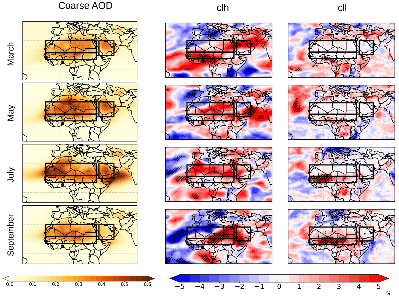
Figure 3. Coarse AOD (550 nm, left column) and mean differences (1985-2014) between the LWAS and NOLWAS simulations (LWAS minus NOLWAS) in cloud area fraction (%), at high (above 440 hPa, middle column), and low (below 640hPa, right column) altitudes (clh and cll, respectively), for the months of March (1st line), May (2nd line), July (3rd line) and September (4th line). Hatching indicates regions with a significant effect at the 0.05 level (Student's t-test).
