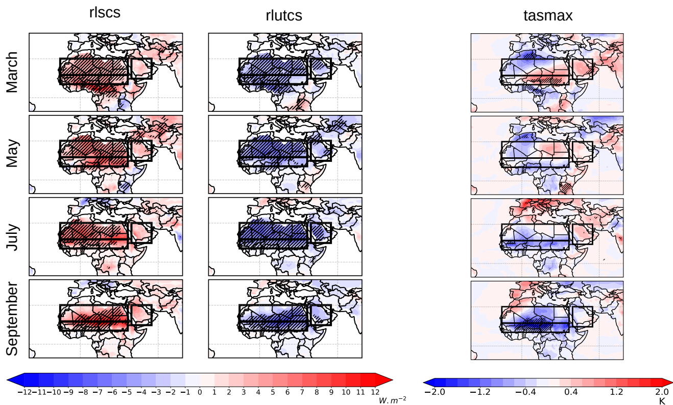
Figure A3. Same as Figure 4 for rlscs (net downward LW surface radiation in clear-sky conditions, \text{W m}^{-2} ), rlutcs (TOA outgoing LW radiation in clear-sky conditions, \text{W m}^{-2} ) and tasmax (maximum surface temperature, K) for the months of March (1st line), May (2nd line), July (3rd line) and September (4th line). Hatching indicates regions with a significant effect at the 0.05 level (Student's t-test).
