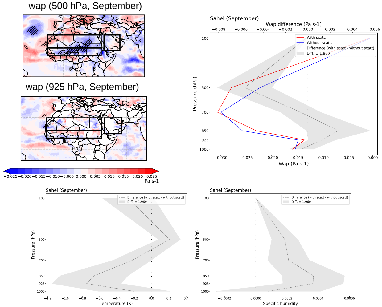
Figure A6. Mean differences (1985-2014) between the LWAS and NOLWAS simulations (LWAS minus NOLWAS) in vertical velocity (wap, 500 and 925 hPa, top left). Vertical profiles of vertical velocity (top right), temperature (bottom left) and specific humidity (bottom right) over the Sahel in September for the LWAS (red) and NOLWAS (blue) simulations. Difference between these two simulations (LWAS minus NOLWAS) is shown (dashed grey line). Confidence intervals for no significant changes indicated in grey light color (Student's t-test, 0.05 level).
