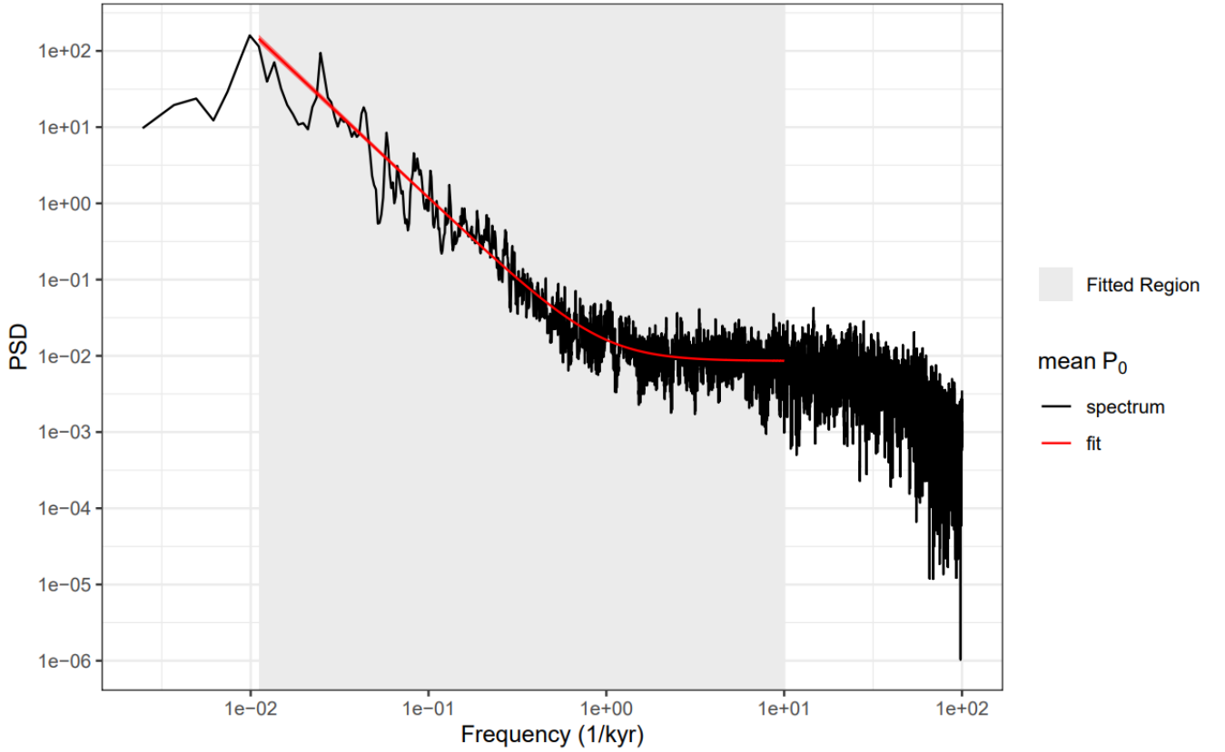
Figure 2. P_0 - P_0(f) fit (red) over the grey shaded region of a composite power spectrum of the EDC water isotope record (black). By excluding high frequencies attenuated by firm diffusion, this fit serves as a good approximation of the initial isotopic variability of the BE-OIC
