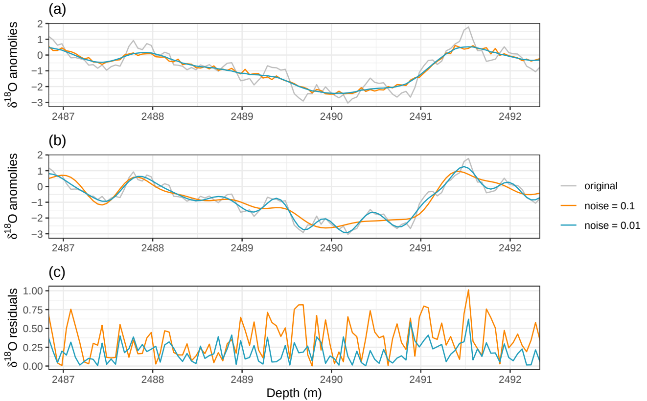
Figure 7. Example of the effect of the measurement noise level on the deconvolution in the depth domain for deep ice. (a) The true, undiffused record (grey) and two diffused records ( \sigma=0.15 - \sigma=0.21 m) with measurement noise standard deviations of 0.1‰ (orange) and 0.01‰ (blue). (b) Deconvolutions of the two diffused records in (a). (c) Residuals between the original and deconvolved records.
