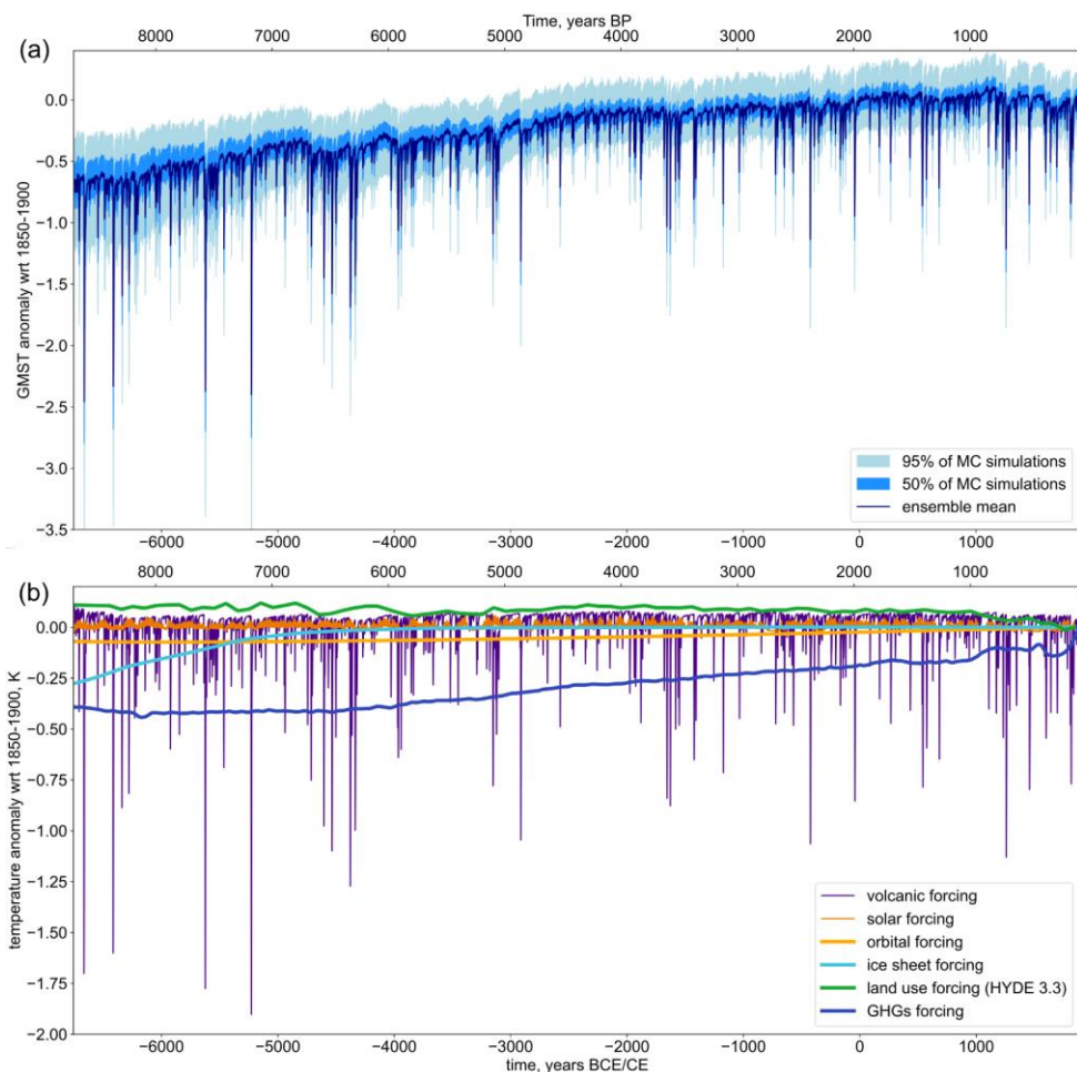
425 Figure 4: a. GMST from the full simulation ensemble (Sect. 3), expressed as an anomaly with respect to 1850-1900 CE; b. Simulated GMST with only one set of forcing varying, and all other ones set to their 6755 BCE value. The EVA_H and FaIR models were FaIR is run using a single set of model parameters. Best estimates were used for volcanic injection parameters. The volcanic forcing corresponds to the 1000-member ensemble mean ERF.
