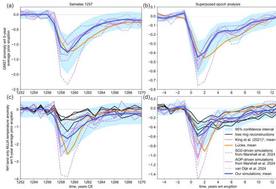
Figure 7: a. GMST response to Samalas 1257 eruption from our simulations compared to simulations from Marshall et al. (2024 5 ) and Lücke et al. (2023); b. superposed epoch analysis of the GMST response to 14 eruptions injecting more than 20 Tg of SO 2 that occurred between 1250 and 1850; c. NH land only MJJA temperature response to Samalas compared to tree-ring-based reconstructions (NTREND 2015, Schneider 2015, Guillet 2017, Büntgen 2021, King et al., 2021) and simulations from Lücke et al. (2023) and Marshall et al. (2024 5 ); d. Superposed epoch analysis of the NH land only MJJA temperature response. *Note that King et al.'s reconstruction corresponds to land and sea mean temperature, whereas other reconstructions are land only.
