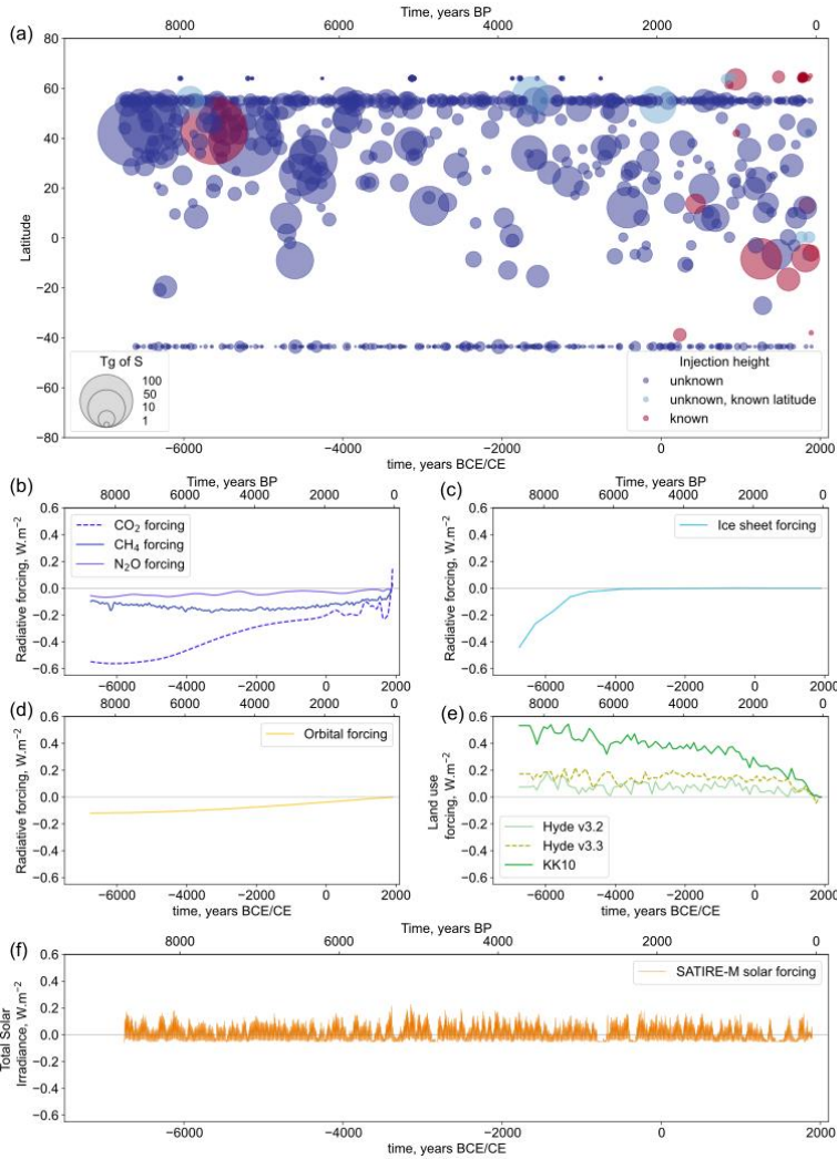
Figure 1: Forcings used in our study; a. Spatiotemporal distribution of volcanic stratospheric sulfur injections, injection heights are constrained from isopleth maps for most of the eruptions for which we have data (Table S1); b. Greenhouse gases forcing (CH 4 , N 2 O, CO 2 ); c. Net ice sheet forcing; d. Orbital forcing; e. Land-use forcing; f. Solar forcing; f. Spatiotemporal
