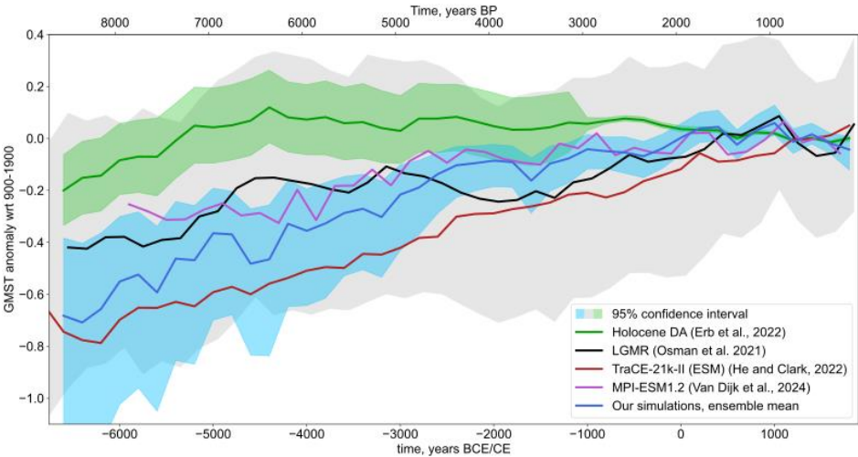
Figure 5: Comparison of our simulated 200-year-smoothed temperatures to the LGMR (Osman et al., 2021), Holocene DA (Erb et al., 2022) , MPI-ESM1.2 (van Dijk et al., 2024) and TraCE-21k-II (He and Clark, 2022), expressed as an anomaly with respect to the last millennium mean temperature.
