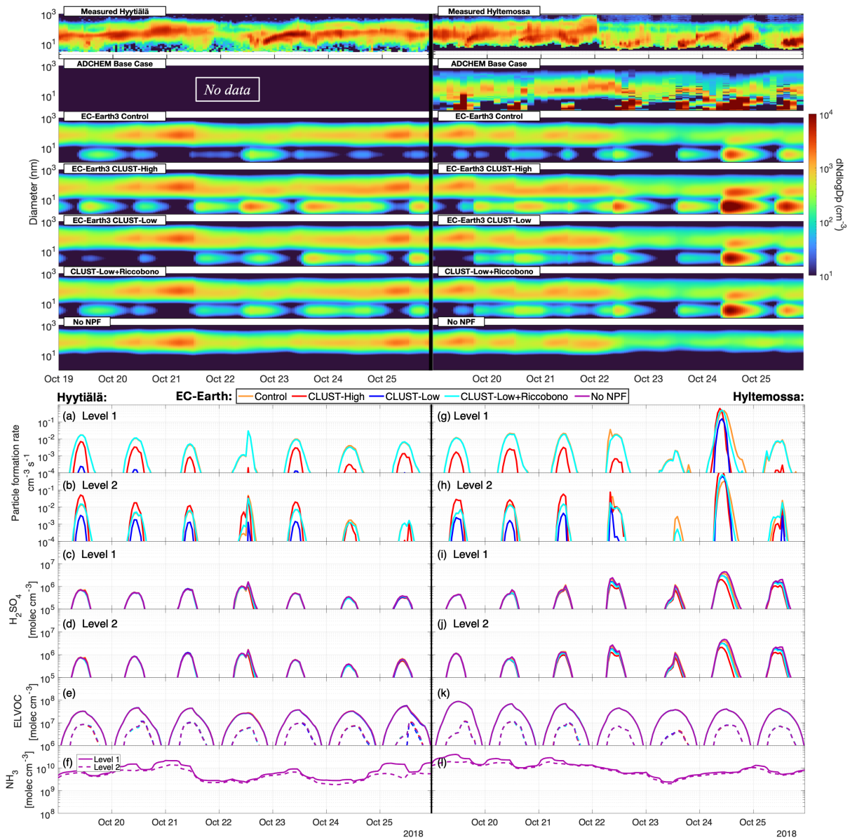
Figure A7. The top two figures show the surface aerosol number size distribution over the autumn period for the 5 modelled EC-Earth3 cases, with the DMPS measured aerosols at Hyttiälä and Hyltemossa. ADCHEM simulations have no available hourly data outside the autumn months for Hyttiälä. The bottom section shows EC-Earth3 modelled layer 1 and layer 2 Hyttiälä and Hyltemossa autumn cases showing (a, b, g, h) daily maximum particle formation rate, (c, d, i, j) \text{H}_2\text{SO}_4 , (e, k) ELVOC, (f, l) and \text{NH}_3 gas concentration. The concentrations for ELVOC and \text{NH}_3 level 2 are shown as dotted lines in e, f, k, l. The missing particle formation rates below 10^{-4} in panel a, b, g, and h are considered practically zero.
