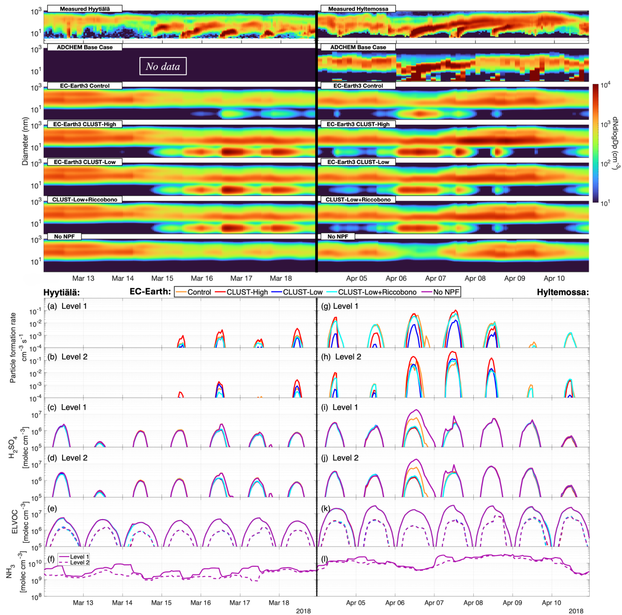
Figure 3. Surface The top two figures shows the surface aerosol number size distribution over the springtime for the 5 modelled EC-Earth3 cases, with the DMPS measured aerosols at Hyttiälä and Hyltemossa. ADCHEM simulations have no available hourly data outside the Summer months for Hyttiälä. The bottom section shows EC-Earth3 modelled layer 1 and layer 2 Hyttiälä and Hyltemossa springtime cases showing (a, b, g, h) daily maximum particle formation rate, (c, d, i, j) \text{H}_2\text{SO}_4 , (e, k) ELVOC, (f, l) and \text{NH}_3 gas concentration. The concentrations for ELVOC and \text{NH}_3 level 2 are shown as dotted lines in e, f, k, l. The missing particle formation rates below 10^{-4} in panel a, b, g, and h are considered practically zero.
