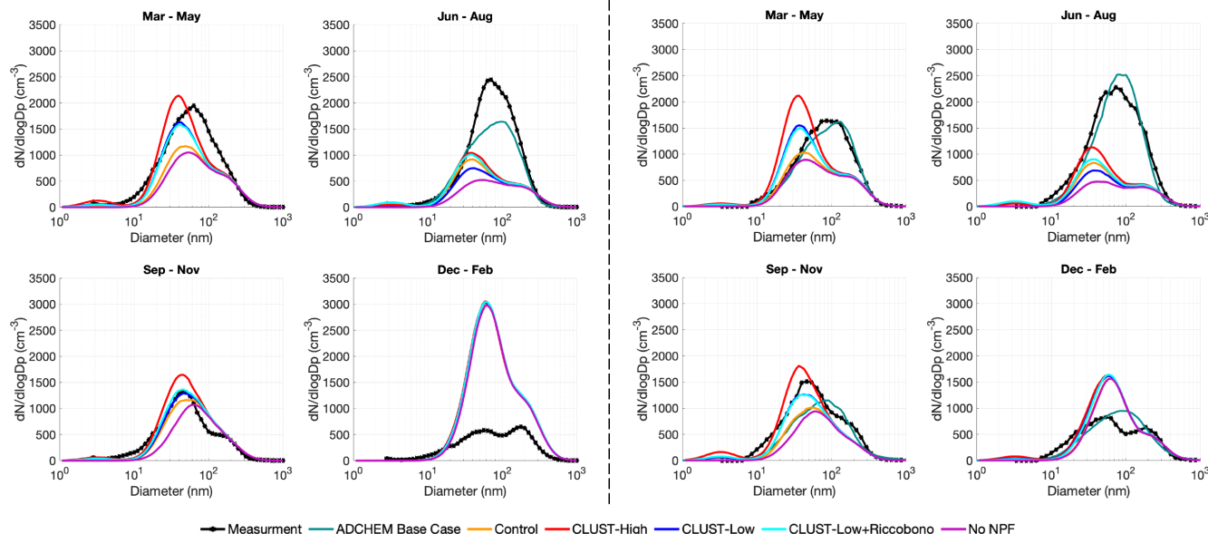
Figure 1. The seasonal median size distribution for the five EC-Earth3 variants, the ADCHEM simulations, and the observations. Note, the ADCHEM model only generated output from May to August for Hyytiälä and thus is only shown for Jun-Aug.
