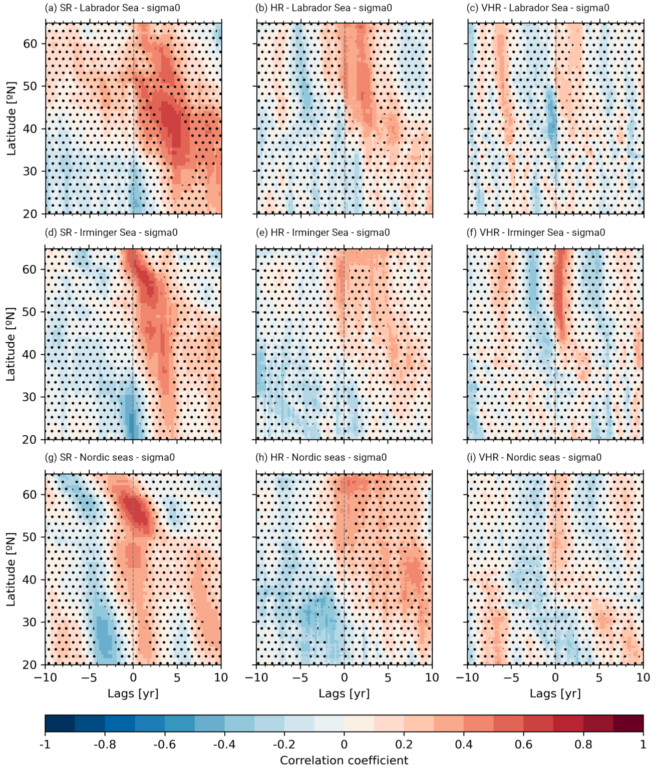
Supporting Figure 3: Correlation of monthly volume overturning stream function without the Ekman transport at 36.73 \text{ kg m}^{-3} sigma2 density level with March surface sigma0 at Labrador Sea (a, b, c), Irminger Sea (d, e, f), and Nordic Seas (g, h, i). For positive lag values, March MLD leads. Non-significant values are masked with dots to improve the visibility of the significant regions
