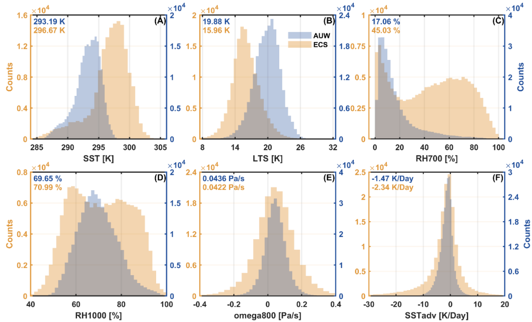
Figure 2. 4 year meteorological conditions of non-precipitation clouds in AUW and ECS region from 2016 to 2019. Histograms of meteorological factors are presented here.
