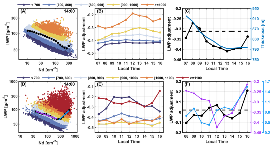
Figure 1. LWP adjustments in log-log spaces and their diurnal patterns in two typical regions (the west of Australia, AUW) and the east China sea, ECS). Non-precipitation cloud samples are scattered in N_d -LWP log space at 1400 LT in (A) AUW and (D) ECS region. Colored dots are samples in different cloud thickness (H) bins (unit: m). Black dots represent the median LWP in each N_d bin. The colored lines are the fits of black dots at different stages: in ECS region . Diurnal variations of LWP adjustments binned by H in (B) AUW and (E) ECS regionregions are showedshown . Colored lines in (C) and (F) are diurnal variations of different stages in (A) and (D), while black lines in (C) and (F) are the overall diurnal variations of LWP adjustments in two regions, respectively. The incompletion of greenblue line in (F) is because the processes are not obvious at 0800 LT and 1600 LT . (C) represents the diurnal variation of H . Dashed lines represent the average LWP adjustments considering diurnal variations, -0.4931 for AUW (C) and 0.3302 for ECS (F).
