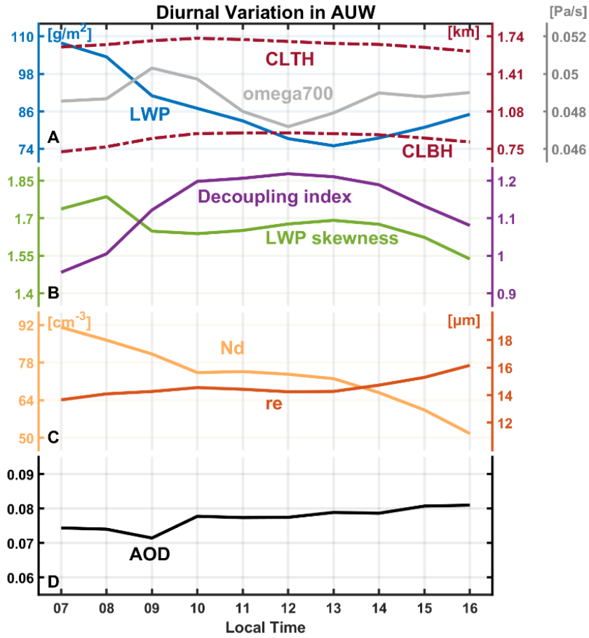
Figure 56. Diurnal patterns in AUW region. (A) Cloud liquid water path (LWP), cloud-top height (CLTH) and cloud bottom height (CLBH) and vertical velocity on 700 hPa ( \omega_{700} , positive values indicate downdraft) from ERA5 reanalysis. (B) LWP skewness and decoupling index in AUW region. (C) Cloud droplet number concentration ( N_d ) and effective radius ( r_e ). (D) Aerosol optical depth (AOD).
