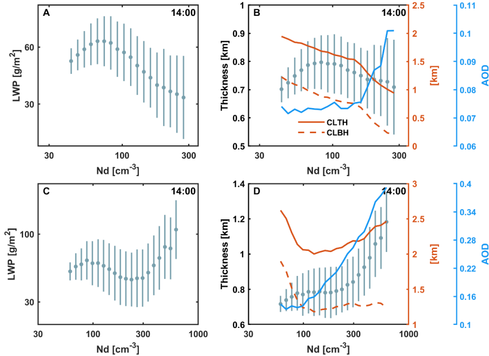
Figure 3. Comparisons between N_d -LWP relationship and N_d -Thickness relationship in two regions. Relationship between N_d and (A) LWP, (B) cloud thickness in AUW region. Relationship between N_d and (C) LWP, (D) cloud thickness in ECS region. The orange solid and dashed lines show the change of cloud top height (CLTH) and cloud bottombase height (CLBH) with N_d .
