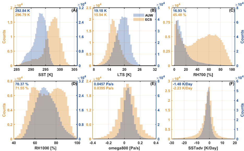
Figure 3. 4-year meteorological conditions of non-precipitation clouds in AUV and ECS regions from 2016 to 2019. Histograms of meteorological factors are presented here. The mean values are labeled in the top-left corner. Data are directly or indirectly derived from ERA5. For vertical velocities on 800 hPa (omega800), positive (negative) values indicate downdraft (updraft).
