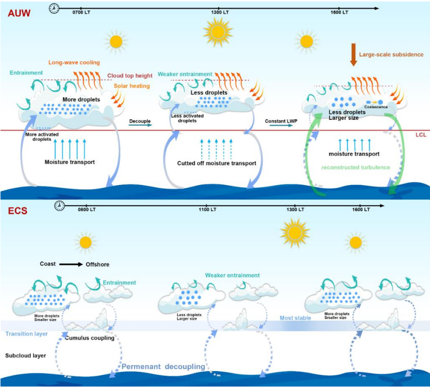
Figure 7 In ECS region, based on the above mechanisms, the diurnal variation of LWP is relatively small, yet N_d exhibits a distinct diurnal pattern. Changes in N_d lead to LWP adjustments that correspond to two microphysical-dynamical processes. The turning point between the two stages exhibits the same diurnal variation as the average N_d (Figure S8). Before noon, a decrease in N_d weakens the warm invigoration (blue line in Figure 1F), while the entrainment feedback intensifies (purple line in Figure 1F). After 1200 LT, the trend reverses. The opposing patterns between warm invigoration and entrainment feedback further reflect their competitive nature. The interaction of these two processes drives the overall diurnal variation in LWP adjustments (black line in Figure 1F).
