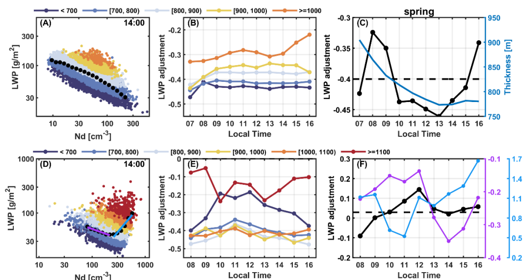
Figure R2. LWP adjustments in log-log spaces and their diurnal patterns in two typical regions (the west of Australia, AUW and the east China sea, ECS) for spring. Same as Figure S9 in the revised Supplementary Materials.
