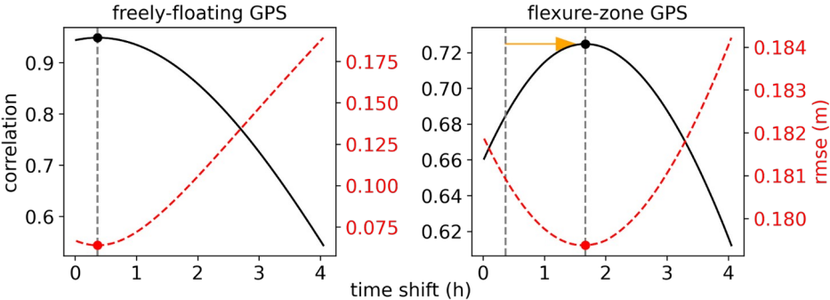
535 Figure 13: Correlations and associated RMSE between GPS measurements and tide model output as a function of a synthetic time shift. The length of the orange arrow corresponds to a 1.3 h time delay that we largely attribute to viscoelastic time delays in the flexural response between the two GPS sites.
