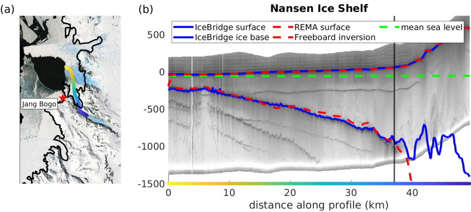
Figure A1: IceBridge radar profile. The cross-section shown in (a) follows the IceBridge flight path and presents (b) the airborne measurements of ice surface and ice base elevations (blue lines). REMA data indicates the ice surface elevation, while the inversion of freeboard is used to determine the ice base depth (dashed red lines). Mean sea level is referenced against the EIGEN-6c4 geoid (dashed green). The approximate location of the grounding line is marked in black.
