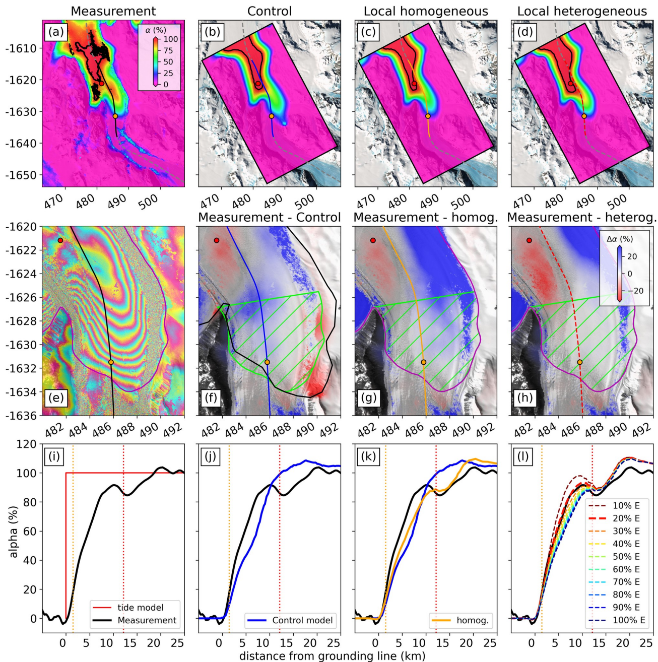
380 Figure 9: Comparison of percentage tidal displacement determined by various \alpha -maps. Panels (a) to (d) show tidal displacement percentages: (a) measured from 31 Sentinel-1 interferograms, (b) from the Control model, (c) from a homogeneous model, and (d) from a heterogeneous model with 20 % effective stiffness in the lateral shear zones. Black contours outline the hydrostatic line, where the ice is in hydrostatic equilibrium, exhibiting full tidal motion ( \alpha=100\% ). The dashed gray line marks the IceBridge flight path, indicating flexure curve locations in panels (i) to (l). Panel (e) shows measured tidal fringes in Priestley Glacier's grounding
