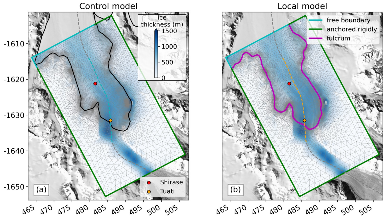
295 Figure 3: Setups for the Control and Local model at Priestley Glacier. (a) The Control model uses the ASAIID grounding line and BedMachine v2 ice thickness. (b) The Local model uses a DInSAR-derived grounding line from TerraSAR-X data and ice thickness from freeboard inversion for floating ice. Colored outlines indicate boundary conditions. The finite-element mesh is in the background. The dashed gray line shows the IceBridge flight path (Nov 300 2013) with radar data for ice-thickness validation (Appendix A). Dashed blue and orange lines represent locations of homogeneous model solutions in Figure 9 j and k, respectively.
