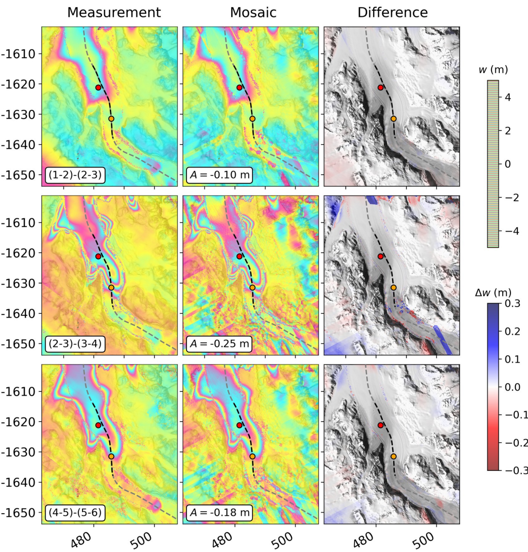
Figure 7: Selection of three measured and mosaicked images from 31 available DInSAR combinations showing double-differential vertical displacement. The SAR image combination is indicated in the lower left corner. The dashed line marks the IceBridge
