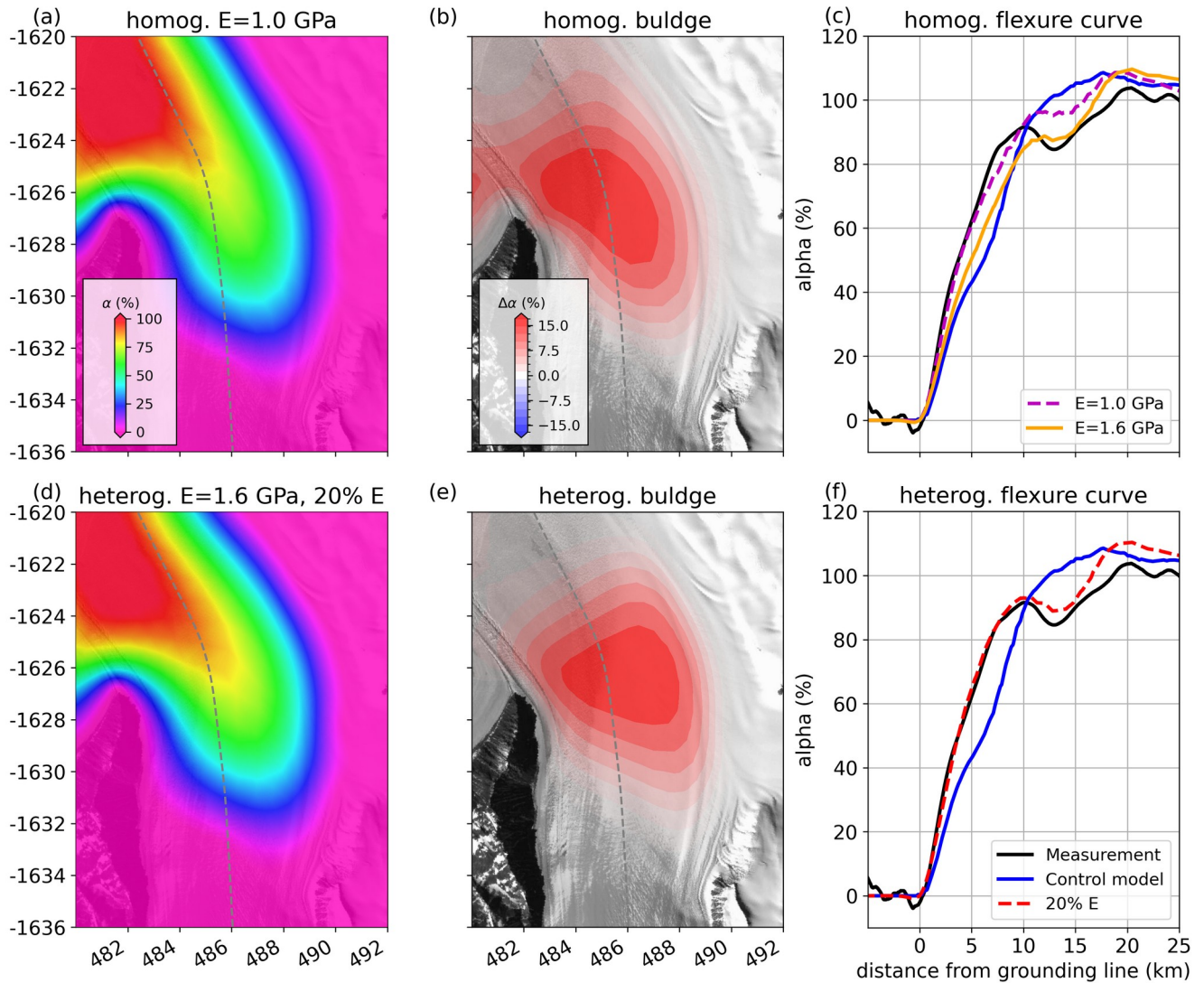
460 Figure 12: Comparison between the best homogeneous and best heterogeneous flexure model solutions. (a) Elastic flexure for a homogeneous Young's modulus of E = 1.0 GPa. (b) Difference relative to the homogeneous reference case of E = 1.6 GPa. (c) Flexure curves for both homogeneous cases compared to the DInSAR measurements and the Control model. (d) Elastic flexure for a heterogeneous ice stiffness model with E = 1.6 GPa and a 20% reduction in the lateral shear zones. (e) Difference between the 465 best heterogeneous case and the homogeneous reference ( E = 1.6 GPa). (f) Best-fit heterogeneous flexure curve compared to satellite observations and the Control model.
