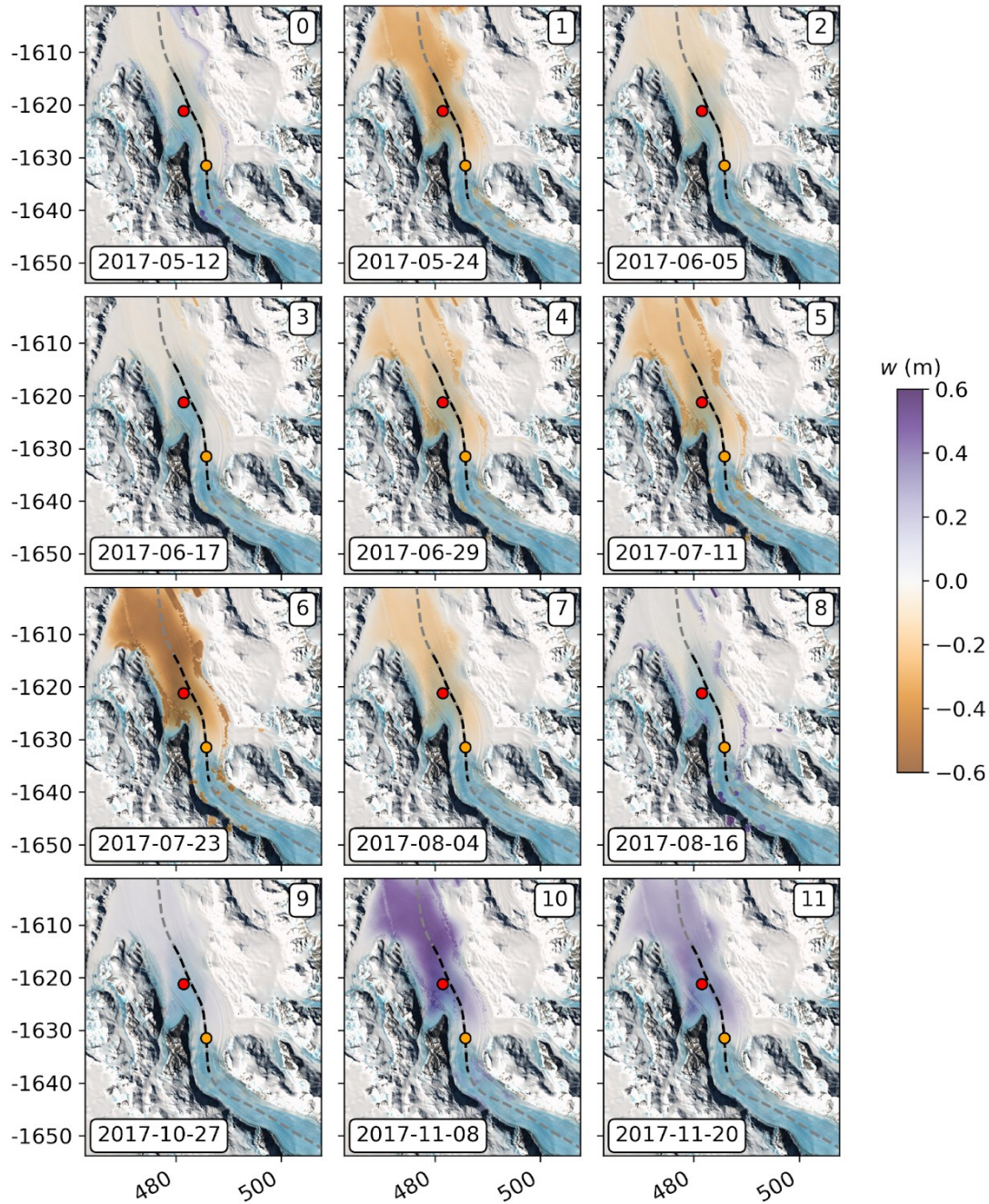
Figure 6. Selection of twelve reconstructed synthesized vertical displacement maps in the tidal flexure zone of Priestley Glacier, showing vertical displacement due to ocean tides during SAR data acquisitions in 2017. The dashed line indicates the IceBridge
