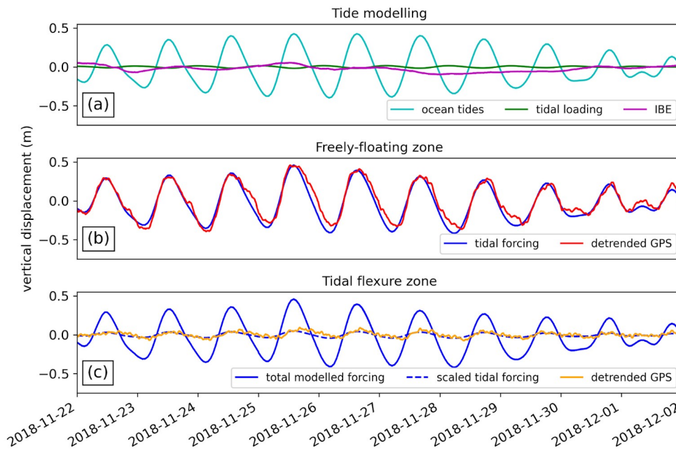
Figure 11: Example of improved tide-model output over one neap-spring-neap tidal cycle, achieved through linear scaling with the tide-deflection ratio from the Control model. (a) The components of the tidal forcing. (b) Tide modeling accurately predicts measured vertical displacement where ice is freely floating, but (c) neglects the damping effect of ice dynamics in the tidal-flexure zone if unscaled. The locations of the two GPS receivers are shown in Figure 9.
