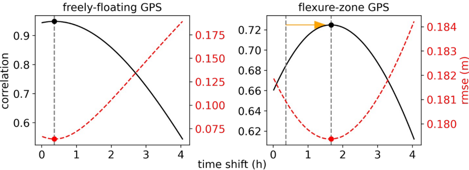
Figure 132: Correlations and associated RMSE between GPS measurements and tide model output as a function of a synthetic time shift. The length of the orange arrow corresponds to a 1.3 h time delay that we largely attribute to viscoelastic time delays in the flexural response between the two GPS sites.
