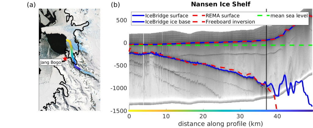
Figure A1: IceBridge radar profile. The cross-section shown in (a) follows the IceBridge flight path and presents (b) the airborne measurements of ice surface and ice base elevations (blue lines). REMA data indicates the ice surface elevation, while the inversion of freeboard is used to determine the ice base depth (dashed red lines). Mean sea level is referenced against the EIGEN-6c4 geoid (dashed green). The approximate location of the grounding line is marked in black.
