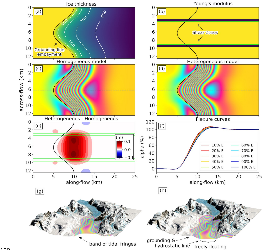
130 Figure 1: Hypothesis: (a) Idealized ice thickness for synthetic model experiments. (b) The Young's modulus field, where values are varied in the shear-zone areas (shown in blue) in steps of 10 % from 10 % to 100 % of the Young's modulus used for the remaining ice-covered areas (indicated in yellow), which is set at 1.6 GPa. (c) Modeled tidal flexure under 1m tidal forcing for a homogeneous case, and (d) a heterogeneous case. (e) Their difference, showing a bulge up to 10 % of the applied tidal forcing. (f) Cross-section along the centerline (dashed lines in panels c and d), illustrating the flexure curves where Young's modulus is reduced in lateral shear zones. Panels (g) and (h) depict vertical tidal flexure during high and low tide scenarios. Each color fringe represents approximately 10 cm of vertical displacement, corresponding to a tidal amplitude of \pm 60 cm in this schematic. The concentrated band of tidal fringes marks the grounding line at its landward edge and the hydrostatic line at its seaward boundary. Beyond this, the ice floats freely on the ocean, oscillating harmonically with the tides. Note that vertical displacement is not to scale in this schematic. 135 140
