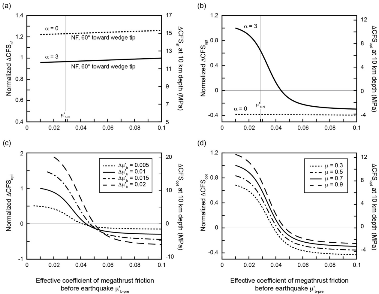
Figure 4: Coulomb failure stress change as function of effective coefficient of megathrust friction before the earthquake, \mu'_{b\text{-pre}} , and for a change in megathrust friction of \Delta\mu'_b = 0.01 . Solid lines indicate solutions for the reference wedge model discussed in the text. Dashed and dotted lines indicate solutions for adjusted model parameters. (a) Coulomb failure stress change on a normal fault (NF) dipping at 60^\circ toward the wedge tip. (b) Difference in Coulomb failure stress on optimal failure planes before and after the earthquake, \Delta\text{CFS}_{\text{opt}} . (c, d) Dependence of \Delta\text{CFS}_{\text{opt}} on \Delta\mu'_b and coefficient of friction \mu . Left ordinates show \Delta\text{CFS} values normalized to the maximum \Delta\text{CFS} value obtained for reference wedge model. Right ordinate indicates \Delta\text{CFS} values at 10 km depth. All \Delta\text{CFS} values in (a-c) are calculated for \mu = 0.7 .
