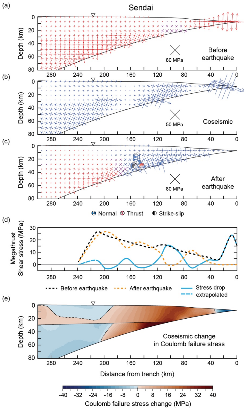
Figure 7: Preferred model of forearc stress change due to the Tohoku-Oki earthquake along the Sendai cross section. See Fig. 5a for the location of the cross section. Red and blue stress crosses in (a-c) indicate that the plunge of \sigma_1 is less than 40° (deviatoric compression) and more than 50° (deviatoric tension), respectively; purple crosses indicate a plunge of \sigma_1 between 40° and 50°. The size of the stress crosses scale with the differential stress. (a) Deviatoric stress before the earthquake. (b) Incremental change in deviatoric stress caused by the earthquake. (c) Deviatoric stress after the earthquake. Beach balls indicate focal mechanism solutions of aftershocks (cf. Fig. 5). (d) Modelled megathrust shear stress before (black) and after (orange) the earthquake, and megathrust stress drop (blue). (e) Coseismic change in Coulomb failure stress calculated for \mu = 0.7 .
