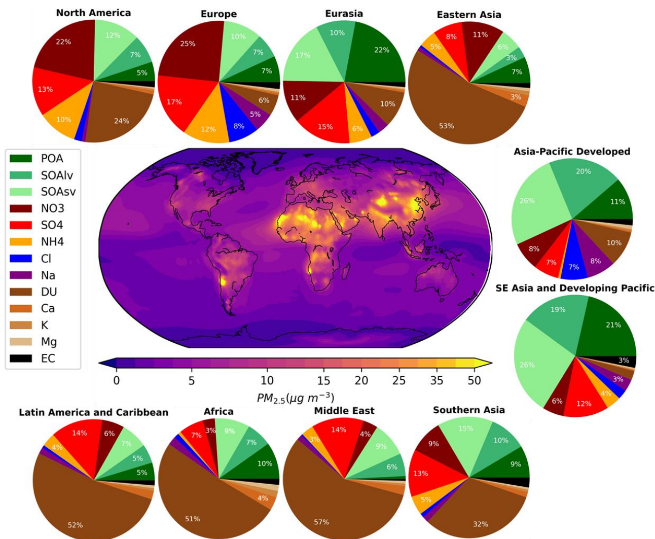
Figure 8: Pie charts showing the simulated 20-year average chemical composition of PM_{2.5} in the 10 regions considered according to WGIIR AR6. The central world map shows the simulated average near-surface concentration of PM_{2.5} (in \mu g m^{-3} ) during the period 2000-2020.
