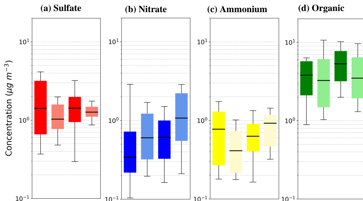
Figure 15: Decadal \text{PM}_1 concentration trends in North America expressed by the bar plots of the mass concentration (in \mu\text{g m}^{-3} ) for (a) sulfate, (b) nitrate, (c) ammonium, and (d) OA during the periods 2000 - 2010 (left) and 2011 - 2020 (right) as calculated from the AMS observational dataset (dark colors) and the corresponding simulation values (light colors). The upper and lower whiskers range from 10-90%, the quartiles from 25-75% of the dataset. The black line is the median.
