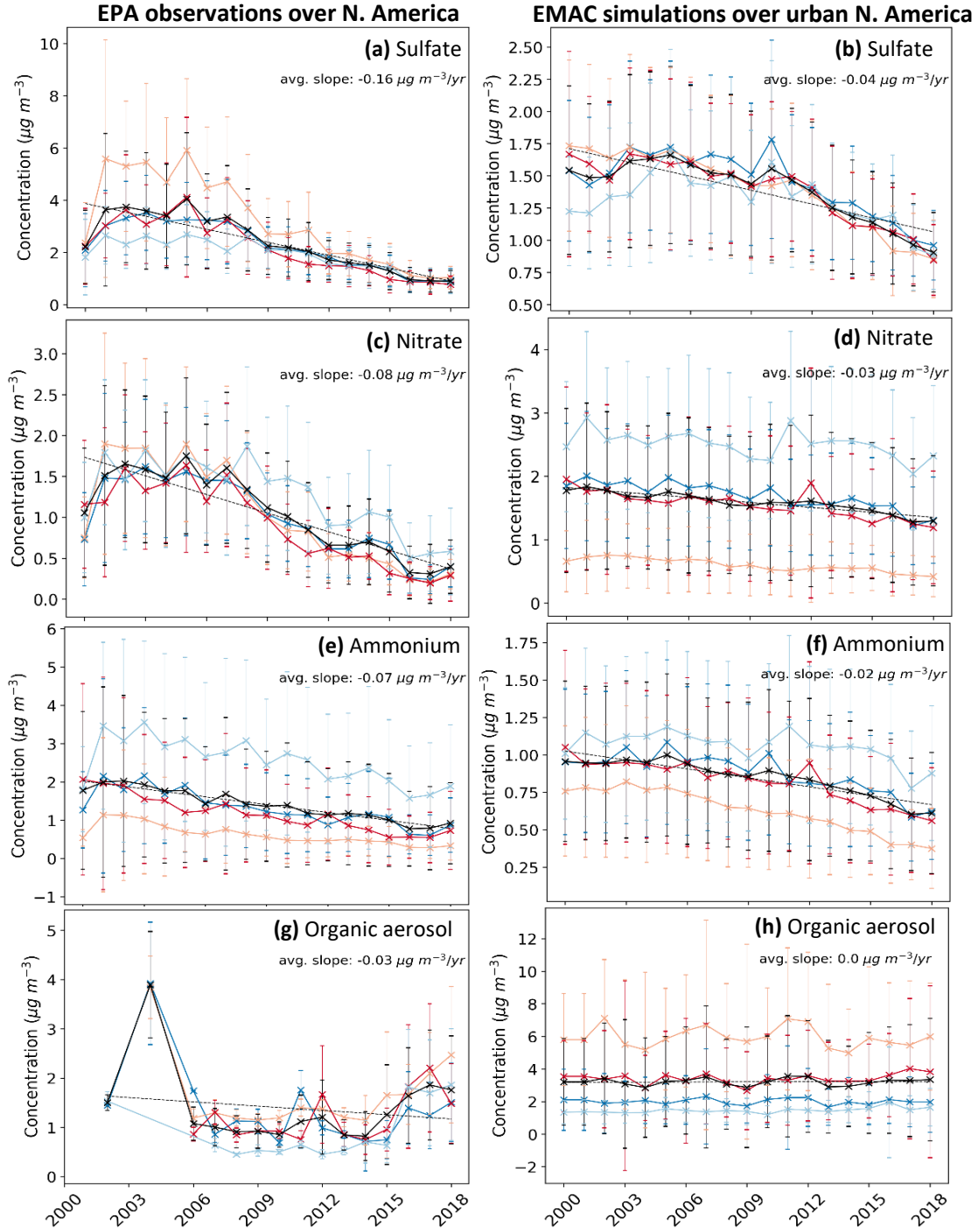
Figure 13: Temporal evolution of the filter-based observed (a, c, e, and g subplots on the left) and simulated (b, d, f, h subplots on the right) concentrations of \text{PM}_{2.5} sulfate (a, b), nitrate (c, d), ammonium, (e, f), and organic aerosol (g, h) during the period 2000–2018 over urban locations in North America. Black lines show the annual trend while the dark blue, light blue, orange, and red lines represent the seasonal trends during winter, spring, summer, and autumn. Ranges represent the 1\sigma SD (standard deviation).
