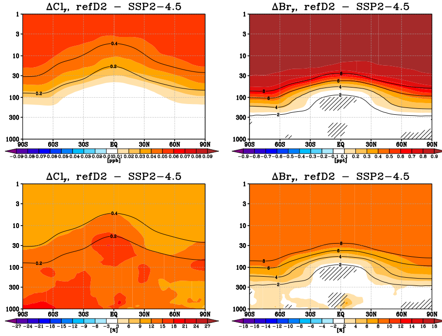
Figure A1. Zonal-mean absolute (top) and relative (bottom) changes in total Chlorine ( \text{Cl}_y ), left, and total bromine ( \text{Br}_y ) (right) between refD2 and SSP2-4.5 scenarios for 2080–2099 conditions.
