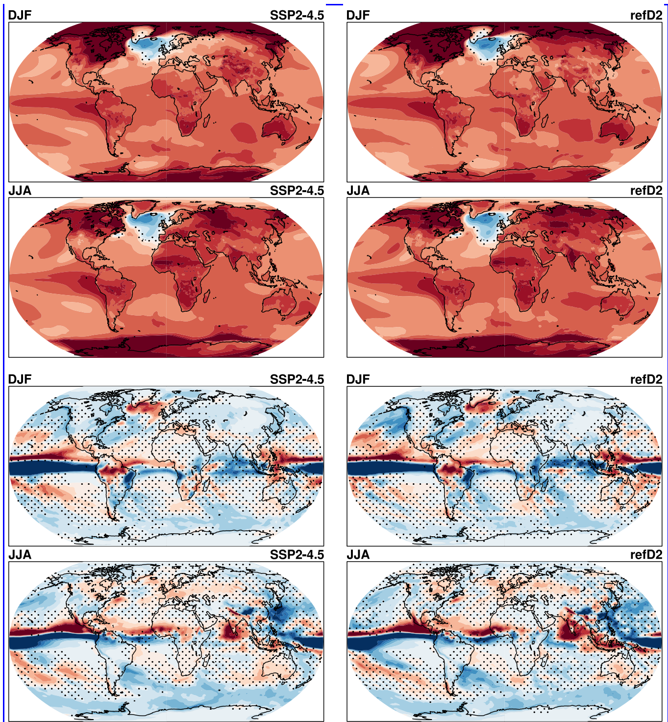
Figure A4. Ensemble-mean differences between 2080 – 2099 future experiments and 2020 – 2030 control experiments for near surface temperature in December/January/February (first row) and June/July/August (second row) and for precipitation in December/January/February (third row) and June/July/August (fourth row) for SSP2-4.5 (left) and refD2 (right). Areas of non-significant difference at the 95 th % level to the control are marked as small black dots.
