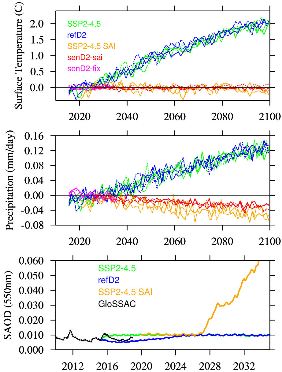
Figure 1. Changes in global mean air surface temperatures (top), precipitation (middle) compared to 2020 – 2030 average conditions, and for available ensemble members (different line styles) for the different experiments performed with CESM2(WACCM6) (different colors). Bottom panel: stratospheric aerosol optical depth averaged between 80°N and 80°S (consistent with for GloSSAC observations (bottom panel black) compared to 2020 – 2030 average conditions, and the ensemble mean for different experiments performed with CESM2(WACCM6) (colored lines).
