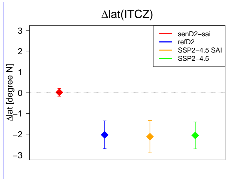
Figure A5. Differences of the annual mean and latitude of the Intertropical Convergence Zone (ITCZ) between 2080 – 2099 compared to 2010 – 2030 for different experiments (see legend), the standard error is shown as vertical bars.
