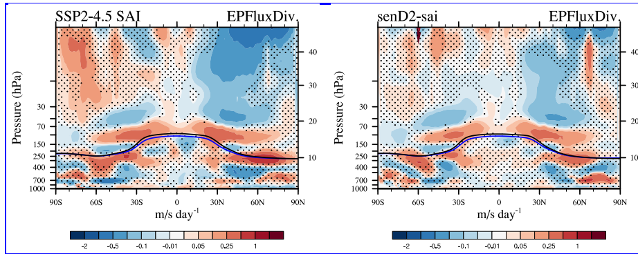
Figure A2. Differences of the annual-mean zonally and latitude-of-the-Intertropical-Convergence-Zone-annually averaged Eliassen-Palm Flux divergence between SSP2-4.5 SAI in 2080–2099 and SSP2-4.5 in 2015–2035 (left) and senD2-sai in 2080–2099 compared to 2010 and senD2-fix in 2015–2030 for different experiments (right). Areas of non-significant difference at the 95 th % level to the control are marked as vertical bars small black dots.
