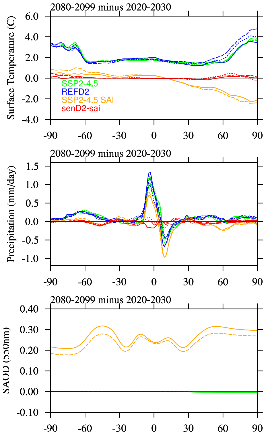
Figure 8. Zonal mean differences between 2080 – 2099 future experiments and 2020 – 2030 control experiments for the available ensemble members ( different line styles ) (see table-Table 1 ), for near surface temperature (top), precipitation (middle), and Stratospheric Aerosol Optical Depth (SAOD) (bottom).
