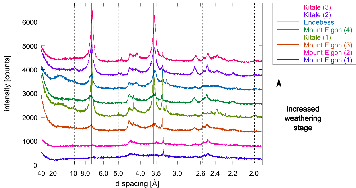
Figure C1: Comparison of the oriented clay fractions in air-dried, Ca-saturated soils from Kenya. Full lines indicate peak positions of kaolinite at 7.17 Å and 3.58 Å, and dotted lines indicate peak positions of illitic mineral phases at 10 Å, 5.0 Å, 3.36 Å, 2.56 Å, and 2.00 Å.
