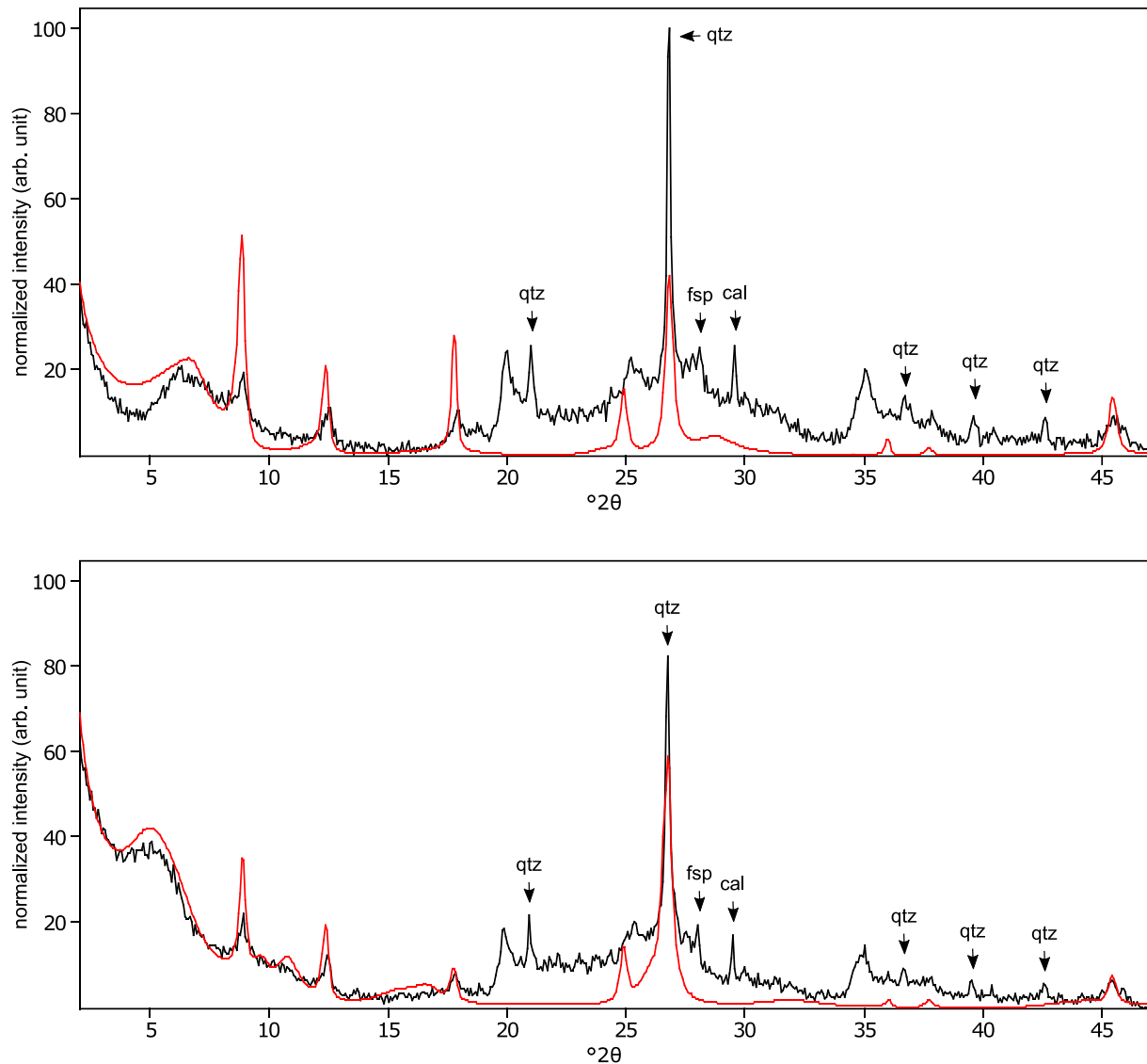
Figure C13: The oriented clay fraction of soil from Changchun (China). Top: experimental XRD patterns in air-dried, Ca-saturated state (black) and the modeled pattern (red) of 9% kaolinite, 11% randomly interstratified kaolinite-smectite (regular) (50:50), 11% randomly interstratified illite-smectite (high charge) (33:33:34), 60% randomly interstratified illite-smectite (97:3), and 9% randomly interstratified illite-smectite (63:37); Bottom: experimental XRD patterns in ethylene glycol solvated, Ca-saturated state (black) and the modeled pattern (red) of 6% kaolinite, 24% randomly interstratified kaolinite-smectite (regular) (50:50), 17% randomly interstratified illite-smectite (high charge) (33:33:34), 22% randomly interstratified illite-smectite (97:3), and 31% randomly interstratified illite-smectite (63:37). The arrows indicate quartz (qtz), feldspar peak (fsp), and calcite (cal) peaks.
