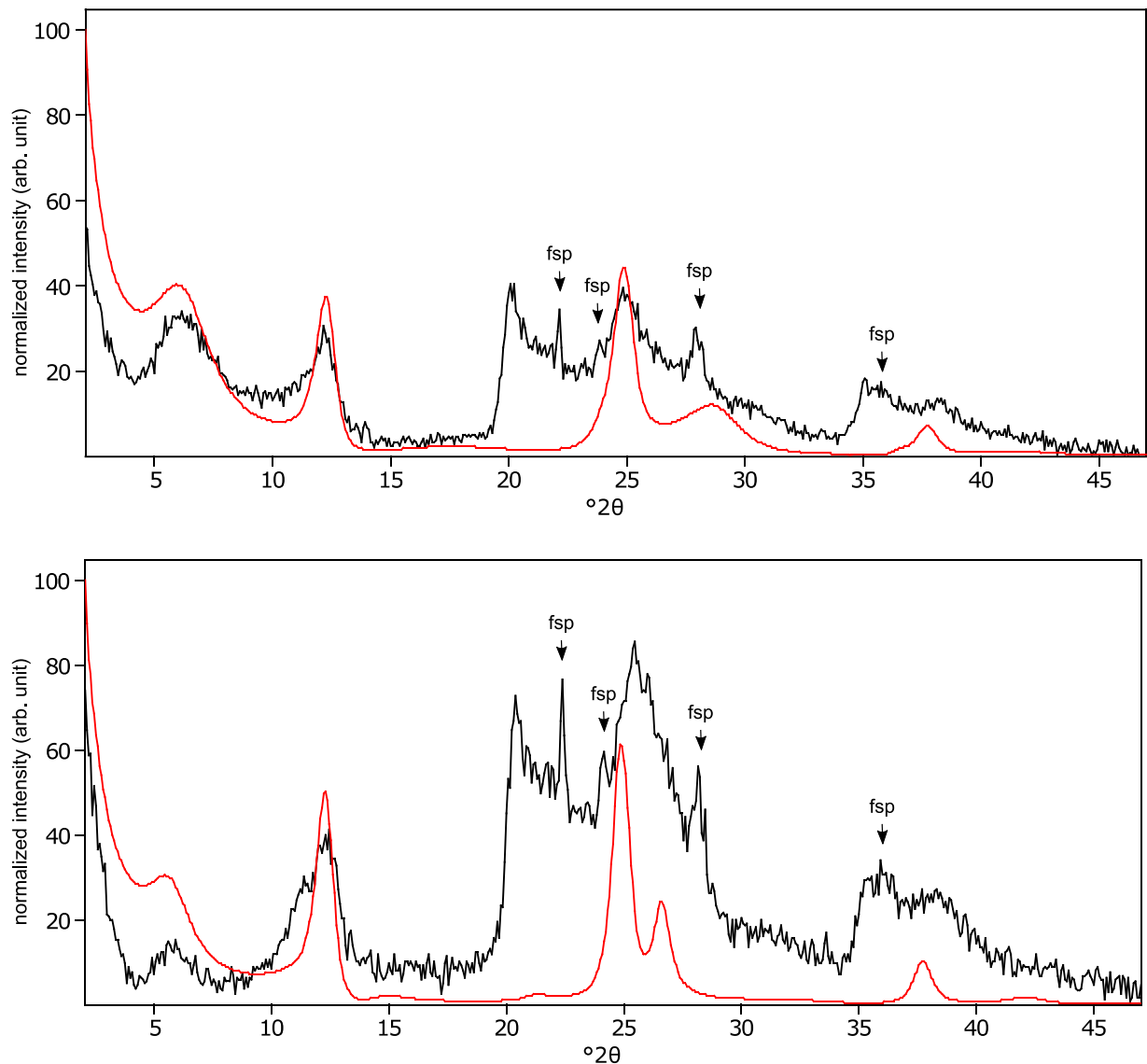
Figure C5: The oriented clay fraction of soil from Pagsanjan (Philippines 1). Top: experimental XRD patterns in air-dried, Ca-saturated state (black) and the modeled pattern (red) of 30% kaolinite and 70% randomly interstratified kaolinite-smectite (high charge) (50:30:20); Bottom: experimental XRD patterns in ethylene glycol solvated, Ca-saturated state (black) and the modeled pattern (red) of 30% kaolinite, and 70% randomly interstratified kaolinite-smectite (high charge) (50:30:20). The arrows indicate feldspar (fsp) peaks.
