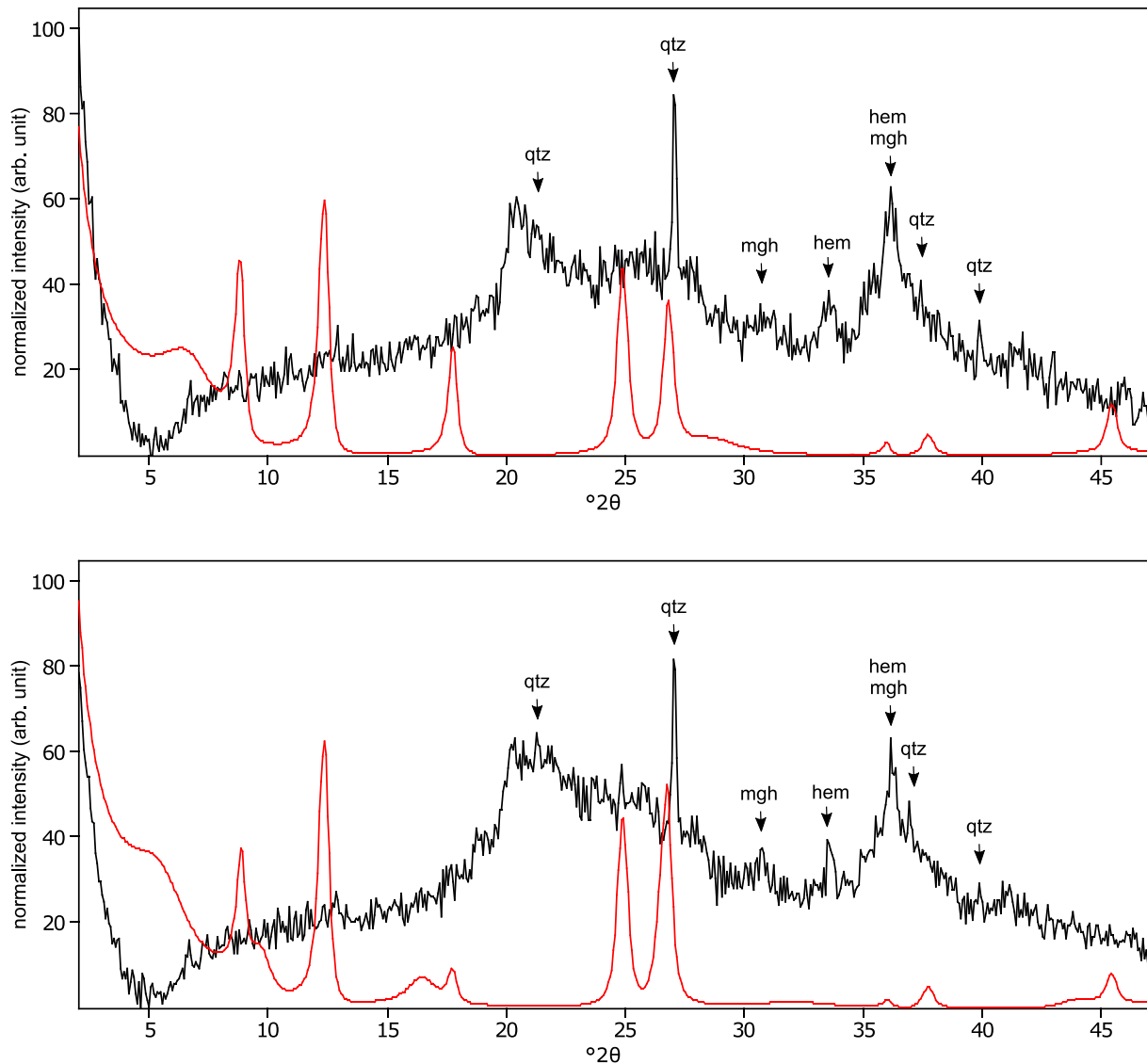
450 Figure C4: The oriented clay fraction of soil from Mount Elgon (Kenya 1). Top: experimental XRD patterns in air-dried, Ca- saturated state (black) and the modeled pattern (red) of 30% kaolinite, 45% randomly interstratified illite-smectite (97:3), and 25% randomly interstratified illite-smectite (60:40); Bottom: experimental XRD patterns in ethylene glycol solvated, Ca-saturated state (black) and the modeled pattern (red) of 27% kaolinite, 24% randomly interstratified illite-smectite (97:3), and 49% randomly 455 interstratified illite-smectite (60:40). The arrows indicate quartz (qtz), maghemite (mgh), and hematite (hem) peaks. Allophane shows broad peaks at 3.52 Å (25.29 °2θ) and 2.50 Å (35.85 °2θ).
