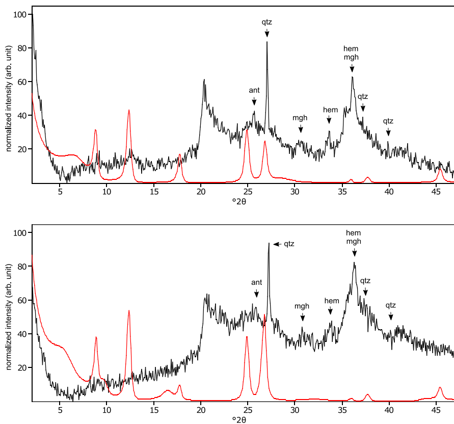
475 Figure C7: The oriented clay fraction of soil from Mount Elgon (Kenya 2). Top: experimental XRD patterns in air-dried, Ca-saturated state (black) and the modeled pattern (red) of 31% kaolinite, 45% randomly interstratified illite-smectite (97:3), and 24% randomly interstratified illite-smectite (60:40); Bottom: experimental XRD patterns in ethylene glycol solvated, Ca-saturated state (black) and the modeled pattern (red) of 26% kaolinite, 28% randomly interstratified illite-smectite (97:3), and 46% randomly interstratified illite-smectite (60:40). The arrows indicate quartz (qtz), anatase (ant), maghemite (mgh), and hematite (hem) peaks.
