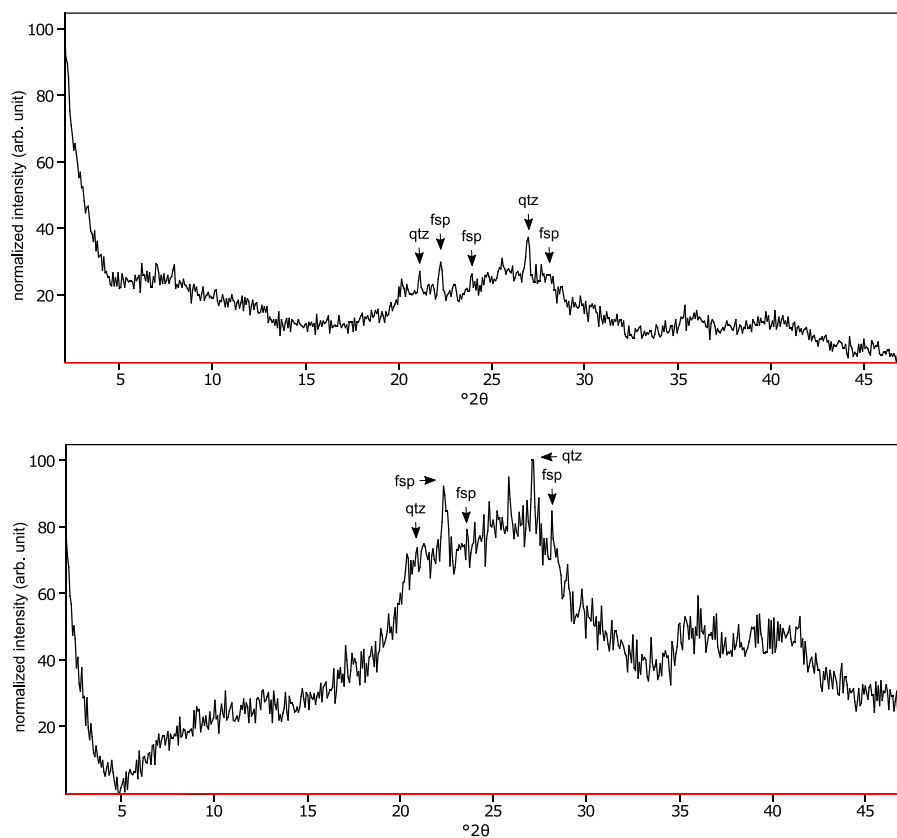
450 Figure C3: The oriented clay fraction of soil from Miyakonojo (Japan). Top: experimental XRD patterns in air-dried, Ca-saturated state (black), and no pattern was modeled because no phyllosilicate could be identified; Bottom: experimental XRD patterns in ethylene glycol solvated, Ca-saturated state (black) and no pattern was modeled because no phyllosilicate could be identified. The arrows indicate quartz (qtz) and feldspar (fsp) peaks. Allophane shows broad peaks at 3.50 Å (25.45 °2θ) and 2.50 Å (35.90 °2θ).
