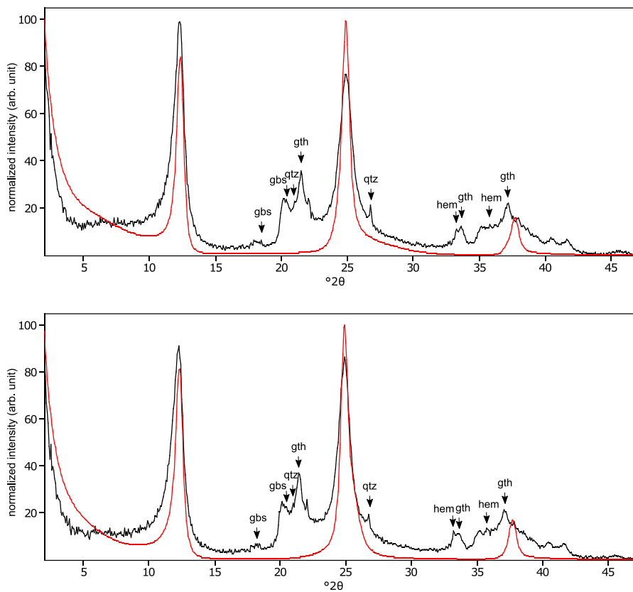
Figure C26: The oriented clay fraction of soil from Cavinti (Philippines). Top: experimental XRD patterns in air-dried, Ca-saturated state (black) and the modeled pattern (red) of 38% kaolinite, and 62% randomly interstratified kaolinite-smectite (high charge) (80:10:10); Bottom: experimental XRD patterns in ethylene glycol solvated, Ca-saturated state (black) and the modeled pattern (red) of 42% kaolinite, and 58% randomly interstratified kaolinite-smectite (high charge) (80:10:10). The arrows indicate quartz (qtz), gibbsite (gbs), goethite (gth), and hematite (hem) peaks.
