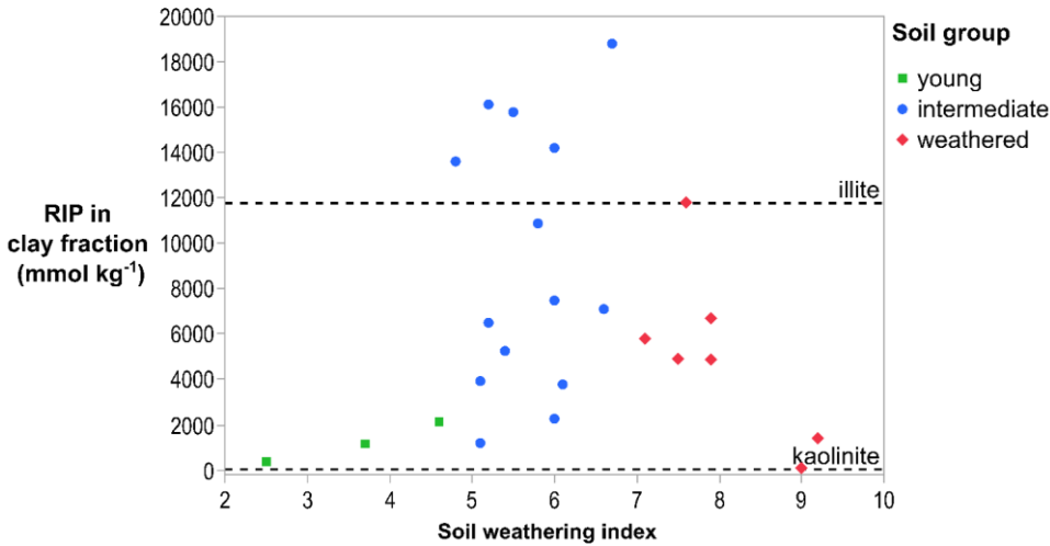
Figure 2: RIPs in the clay fractions of soils as a function of soil weathering. The dashed lines are RIP of illite ( 11,800 \text{ mmol kg}^{-1} in < 2 \mu\text{m} fraction; Nakao et al., 2008) and kaolinite ( 6 \text{ mmol kg}^{-1} in < 2 \mu\text{m} fraction; Nakao et al., 2008). The data suggest an upward trend between young and intermediate weathering followed by a decrease in highly weathered soils.
