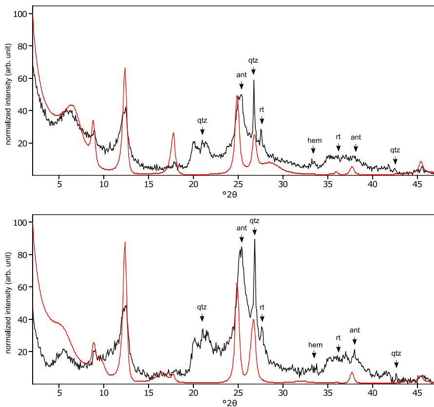
Figure C20: The oriented clay fraction of soil from Endebess (Kenya). Top: experimental XRD patterns in air-dried, Ca-saturated state (black) and the modeled pattern (red) of 29% kaolinite, 25% randomly interstratified illite-smectite (97:3), and 46% randomly interstratified illite-smectite (60:40); Bottom: experimental XRD patterns in ethylene glycol solvated, Ca-saturated state (black) and the modeled pattern (red) of 38% kaolinite, 13% randomly interstratified illite-smectite (97:3), and 49% randomly interstratified illite-smectite (60:40). The arrows indicate quartz (qtz), anatase (ant), rutile (rt), and hematite (hem) peaks.
