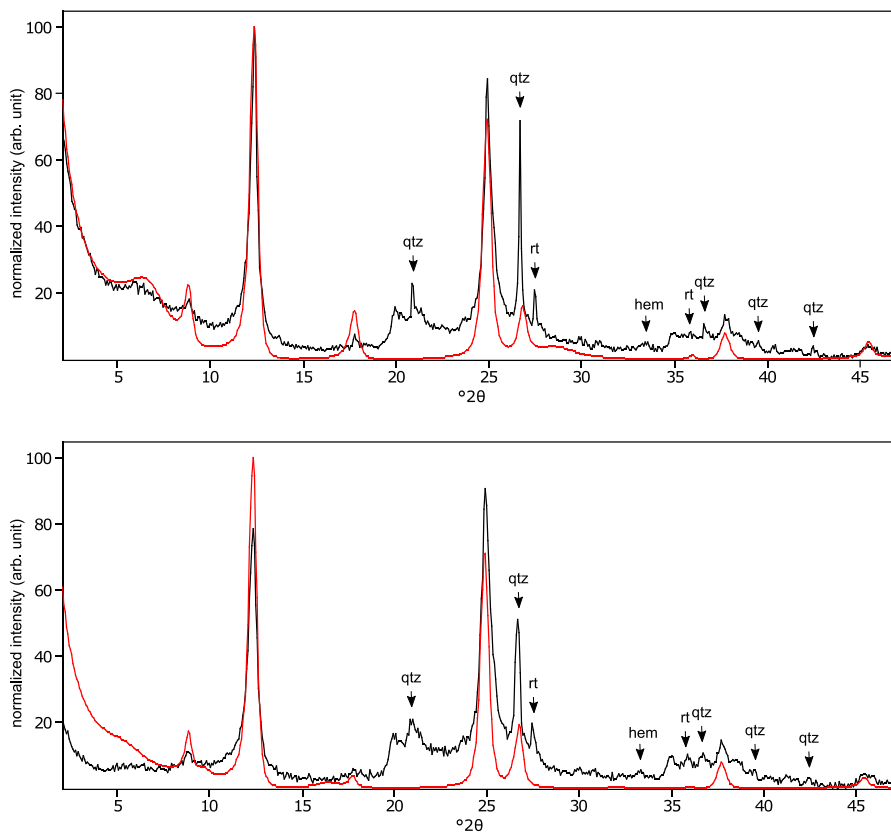
Figure C17: The oriented clay fraction of soil from Kitale (Kenya 1). Top: experimental XRD patterns in air-dried, Ca-saturated state (black) and the modeled pattern (red) of 53% kaolinite, 19% randomly interstratified illite-smectite (97:3), and 28% randomly interstratified illite-smectite (60:40); Bottom: experimental XRD patterns in ethylene glycol solvated, Ca-saturated state (black) and the modeled pattern (red) of 65% kaolinite, 16% randomly interstratified illite-smectite (97:3), and 19% randomly interstratified illite-smectite (60:40). The arrows indicate quartz (qtz), rutile (rt), and hematite (hem) peaks.
