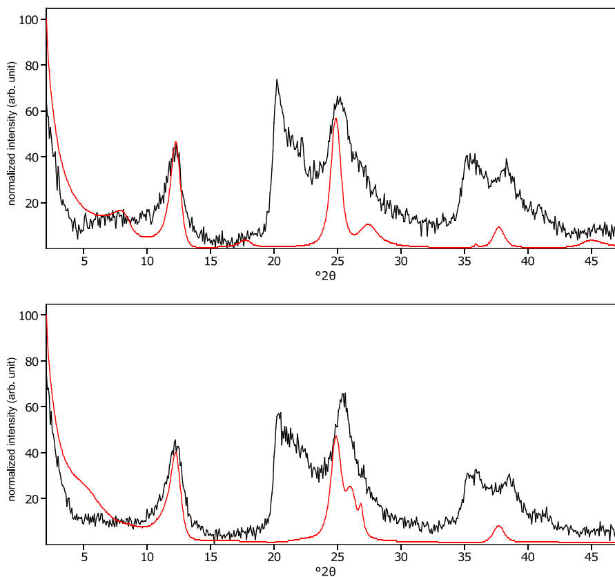
570 Figure C22: The oriented clay fraction of soil from Pagsanjan (Philippines 5). Top: experimental XRD patterns in air-dried, Ca-saturated state (black) and the modeled pattern (red) of 66% kaolinite, 2% randomly interstratified kaolinite-smectite (high charge) (60:24:16), and 32% randomly interstratified illite-smectite (high charge) (70:15:15); Bottom: experimental XRD patterns in ethylene glycol solvated, Ca-saturated state (black) and the modeled pattern (red) of 36% kaolinite, 58% randomly interstratified kaolinite-smectite (high charge) (60:24:16) and 6% randomly interstratified illite-smectite (high charge) (70:15:15).
