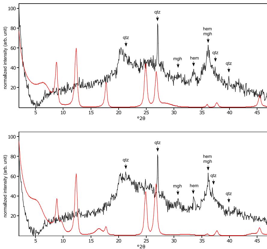
455 Figure C4: The oriented clay fraction of soil from Mount Elgon (Kenya 1). Top: experimental XRD patterns in air-dried, Ca- saturated state (black) and the modeled pattern (red) of 30% kaolinite, 45% randomly interstratified illite-smectite (97:3), and 25% randomly interstratified illite-smectite (60:40); Bottom: experimental XRD patterns in ethylene glycol solvated, Ca-saturated state (black) and the modeled pattern (red) of 27% kaolinite, 24% randomly interstratified illite-smectite (97:3), and 49% randomly 460 interstratified illite-smectite (60:40). The arrows indicate quartz (qtz), maghemite (mgh), and hematite (hem) peaks. Allophane shows broad peaks at 3.52 Å (25.29 °2θ) and 2.50 Å (35.85 °2θ).
