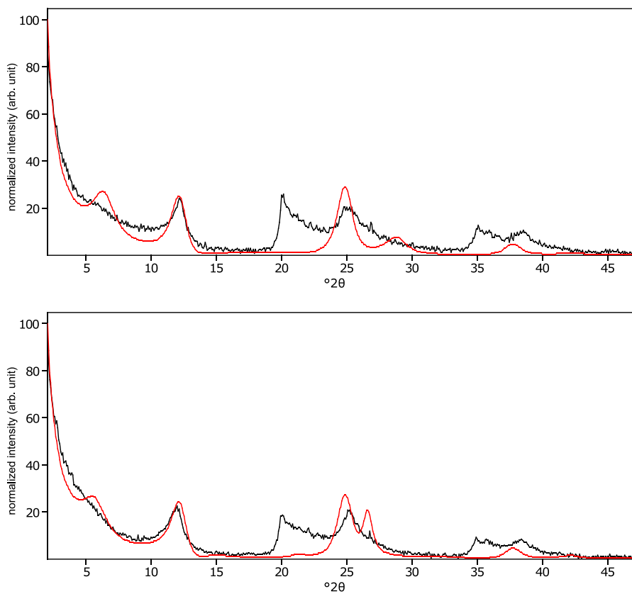
565 Figure C21: The oriented clay fraction of soil from Pagsanjan (Philippines 4). Top: experimental XRD patterns in air-dried, Ca-saturated state (black) and the modeled pattern (red) of 52% kaolinite and 48% randomly interstratified kaolinite-smectite (high charge) (33:33:34); Bottom: experimental XRD patterns in ethylene glycol solvated, Ca-saturated state (black) and the modeled pattern (red) of 41% kaolinite, and 59% randomly interstratified kaolinite-smectite (high charge) (33:33:34).
