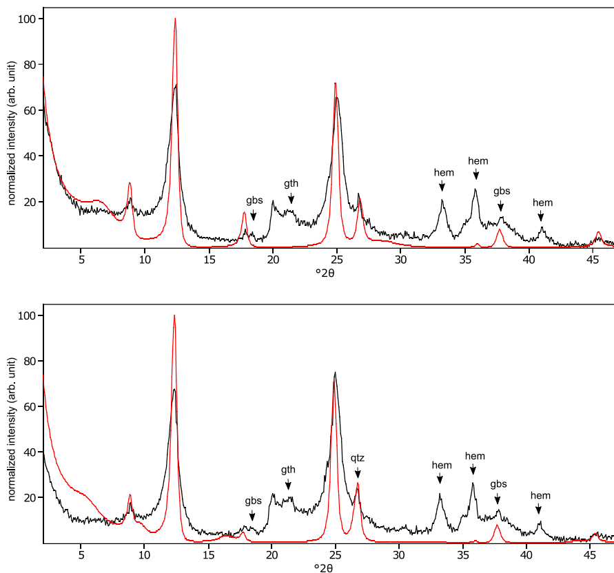
Figure C23: The oriented clay fraction of soil from Kitale (Kenya 2). Top: experimental XRD patterns in air-dried, Ca-saturated state (black) and the modeled pattern (red) of 53% kaolinite, 27% randomly interstratified illite-smectite (97:3), and 20% randomly interstratified illite-smectite (60:40); Bottom: experimental XRD patterns in ethylene glycol solvated, Ca-saturated state (black) and the modeled pattern (red) of 55% kaolinite, 16% randomly interstratified illite-smectite (97:3), and 29% randomly interstratified illite-smectite (60:40). The arrows indicate gibbsite (gbs), goethite (gth), and hematite (hem) peaks.
