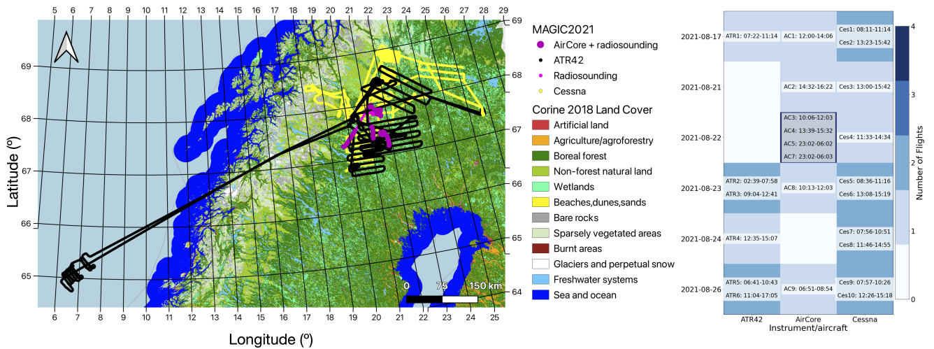
Figure 1. Location (left) and date and time (right) of MAGIC2021 measurements used in this study. Map background shows land use adapted from the Corine2018 dataset (European Environment Agency, 2019). Individual land cover types from the Corine2018 dataset are grouped in broader categories to ease map interpretation. Notably, wetlands include inland marshes, peat bogs, salt marshes, salines, intertidal flats, coastal lagoons and estuaries, i.e. both freshwater and saltwater wetlands.
