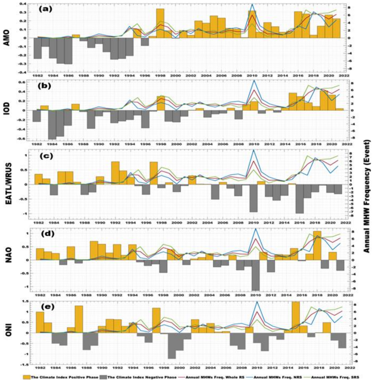
865 Figure 11. Annual time series of normalized climate indices and marine heatwave frequency in the Red Sea. (a) AMO index, (b) IOD index, (c) EATL/WRUS pattern, (d) NAO index, and (e) ONI index are shown with annual MHW frequency in the entire Red Sea (red line), northern Red Sea (blue line), and southern Red Sea (green line). Yellow and gray bars indicate the positive and negative phases of the climate indices, respectively.
