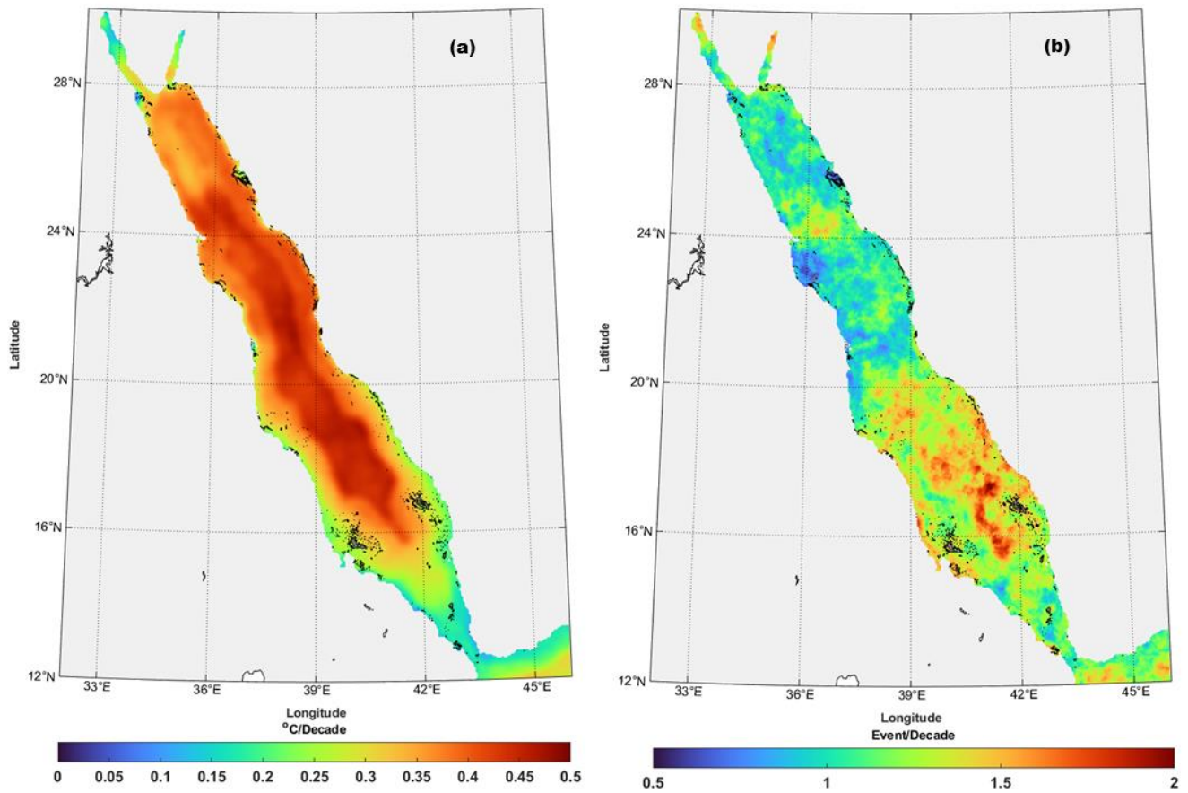
755 Figure 4. Trends in (a) sea surface temperature ( ^{\circ}\text{C}/\text{decade} ) and (b) marine heatwave frequency (events/decade) in the Red Sea from 1982 to 2021.
