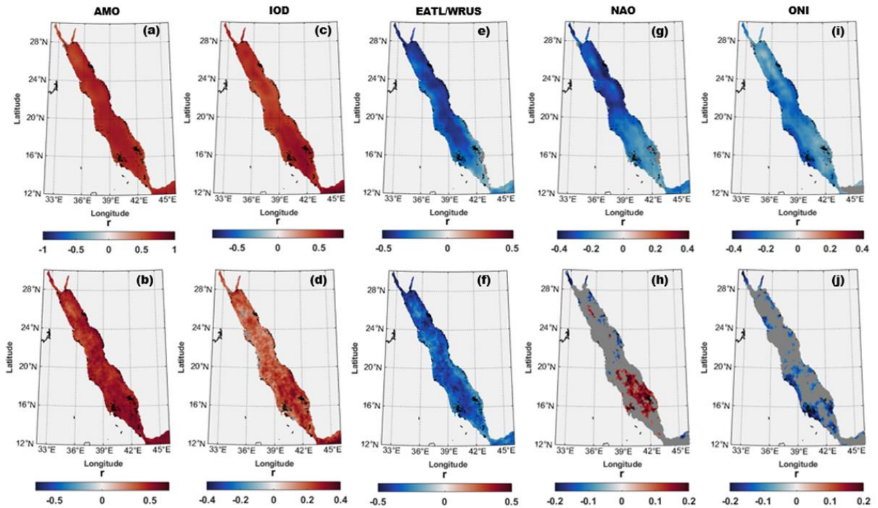
850 Figure 10. Correlation maps of the SST anomaly (upper panels) and marine heatwave frequency (lower panels) in the Red Sea with different climate modes from 1982 to 2020. Correlations are shown with the AMO index (a, b), IOD pattern (c, d), EATL/WRUS index (e, f), NAO index (g, h), and ONI index (i, j). Gray shading indicates areas where the correlation is not significant ( p -value > 0.05 ).
