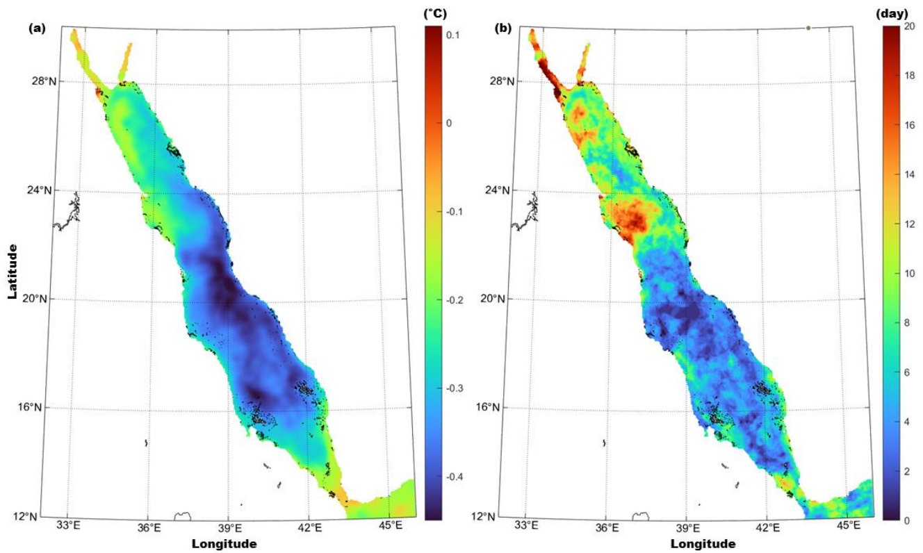
780 Figure 6. Spatial distribution of the average (a) sea surface temperature anomaly ( ^{\circ}\text{C} ) and (b) marine heatwave days (days) in 785 the Red Sea during the coldest years of the study period (1982-2021).
