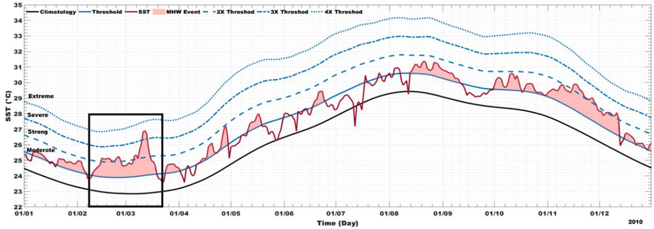
870 Figure 12. Marine heatwave events in the northern Red Sea in 2010. The red shaded area indicates the duration of the event. The solid red line represents the sea surface temperature, the solid black line represents the climatology, the solid blue line represents the threshold, and the dotted blue lines represent the multiples of the threshold (defining the MHW categories).
