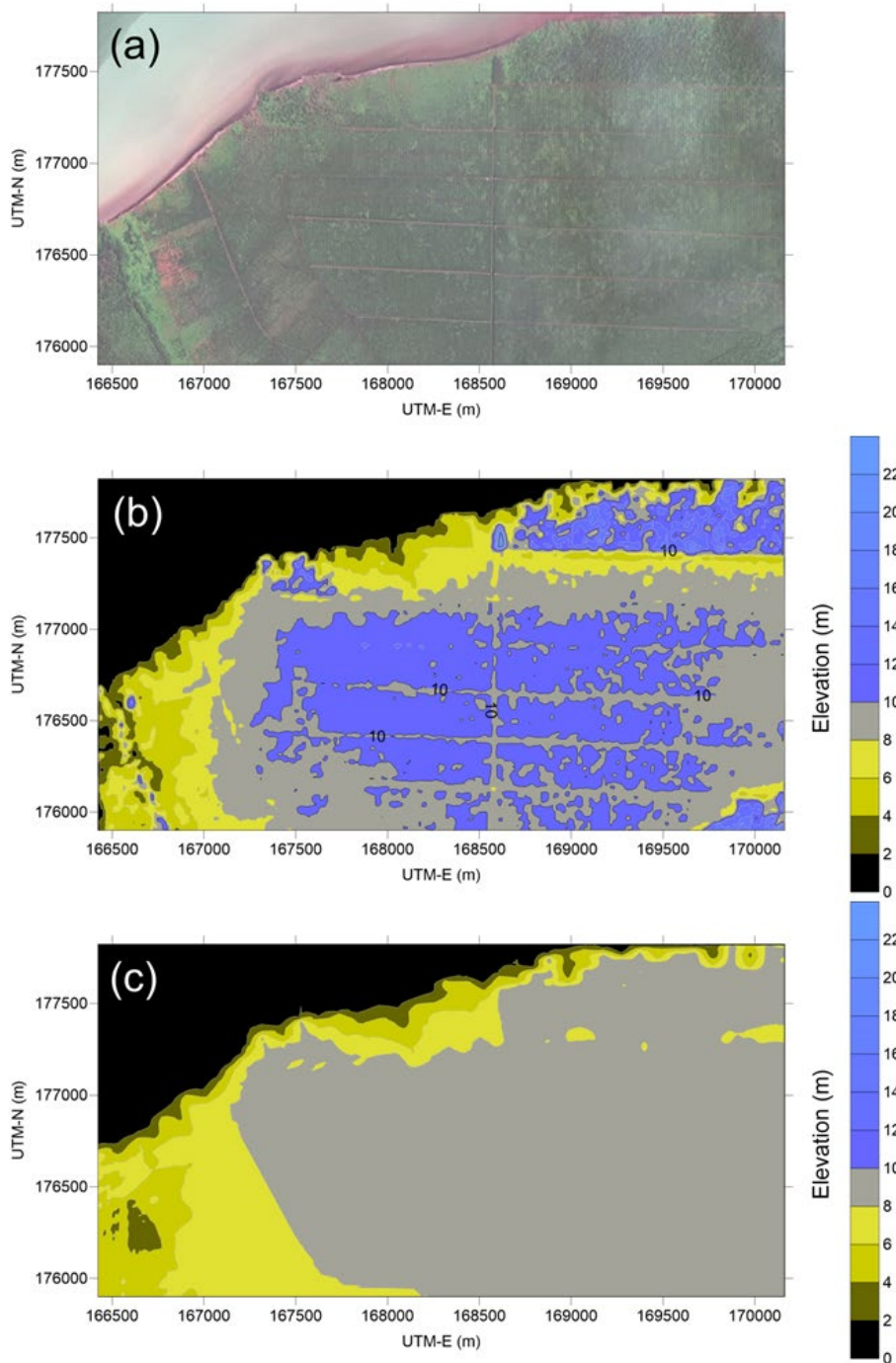
Figure F2: Comparison of (a) SPOT-6 data with (b) original DEMNAS data with (c) DTM removed from vegetation. The elevation of the bare land above 0 m was used to interpolate and generate a DTM with an 8 m resolution by kriging.
