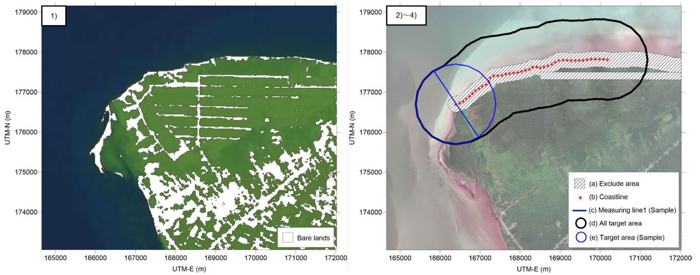
Figure F1: Methodology of removal of vegetation from DEMNAS data. 1) A Landsat5 image (2 February 2010) was used to classify bare land and other land covers using machine learning. 2) The bare land raster was set at 1 and multiplied by the DEMNAS data to produce the bare land elevation data. The elevation anomalies at the boundary between the peat swamp forest and the bare road and a radius of 200 m from the coastline (a) were masked. 3) A measuring line was made in the offshore direction from inland at points where the coastline was divided at 100 m intervals (b) (c). 4) The median elevation of the bare lands found 1 km (d) (e) from the coastline was assigned to the coastline and linearly complemented.
