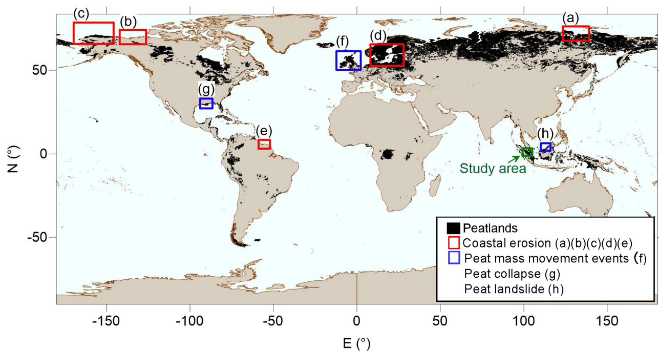
780 Figure A1: Global distribution of the lateral degradation in peatlands (Based on data from the Global Peatland Database / Greifswald Mire Centre (2024)).
