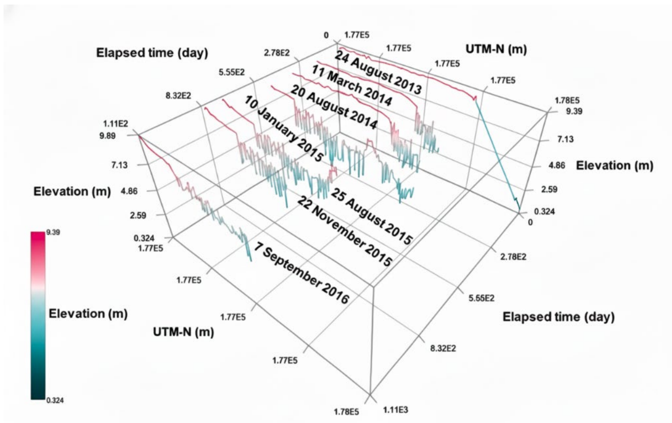
460 Figure 7: The change in temporal elevation in Section A-A'. The elevation decreased due to PMM since 24 August 2013.
