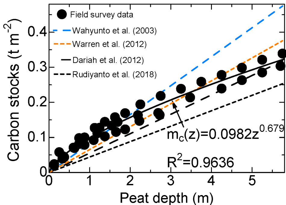
Figure 17: Carbon stocks relative to depth. Literature values sourced from Wahyunto et al., 2003; Dariah et al., 2012; Warren et al., 2012 and Rudiyanto et al., 2018. The literature values from Wahyunto et al., 2003 were calculated using average values for the bulk density and carbon content of Hemic peat. Literature values from Dariah et al., 2012 were calculated using a function to estimate carbon stocks according to the depth of the peat layer. The literature values from Warren et al., 2012 were calculated using a function to estimate carbon stocks from average bulk density. Literature values from Rudiyanto et al., 2018 estimated carbon stocks from average carbon content and bulk density.
