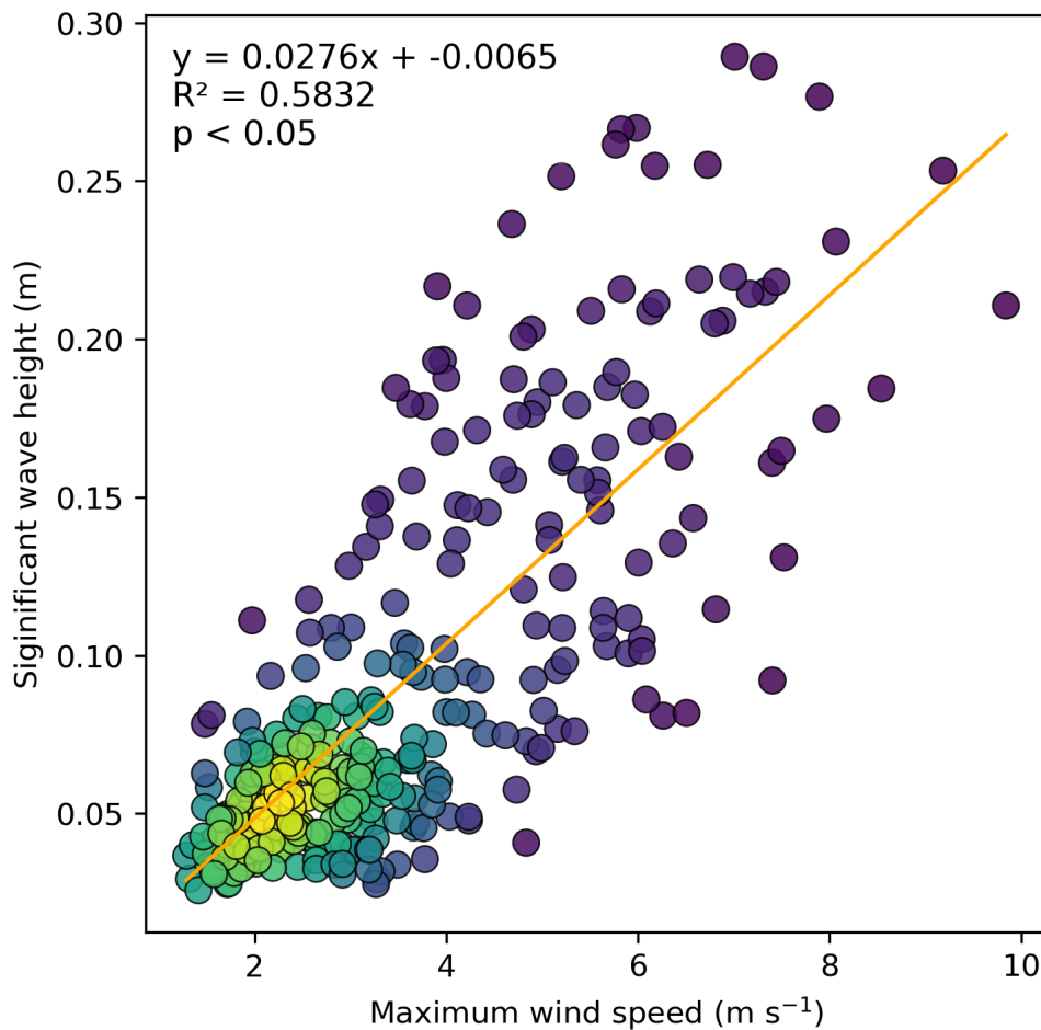
Figure 13: Relationship between maximum wind speed and significant wave height at the offshore of the Bengkalis Island (St. M). A significant positive relationship ( p < 0.05 , t-test) indicates that the regression is not a random coincidence.
