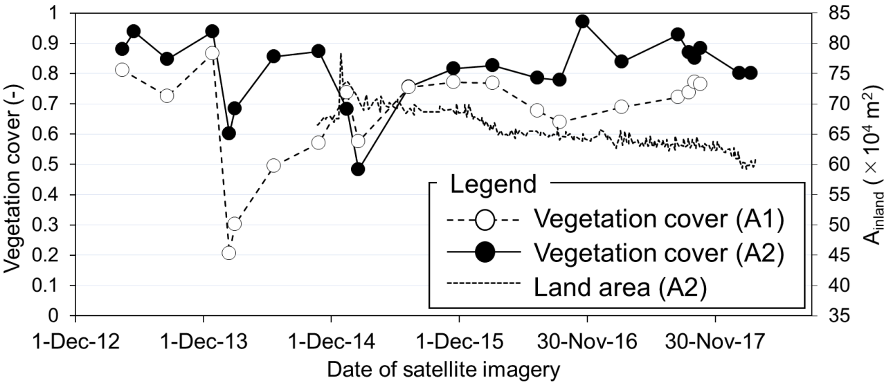
Figure 9: Time series of estimated vegetation covers in landslide-affected areas. Vegetation covers rapidly decreased from 27 December 2013 to 13 February 2014, dropping from 0.87 to 0.21 (Fig. 3c A1). Similarly, vegetation covers rapidly decreased from 27 October 2014 to 16 February 2015, declining from 0.87 to 0.48 (Fig. 3c A2). The land experienced a sudden extension, increasing by approximately 18.4 \times 10^4 \text{ m}^2 between December 22 and 28, 2014 (Fig. 3c A2).
