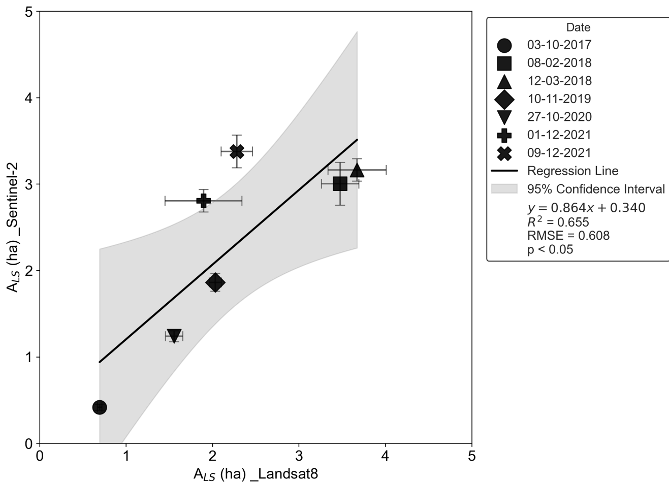
Figure 11: Evaluation of resolution-induced errors using Landsat 8 and Sentinel-2 imagery. A significant positive relationship ( p < 0.05 , t-test) indicates that the regression is not a random coincidence.
