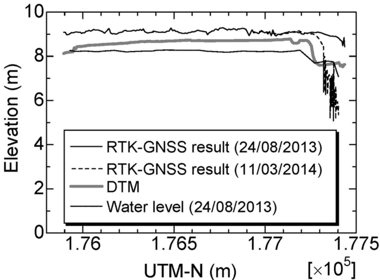
Figure F3: Comparison of the RTK-GNSS land survey with a section created from DEMNAS data. The section where the elevations of DTM has decreased was the section where the collapse was identified in December 2013 after the RTK-GNSS land survey. The RMSE of removing the landslide-affected area was 0.6951 (m).
