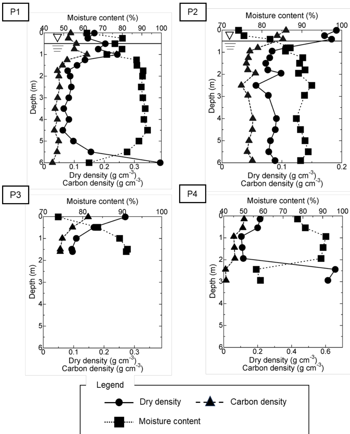
Figure 16: Vertical distribution of dry density of peat, carbon density, and moisture content by peat core analysis in Bengkalis Island.
