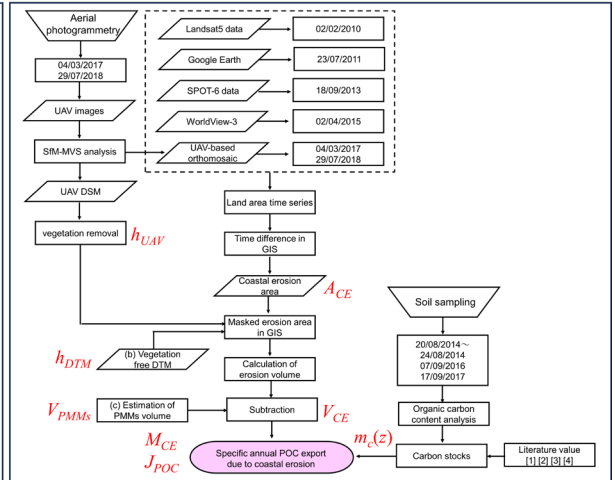
(f) Estimation of specific annual POC export into ocean due to coastal erosion
