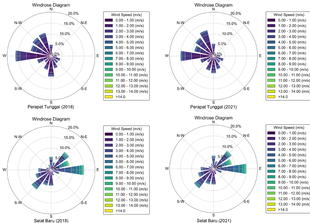
955 Figure J1: Annual wind rose diagrams for Perapat Tunggal and Selat Baru in 2018 and 2021.
