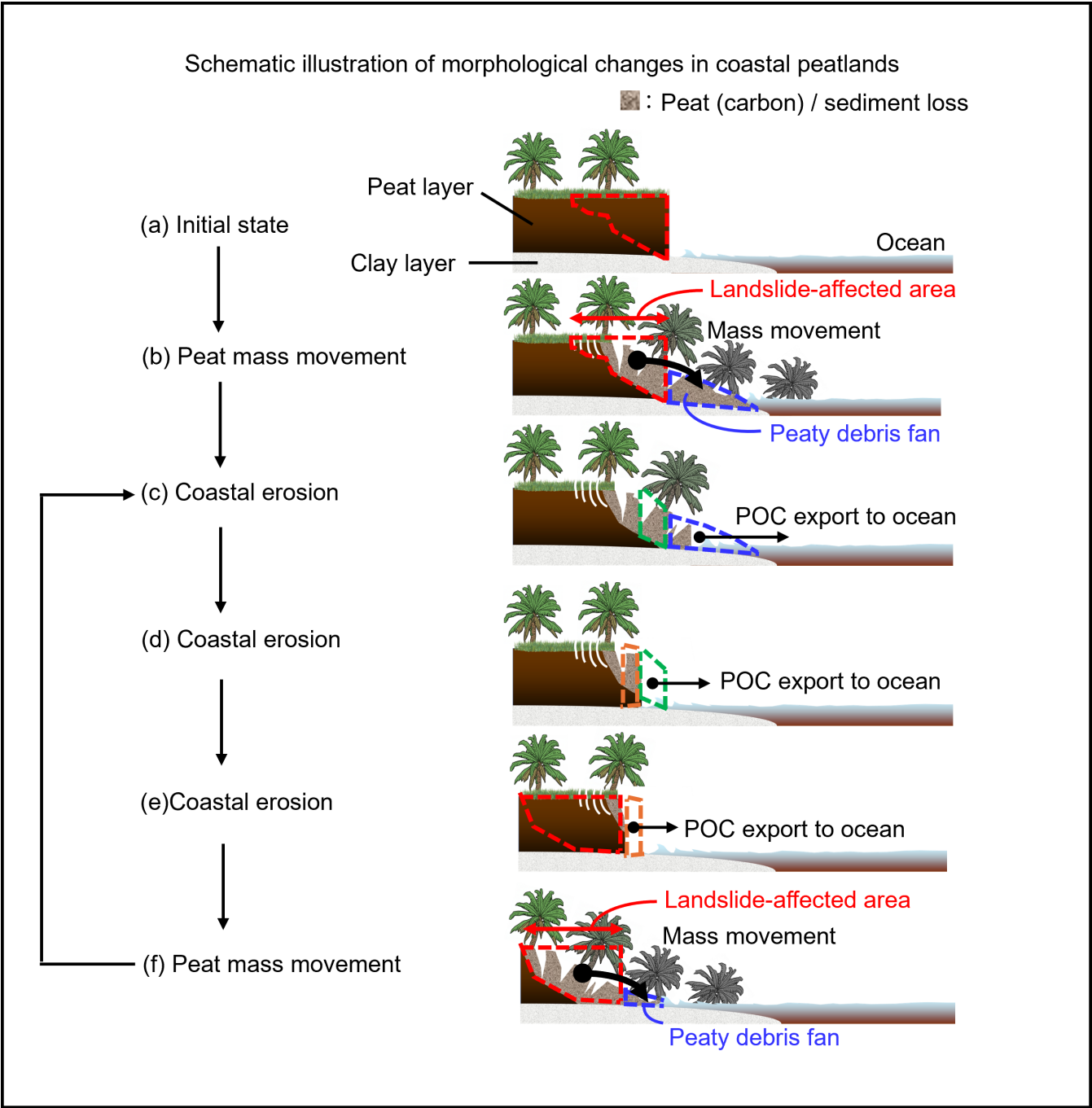
565 Figure 15: Conceptual diagram illustrating the lateral degradation processes in tropical peatlands. (a) shows the conditions around the 1960s, when the loss of mangrove belts reduced wave attenuation and initiated coastal erosion, resulting in the formation of peat cliffs. (b) illustrates a peat mass movement (PMM) triggered at the head scarp, where surface tears developed and a peaty debris fan extended seaward. Subsequent stages (c)–(e) depict the progressive
