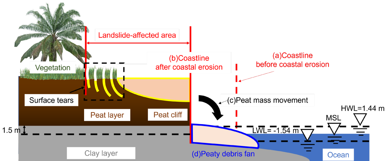
Figure 2: Conceptual figure of coastal erosion and PMMs on the peatland coast. Where the High-Water Level (HWL) is 1.44 m, the Mean Sea Level (MSL) is 0 m, and the Low Water Level (LWL) is -1.54 m. (a)-(d) show the transitional changes in the coastal landform and a cross-section of the coast. (a) coastline before coastal erosion; (b) coastline after coastal erosion; (c) trace of where PMM occurred; and (d) peaty debris fan formed by peat overhanging the coastline due to the occurrence of PMMs. When PMMs occur, cracks through the peat layer, known as surface tears, appear in the hinterland. In this study, the area affected by the landslide was defined as the hinterland from the peaty debris fan to the head of the source of surface tears. Landslide-affected areas have a thinner vegetation cover.
