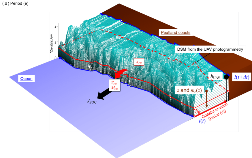
Figure 5: Illustrative image of abbreviations. (a) Model of abbreviations associated with peat mass movement events; (b) Model of abbreviations associated with coastal erosion.
