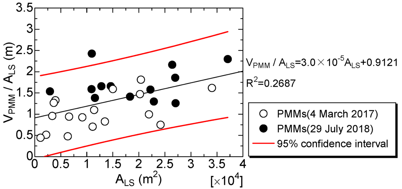
Figure 6: Area-Volume/Area relationship of a peat mass movement event. Where, A_{LS} is landslide-affected area, V_{PMM} is the loss of the peat volume due to a PMM event. There is a linear relationship between A_{LS} and V_{PMM} / A_{LS} ; If V_{PMM} / A_{LS} is assumed to be the depth of landslide-affected area, the greater the A_{LS} , the deeper the depth of the collapse. It was found that the ground level drop was around 0.91 m in small collapses.
