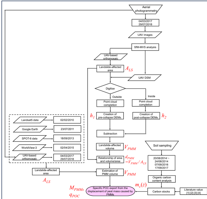
(e) Estimation of the Specific POC export from the displacement of peat mass caused by PMMs
