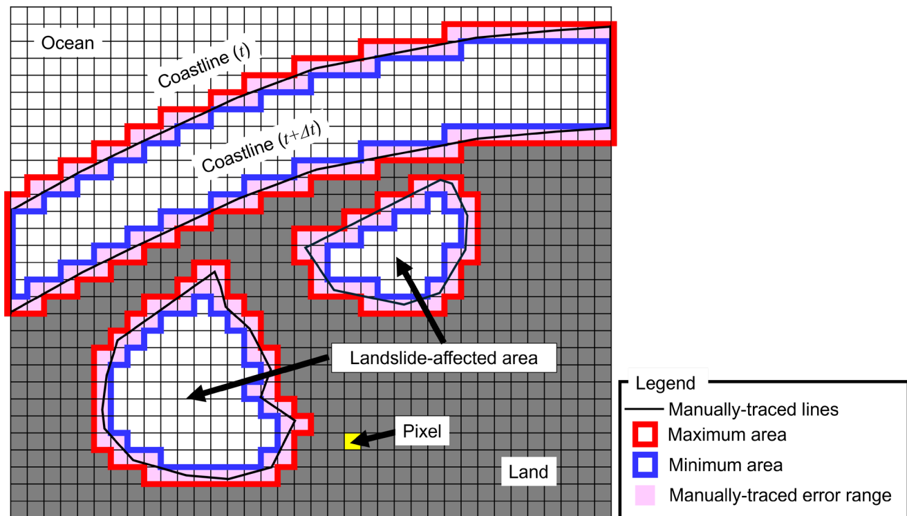
Figure H1: Concept of the error evaluation method for traced coastal erosion areas and landslide-affected areas in the GIS software. Manual tracing errors tend to be resolution dependent.
