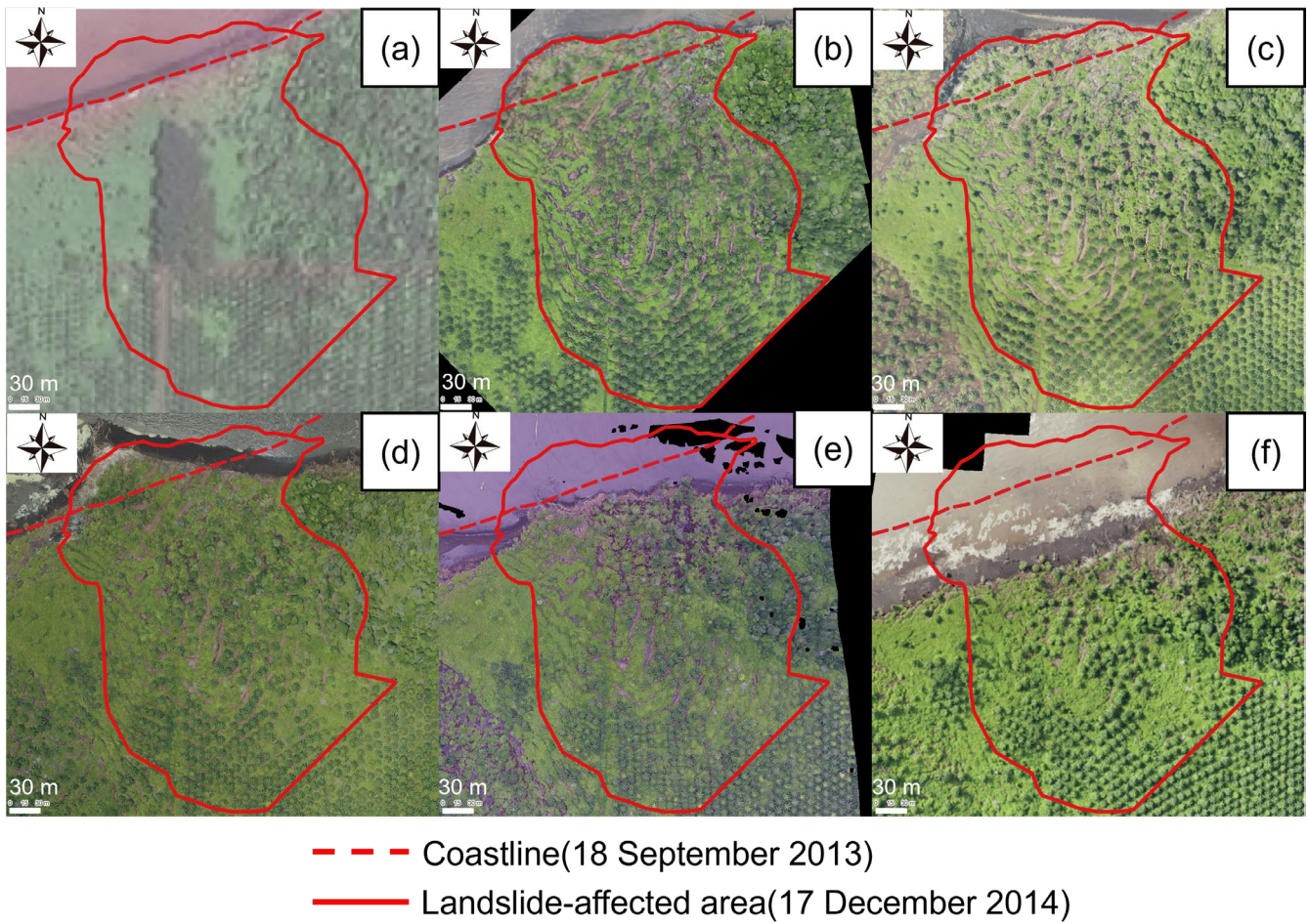
Figure 14: Annual changes at the landslide-affected area in the northwestern part of Bengkalis Island. (a) Initial status of the focus area with a peat cliff coastline (SPOT-6, 18 September 2013). (b) The immediate aftermath of a peat mass movement; a peaty debris fan was confirmed outside the initial coastline, with many tears observed on the ground surface of the hinterland (UAV-based orthomosaic, 17 Dec. 2014). (c) A larger peat mass movement occurred in the western area, creating a second peat fan, while the first peat fan remained (UAV-based orthomosaic, 10 Jan. 2015). (d) The second peaty debris fan in the west area completely disappeared, while the first peaty debris fan remained (UAV-based orthomosaic, 5 Mar. 2016). (e) Gradually, the first peaty debris fan eroded and decreased in area (UAV-based orthomosaic, 4 Mar. 2017). (f) The first peaty debris fan disappeared, and the coastline receded approximately 90 m from the initial status on average, returning to a peat cliff (UAV-based orthomosaic, 29 Jul. 2018).
