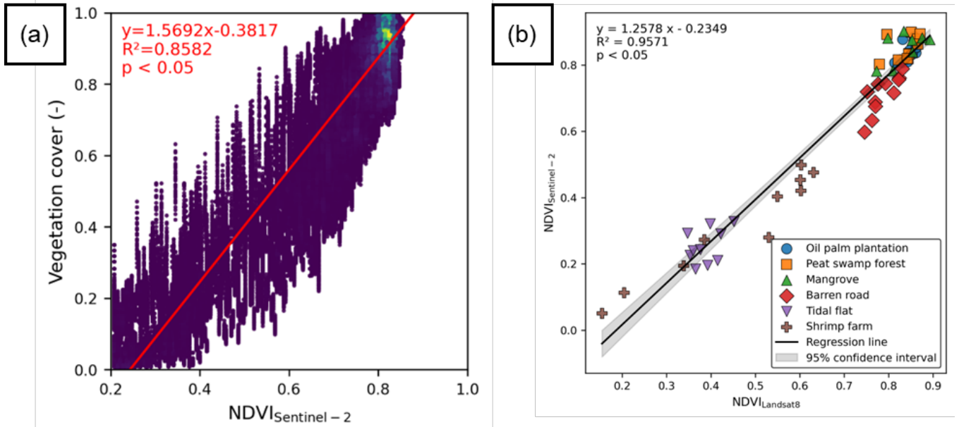
Figure D1: (a): Relationship between Sentinel-2 NDVI and vegetation cover (b): Relationship between Landsat 8 NDVI and Sentinel-2 NDVI, and Both figures show a linear relationship. A significant positive relationship ( p < 0.05 , t-test) indicates that the regression is not a random coincidence.
