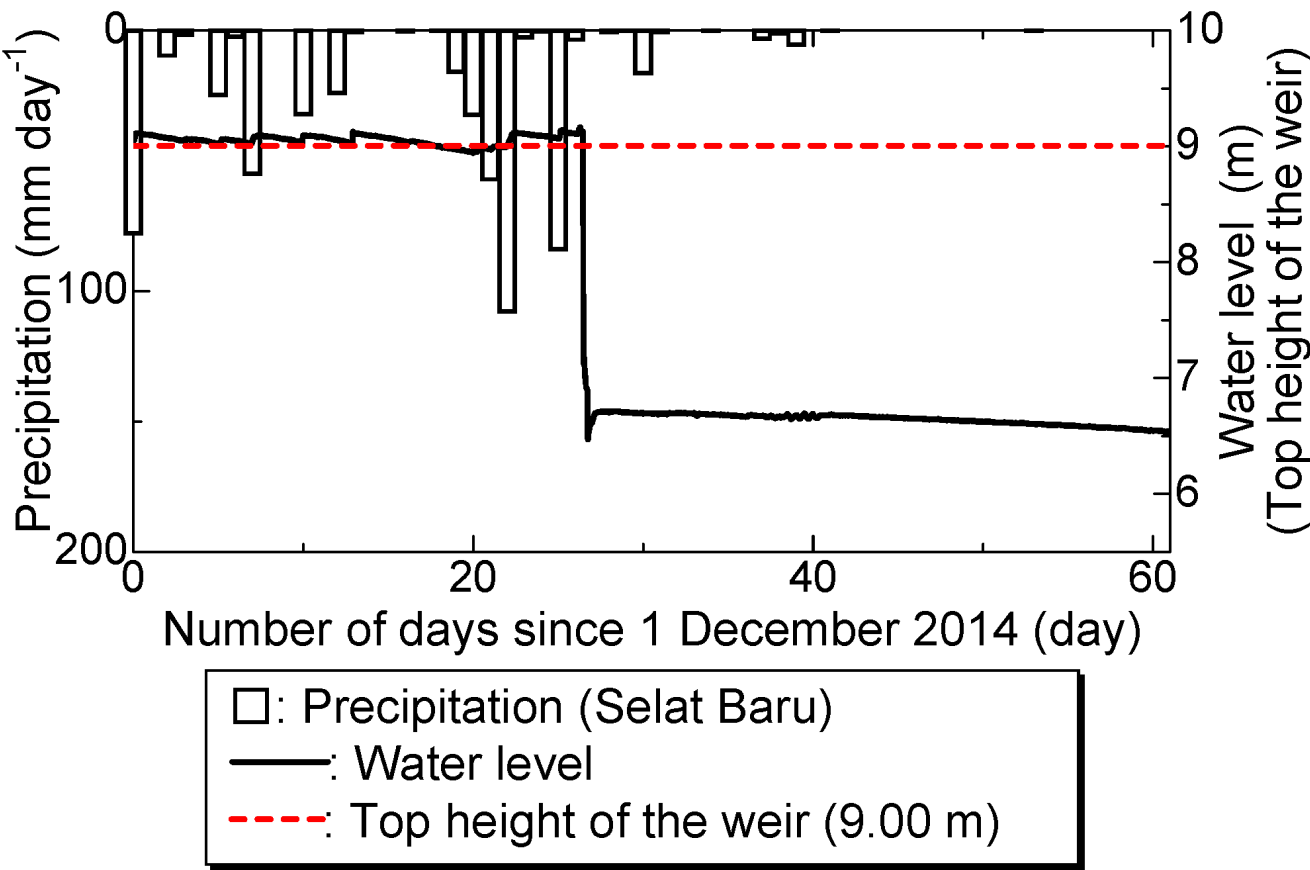
480 Figure 11: Water level of the water way at WP1 and precipitation at Selat Baru station during the peat mass movement event on 27th Dec. 2014. The major precipitation before the event were 107.9 \text{ mm day}^{-1} (Dec. 23) and 84.1 \text{ mm day}^{-1} (Dec. 26). Subsequently, the water level of the water way dropped suddenly on Dec. 27, 2014. The top height of the weir was 9.00 m, but the water level was recorded at 9.124 m at 11:10 on December 27, 2014, followed by a sudden drop to 7.896 m just 10 minutes later.
