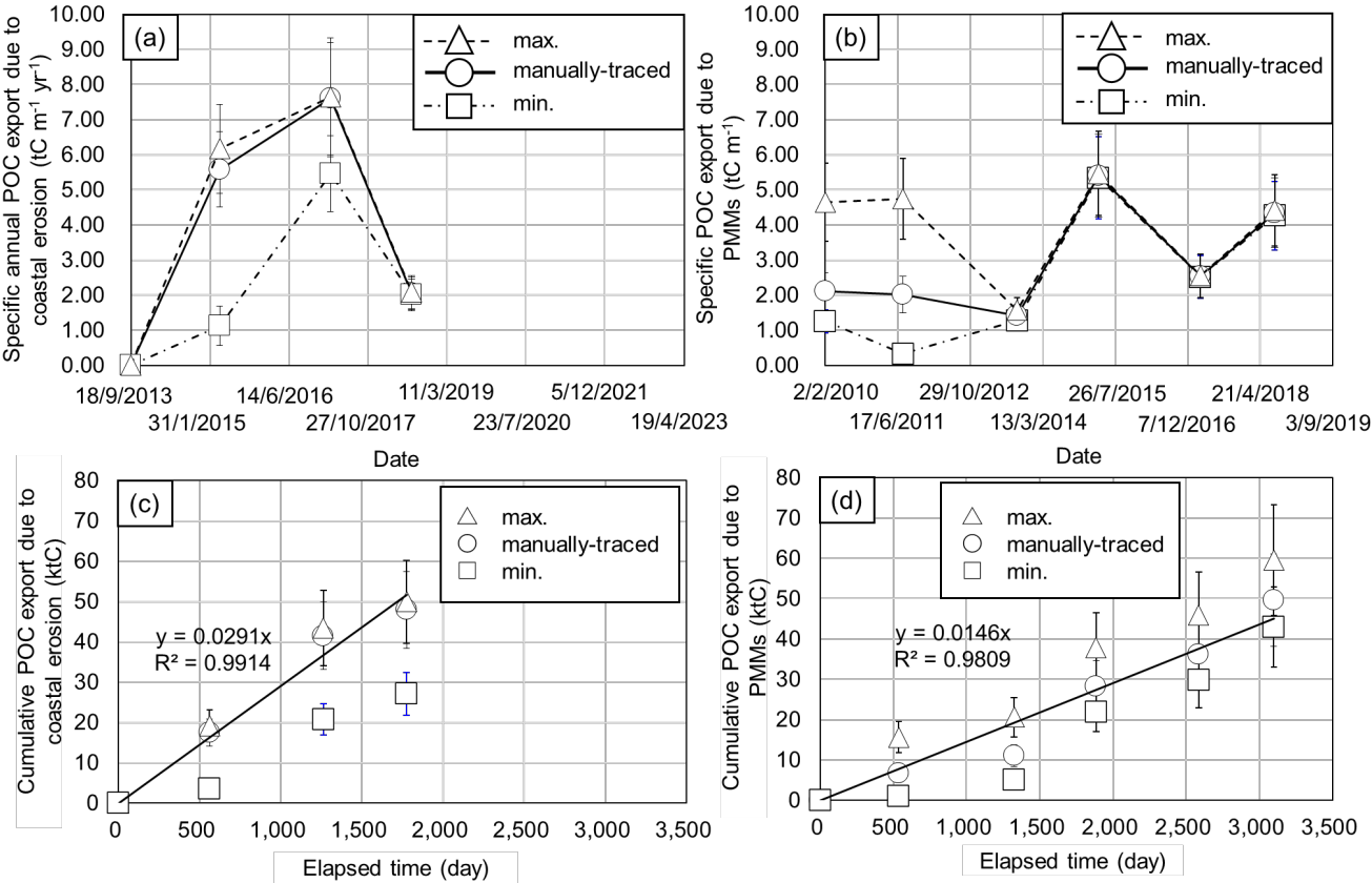
Figure 19: Time series of (a) estimated specific annual POC export due to coastal erosion and (b) estimated POC export due to displacement of peat mass caused by PMMs for observation moment. The average specific annual POC export of POC to the ocean was estimated to be 2.06 to 7.60 tC m -1 yr -1 by coastal erosion and 1.43 to 5.41 tC m -1 from PMMs. The error bars indicate the standard deviation (SD). Panels (c) and (d) show the cumulative POC export derived from the time series in (a) and (b), indicating that the observed POC export is driven due to coastal erosion and PMMs.
