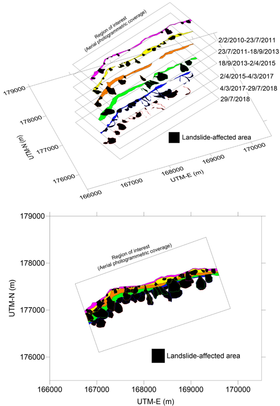
Figure 18: History of coastal erosion and landslide-affected area within the region of interest (0.68 km 2 ). This figure shows that the coastal erosion and peat mass movements occurred by turn and the landslide-affected area had been expanding towards the hinterland.
