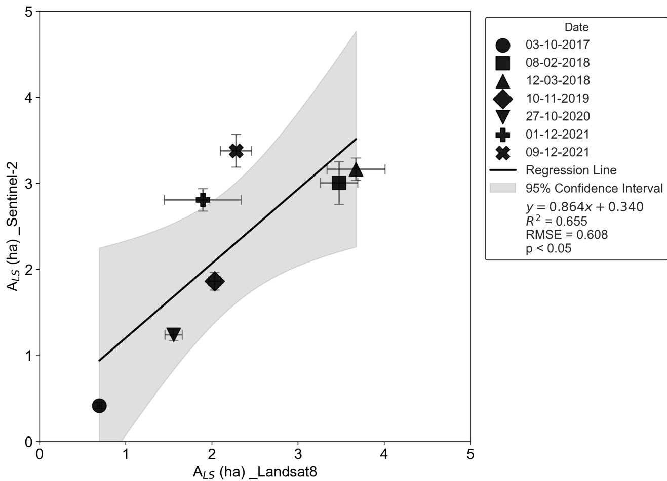
Figure I1: Evaluation of resolution-induced errors using Landsat 8 and Sentinel-2 imagery. A significant positive relationship ( p < 0.05 , t-test) indicates that the regression is not a random coincidence.
