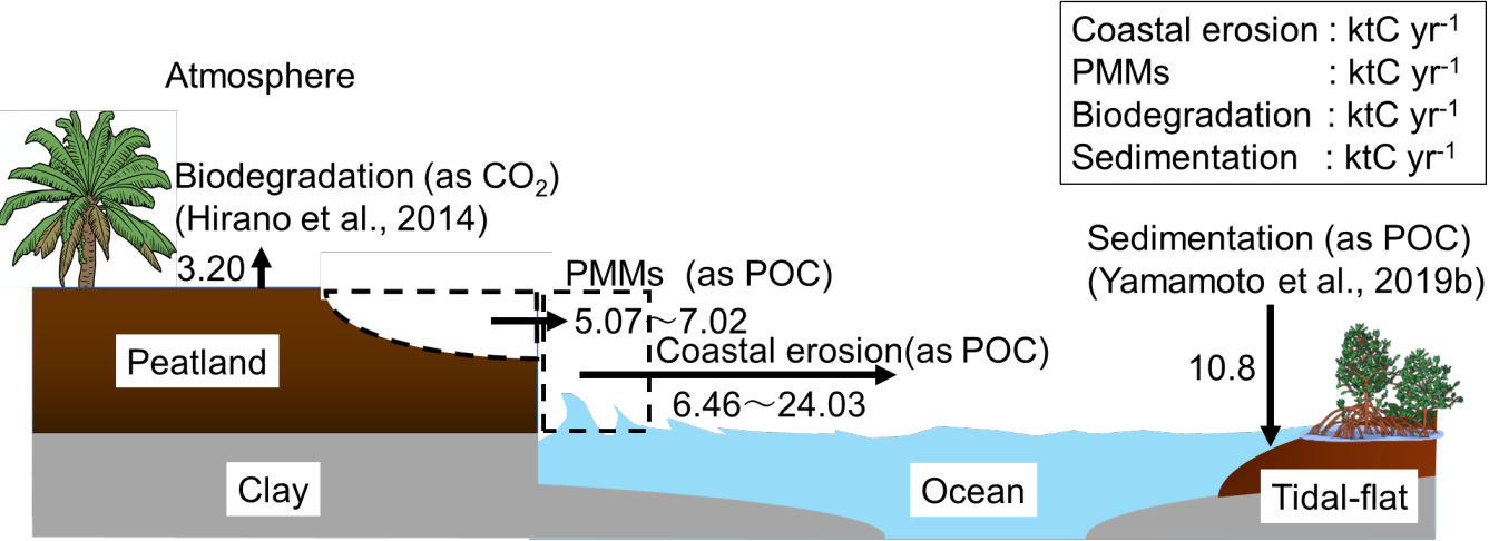
Figure 20: Estimated annual particulate organic carbon (POC) flux around the studied peatland watershed (6.41km 2 ) in Bengkalis Island. Biodegradation was referred to Hirano et al., 2014. The coastline along the peatland watershed was 3.1 km and the area of the tidal flat in Bengkalis Island where the sedimentation happened was 1.46 km 2
