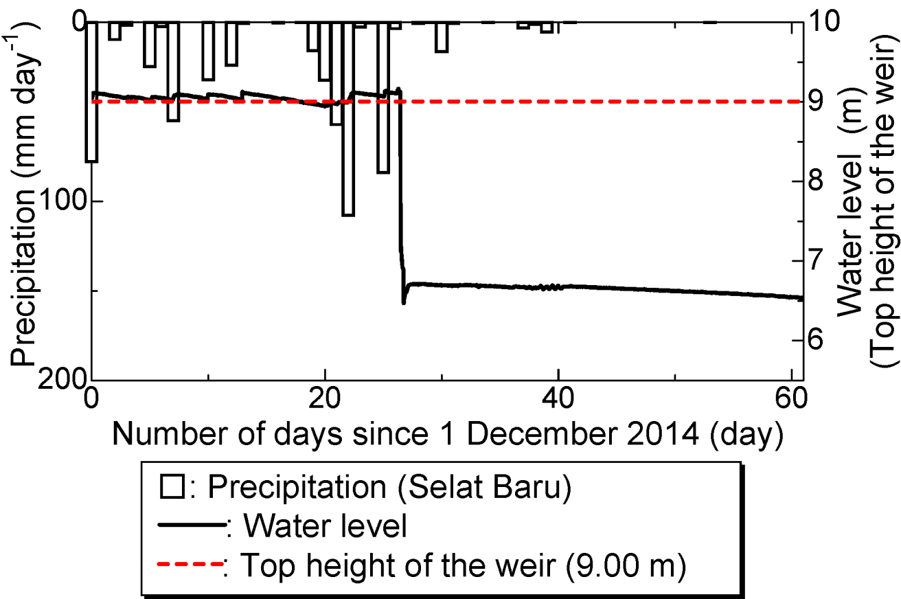
480 Figure 11: Water level of the water way at WP1 and precipitation at Selat Baru station during the peat mass movement event on 27th Dec. 2014. The major precipitations before the event were 107.9 \text{ mm day}^{-1} (Dec. 23) and 84.1 \text{ mm day}^{-1} (Dec. 26). Subsequently, the water level of the water way dropped suddenly on Dec. 27, 2014. The top height of the weir was 9.00 m, but the water level was recorded at 9.124 m at 11:10 on December 27, 2014, followed by a sudden drop to 7.896 m just 10 minutes later.
