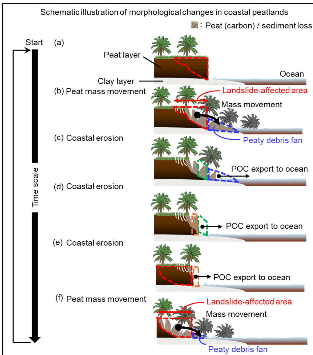
Figure 15: Conceptual diagram illustrating the lateral degradation processes in tropical peatlands. (a) shows the conditions around the 1960s, when the loss of mangrove belts reduced wave attenuation and initiated coastal erosion, resulting in the formation of peat cliffs. (b) illustrates a peat mass movement (PMM) triggered at the head scarp, where surface tears developed and a peaty debris fan extended seaward. Subsequent stages (c)–(e) depict the progressive erosion of the debris fan and the landslide-affected area, leading to the direct export of particulate organic carbon (POC) to the ocean. (f) shows the stage at which the coastal peat cliff has been rebuilt by ongoing erosion, allowing a new PMM to occur and thereby completing the cyclic process of lateral degradation.
