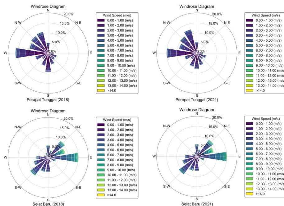
Figure J1-44: Annual wind rose diagrams for Perapat Tunggal and Selat Baru in 2018 and 2021.
