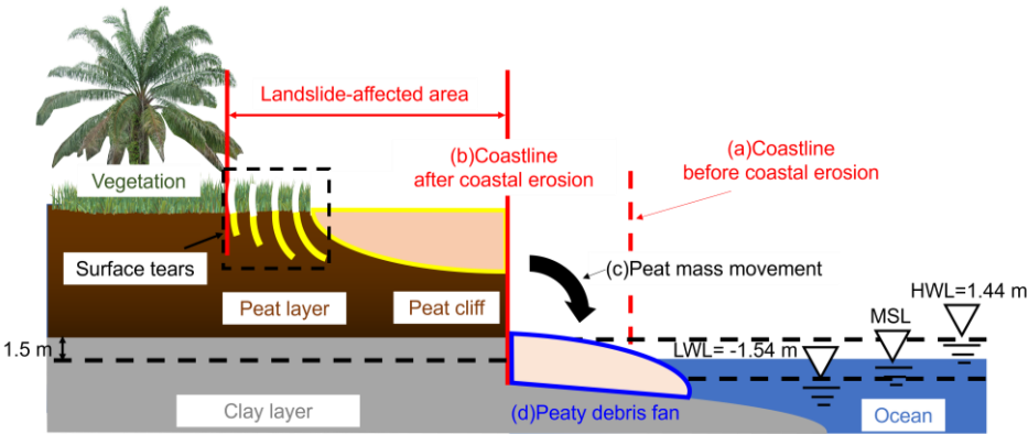
Figure 2: Conceptual figure of coastal erosion and PMMs on the peatland coast. Where the High-Water Level (HWL) is 1.44 m, the Mean Sea Level (MSL) is 0 m, and the Low Water Level (LWL) is -1.54 m. (a)~(d) show the transitional changes in the coastal landform and a cross-section of the coast. (a) coastline before coastal erosion; (b) coastline after coastal erosion; (c) trace of where PMM occurred; and (d) peaty debris fan formed by peat overhanging the coastline due to the occurrence of PMMs. When PMMs occur, cracks through the peat layer, known as surface tears, appear in the hinterland. In this study, the area affected by the landslide
