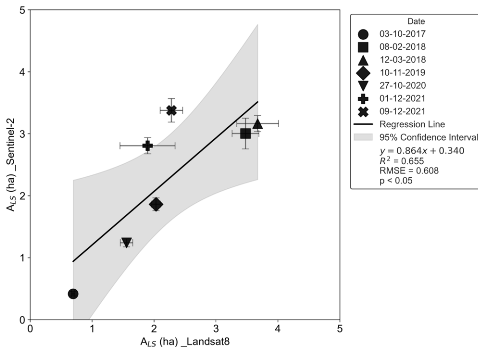
965 Figure II: Evaluation of resolution-induced errors using Landsat 8 and Sentinel-2 imagery. A significant positive relationship ( p < 0.05 , t-test) indicates that the regression is not a random coincidence.
