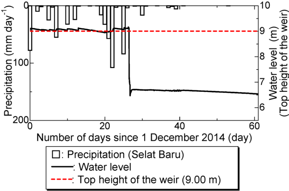
Figure 11: Water level of the water way at WP1 and precipitation at Selat Baru station during the peat mass movement event on 27th Dec. 2014. The major precipitations before the event were 107.9 \text{ mm day}^{-1} (Dec. 23) and 84.1 \text{ mm day}^{-1} (Dec. 26). Subsequently, the water level of the water way dropped suddenly on Dec. 27, 2014. The top height of the weir was 9.00 m, but the water level was recorded at 9.124 m at 11:10 on December 27, 2014, followed by a sudden drop to 7.896 m just 10 minutes later.
