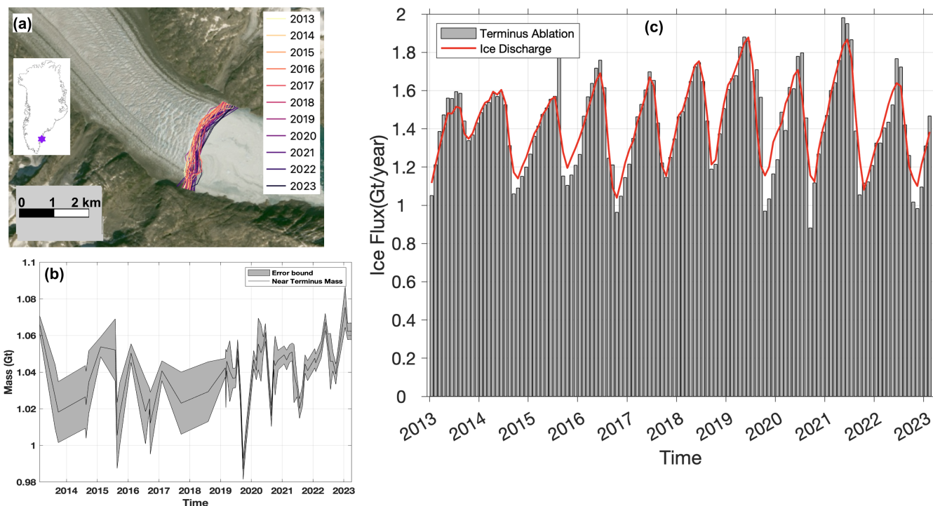
Figure 5. Heidmdal Glacier (coordinates: -42.67188^{\circ}\text{W} , 62.9001^{\circ}\text{N} ). (a) Terminus positions for Heidmdal Glacier during 2013–2023 displayed on a true-color composite Sentinel-2 image (courtesy of European Space Agency, Copernicus). The inset of Greenland with a purple star shows the glacier location. (b) Time series of mass within the terminus polygon (Gt) with uncertainty shown as gray shading. (c) Time series for terminus ablation and discharge in gigatons per year (Gt/yr).
