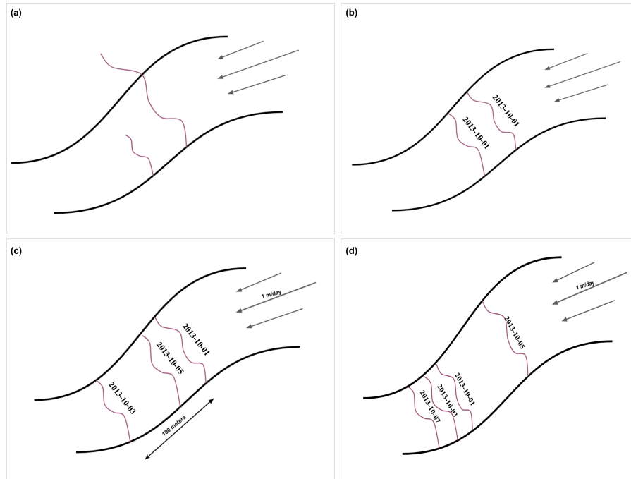
Fig. 4. Issues associated with terminus positions from TermPicks and CALFIN: (a) incomplete terminus traces extend beyond the fjord wall; (b) duplicate traces for the same day; (c) anomalous advance where the terminus position moved faster than possible based on independent speed estimates; and (d) anomalous retreat, a similar condition to (c), where the terminus is anomalously retreated relative to the subsequent observations. Arrows show the direction of glacier flow.
