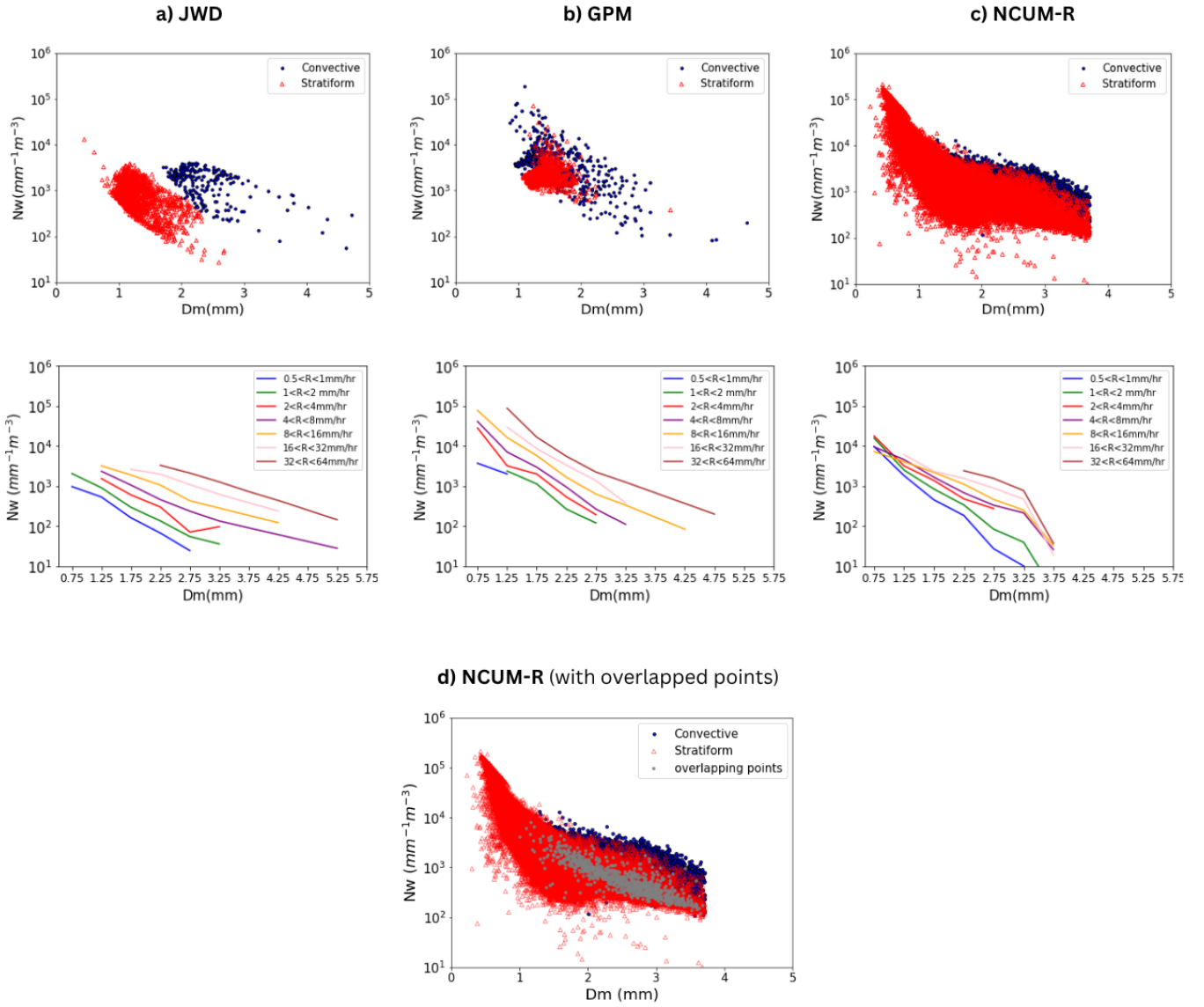
Figure 7. Scattered plot of Nw vs Dm segregated to different rain types(convective and stratiform)(top row) and Nw vs Dm for different Rainrates (second row) of JWD, GPM and NCUM-R (a,b and c).(d) shows the NCUM-R scattered figure with overlapping of convective and stratiform points
