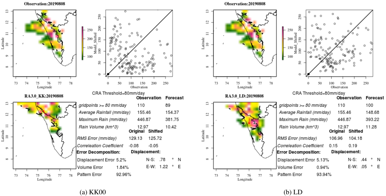
Figure 9. CRA analysis of convective event on 8th August 2019
