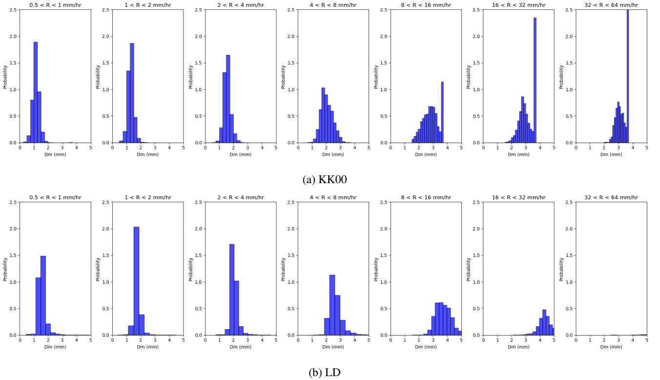
Figure 8. Frequency of drops corresponding to different diameters( D_m ) in each rain rate intervals
