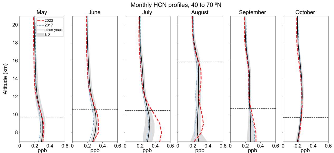
140 Figure 1: Monthly average HCN profiles from 40 to 70° N measured by ACE-FTS. The red curves show monthly averages in 2023, and the black curves show monthly averages from 2004–2022 with the grey shaded area representing \pm one standard deviation from the 2004–2022 average. The blue dashed line indicates 2017 averages as it was an anomalous year with the PNE. The monthly average lapse rate tropopause altitudes calculated for 2023 are plotted as horizontal dashed lines for reference.
