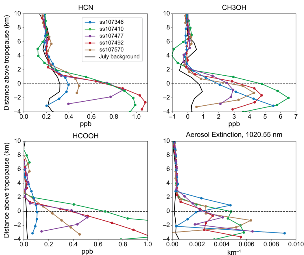
175 Figure 3: Tropopause-relative profiles for July 2023 occultations that exhibit enhanced wildfire product VMRs and aerosol extinction in the lower stratosphere. A background profile with no smoke from a similar location in July 2023, ss107249, is plotted for reference.
