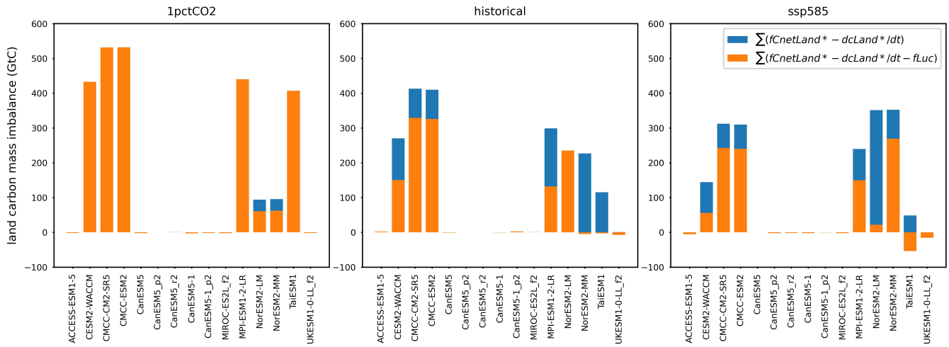
655 Figure A10. The carbon mass imbalance from mismatch of net land carbon flux ( f_{\text{CnetLand}}^* , with or without the consideration of fl_{\text{Luc}} , reconstructed from flux data) and the change in land carbon pool size over time ( dc_{\text{Land}}^*/dt , derived from pool size data) for CMIP6 ESMs across different scenarios.
