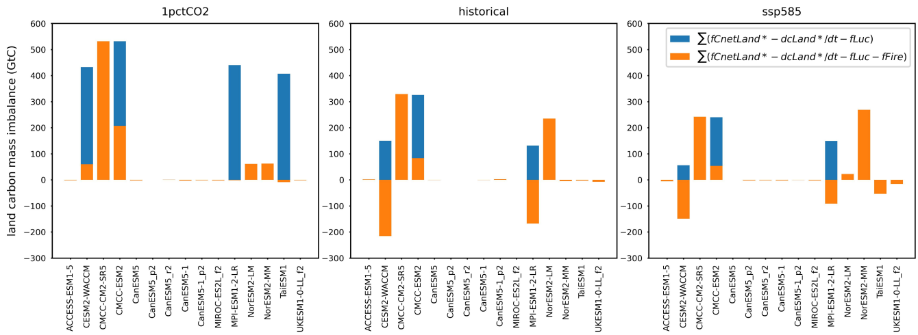
660 Figure A11. The carbon mass imbalance from mismatch of net land carbon flux ( f_{\text{CnetLand}}^* , with or without the consideration of ff_{\text{Fire}} , reconstructed from flux data) and the change in land carbon pool size over time ( dc_{\text{Land}}^*/dt , derived from pool size data) for CMIP6 ESMs across different scenarios.
