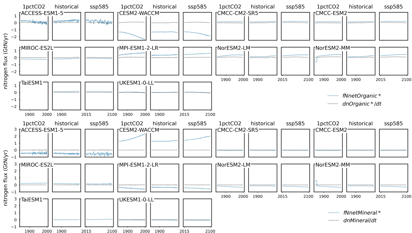
Figure A8. Comparison of net nitrogen fluxes for organic and mineral pools ( f_{\text{NnetOrganic}}^* and f_{\text{NnetMineral}}^* , reconstructed from flux data) and the change of nitrogen pool size over time for organic and mineral pools ( dn_{\text{Organic}}^*/dt and dn_{\text{Mineral}}/dt , derived from pool size data) from CMIP6 ESMs across different scenarios.
