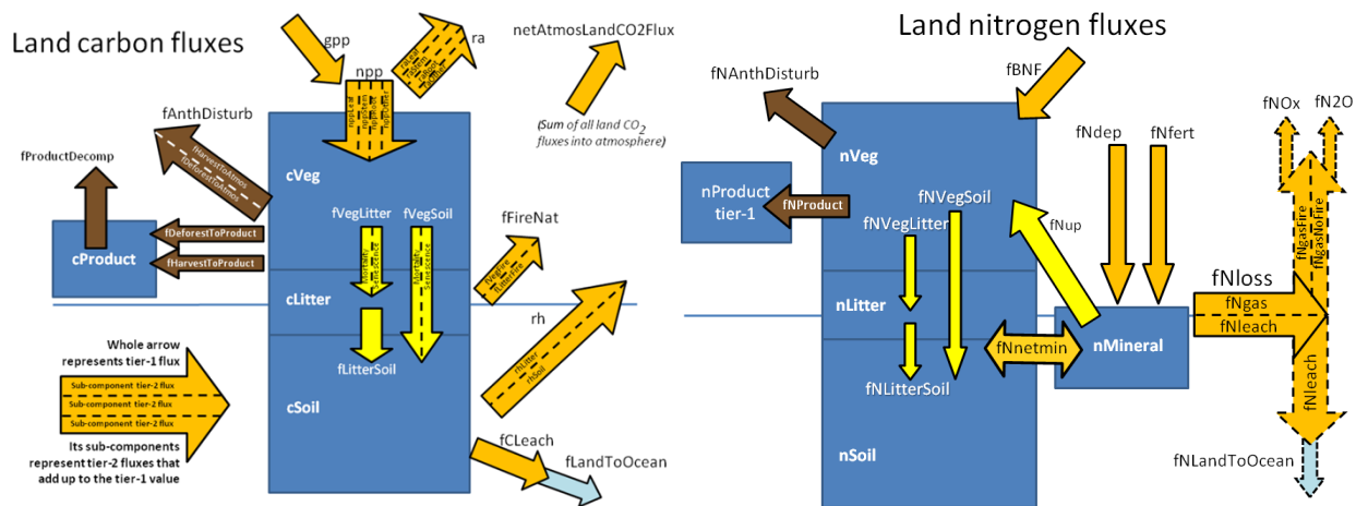
Figure 1. Land carbon-nitrogen pools and fluxes requested by the C4MIP protocol. The boxes represent pools, while the arrows indicate fluxes and their directions. Details of variable descriptions are provided in Table A1. This figure is reproduced from the C4MIP protocol (Jones et al., 2016) under the Creative Commons Attribution 3.0 License.
