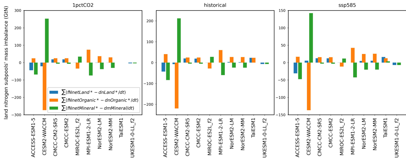
Figure 6. The nitrogen mass imbalance from mismatch of net nitrogen fluxes for total land, land organic, and land inorganic pools ( fN_{netLand}^* , fN_{netOrganic}^* , and fN_{netMineral}^* , calculated from flux data) and the change of nitrogen pool size over time for total land, land organic, and land inorganic pools ( dn_{Land}/dt , dn_{Organic}/dt , and dn_{Mineral}/dt , derived from pool size data) for CMIP6 ESMs across different scenarios.
