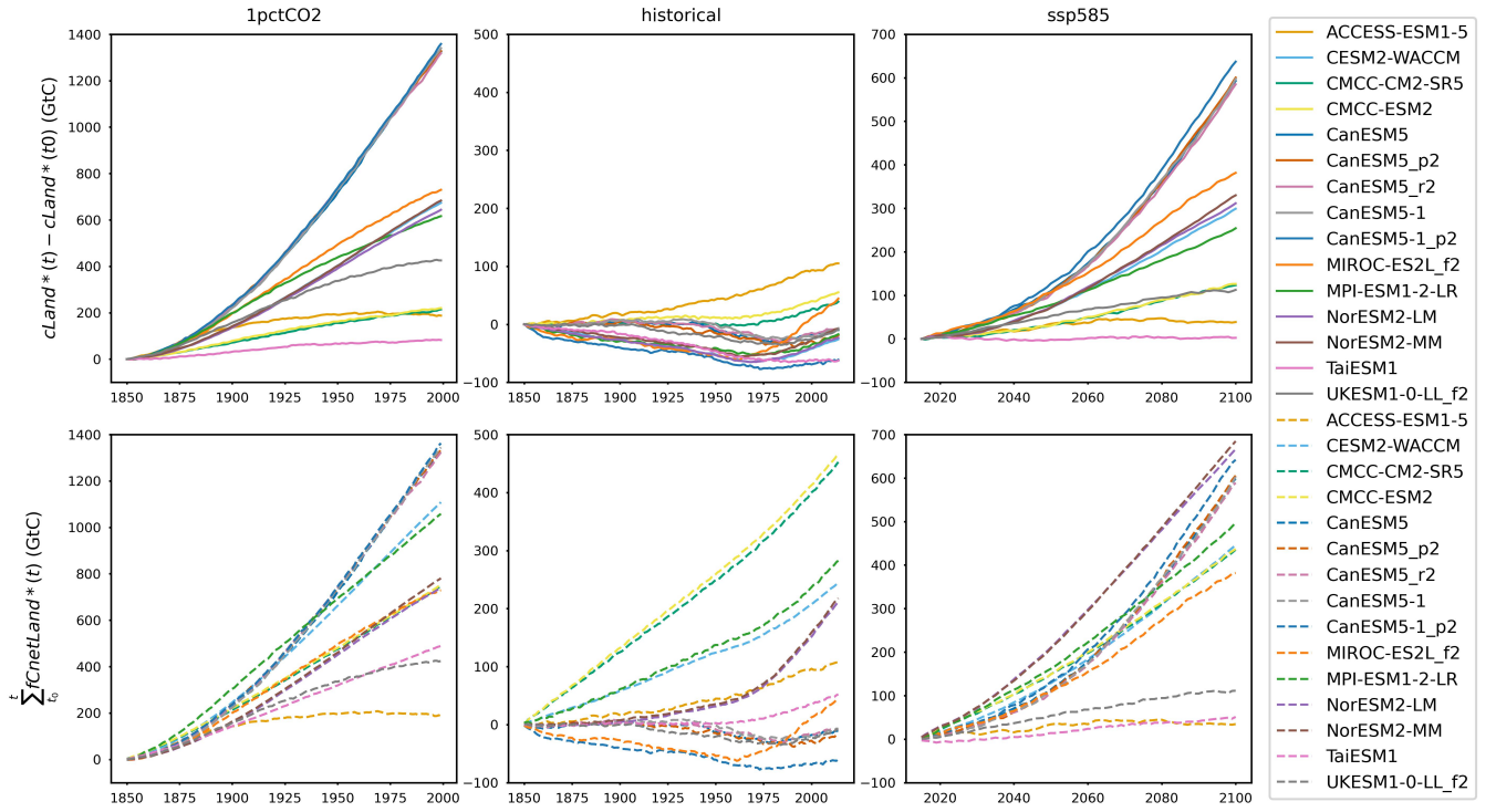
Figure A6. The mismatch of changes in land carbon pool size derived from pool size data [cLand^*(t) - cLand^*(t_0)] (solid lines) and those retrieved from the integration of net land carbon flux reconstructed from flux data ( fCnetLand^* , dashed lines) in CMIP6 ESMS across different scenarios.
