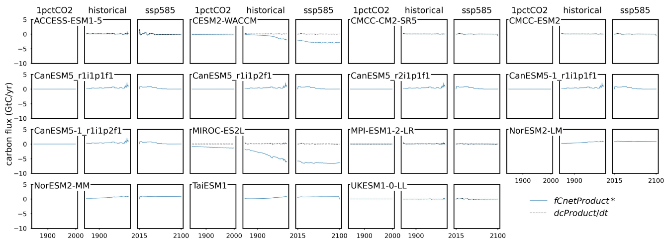
Figure A7. Comparison of net carbon flux for vegetation, litter+soil, and product pools ( f_{\text{CnetVeg}}^* , f_{\text{CnetLitterSoil}}^* , and f_{\text{CnetProduct}}^* , reconstructed from flux data) and the change of carbon pool size over time for vegetation, litter+soil, and product pools ( dc_{\text{Veg}}/dt , dc_{\text{LitterSoil}}/dt , and dc_{\text{Product}}/dt , derived from pool size data) from CMIP6 ESMs across different scenarios.
