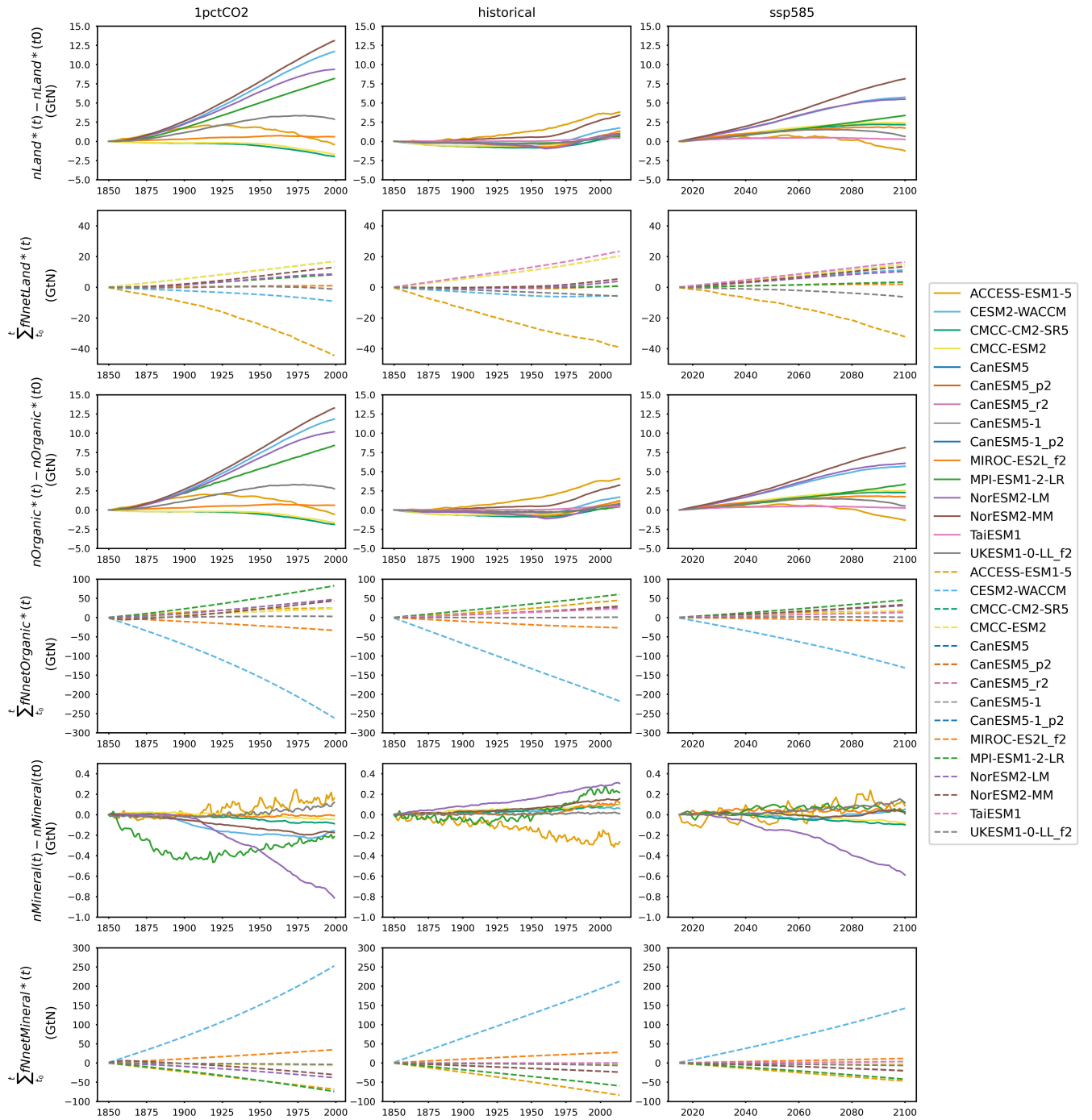
Figure A9. The mismatch of changes in land nitrogen pool size derived from pool size data [land nitrogen: n_{Land}^*(t) - n_{Land}^*(t_0) ; organic nitrogen: n_{Organic}^*(t) - n_{Organic}^*(t_0) , and mineral nitrogen: n_{Mineral}(t) - n_{Mineral}(t_0) ] (solid lines) and those retrieved from the integration of net nitrogen flux reconstructed from flux data (land nitrogen: f_{NetLand}^* , organic nitrogen: f_{NetOrganic}^* , and mineral nitrogen: f_{NetMineral}^* , dashed lines) in CMIP6 ESMs across different scenarios. Note there is no nitrogen cycle in CanESM.
