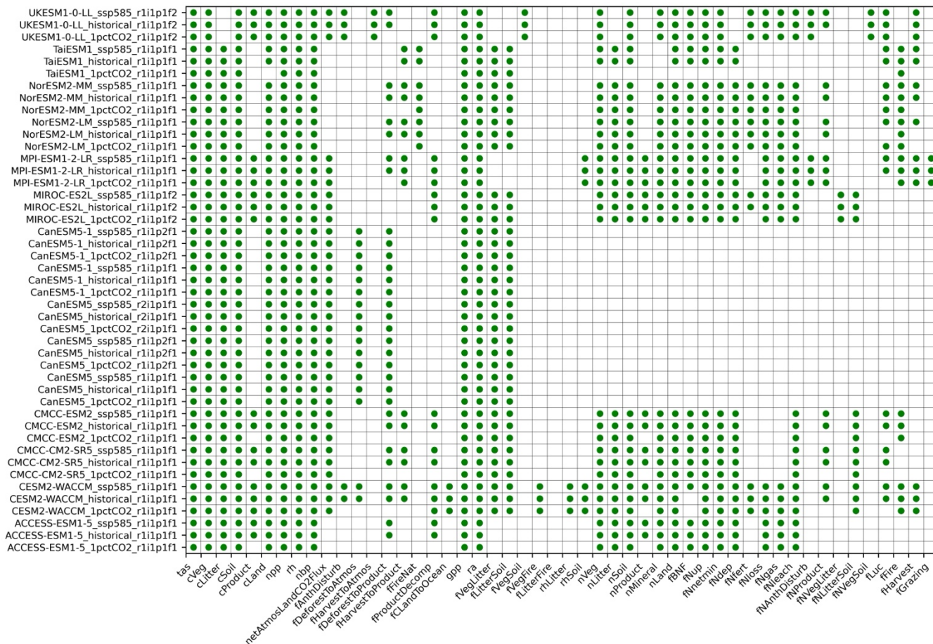
Figure A1. Overview of data availability for the studied CMIP6 ESMs and experiments. The green dots indicate the data is available from ESGF.
