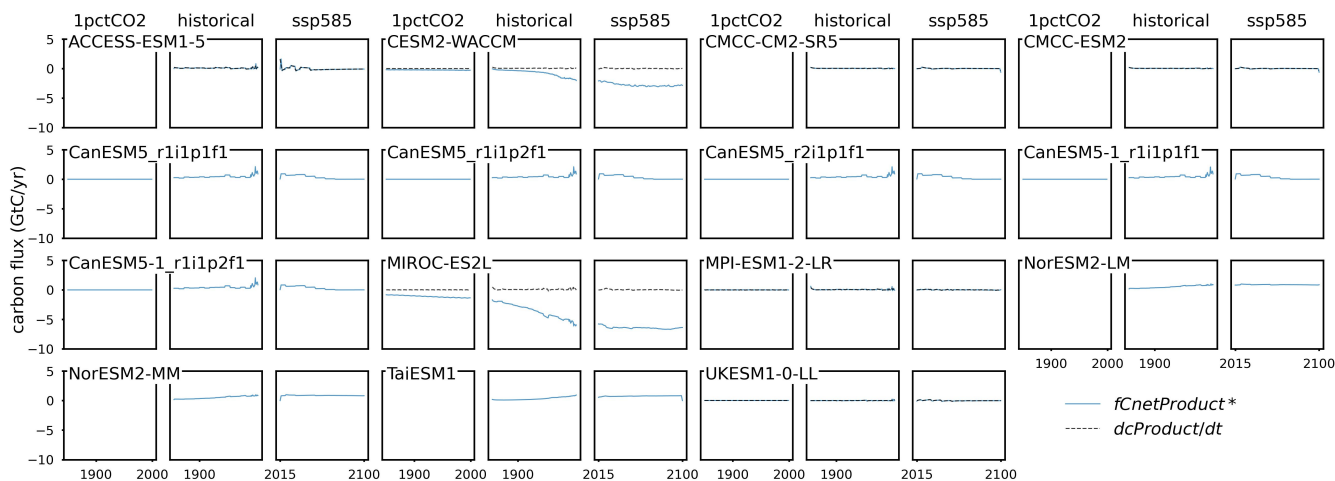
Figure A7. Comparison of net carbon flux for vegetation, litter+soil, and product pools ( f_{\text{NetVeg}}^* , f_{\text{NetLitterSoil}}^* , and f_{\text{NetProduct}}^* , reconstructed from flux data) and the change of carbon pool size over time for vegetation, litter+soil, and product pools ( dc_{\text{Veg}}/dt , dc_{\text{LitterSoil}}/dt , and dc_{\text{Product}}/dt , derived from pool size data) from CMIP6 ESMs across different scenarios.
