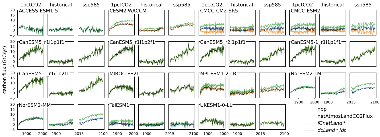
145 Figure 2. Comparison of ‘net biosphere production’ (nbp), netAtmosLandCO2Flux, net land carbon flux (fCnetLand*, reconstructed from flux data), and the change of land carbon pool size over time (dcLand*/dt, derived from pool size data) from CMIP6 ESMs across different scenarios
