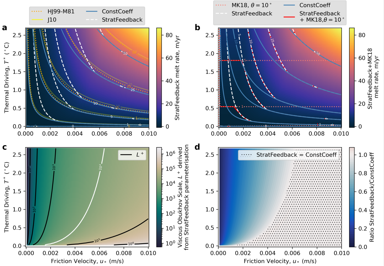
Figure 2. Thermal driving – friction velocity phase-parameter space diagram indicating melt rates calculated as a function of far-field temperature, salinity and pressure (which are set to S = 34.5 psu and p = 500 dbar) and friction velocity. The melt rates are solved for a variety of parameterisation options in (a) and (b). The orange, dotted lines in panel (a) are the Holland and Jenkins (1999) formulation with the \eta_* stratification parameter (McPhee, 1981). A constant transfer coefficient formulation (ConstCoeff) is in the blue solid lines (using the maximal values of Vreugdenhil and Taylor (2019), which is similar to Jenkins et al. (2010) in the light yellow solid lines), and the stratification feedback (StratFeedback) parameterisation we develop here is shown in white solid-dashed lines. In panel (b), we add in the constant melt rates obtained from McConnochie and Kerr (2018) with a slope angle of \theta = 10^\circ from the horizontal in the pink dotted line, and the combination of the StratFeedback+MK18 limit in the red dash-dot line. Panel (c) shows the viscous Obukhov scale L^+ derived from the stratification feedback parameterisation, and where the white L^+ = 1 \times 10^4 indicates where the white dashed lines (StratFeedback) and blue line (ConstCoeff) transition from having the same melt rate to the right and different to the left. Panel (d) also shows this in the ratio of the StratFeedback to ConstCoeff melt rates, with stippling indicating where they are equal.
