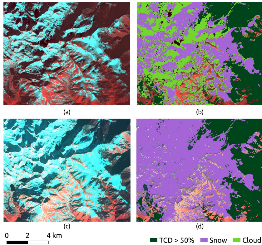
Figure C3. Alps 03 December 2013: 12x12 km 2 scene with a) Landsat 8 OLI image (Green, Red, SWIR); b) DLR-Landsat 2B product; c) SPOT 5 HRG image (Green, Red, SWIR); d) SWH 2B product.
