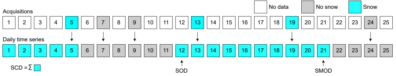
Figure 3. 25 days hydrological period of snow, no-snow and no-data days representing how snow periods are interpolated. The longest Snow Cover Duration (SCD) starts with the Snow Onset Day (SOD) on day 12 and ends with the Snow Melt-Out Day (SMOD) on day 21
