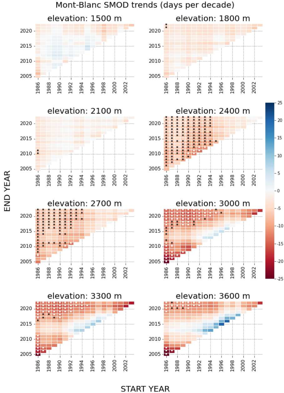
Figure 10. Mont-Blanc massif (French Alps). Results of the Mann–Kendall test over the trend of the SMOD median of each elevation band ( \pm 150 ) filtered for \text{NOBS}_{\min} \geq 10 and applied to all possible combinations of start and ending dates involving at least 20 years duration for the HY 1986 to 2022. Colors indicate the SMOD trend as days per decade, and dots indicate statistically significant trends ( p\text{-value} < 0.05 ).
