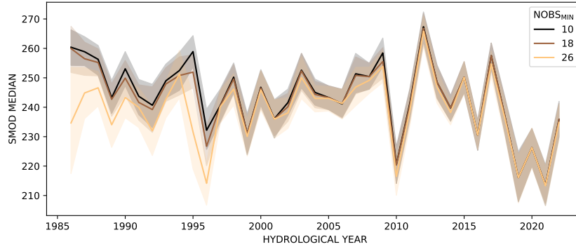
Figure D3. For \text{NOBS}_{\min} of 10, 18, and 26, yearly average of the SMOD medians from each combination of massif and elevation band, with a confidence interval of 95%. The distribution is robust to \text{NOBS}_{\min} except for earlier years at a \text{NOBS}_{\min} of 26 due to the significant reduction of available combinations.
