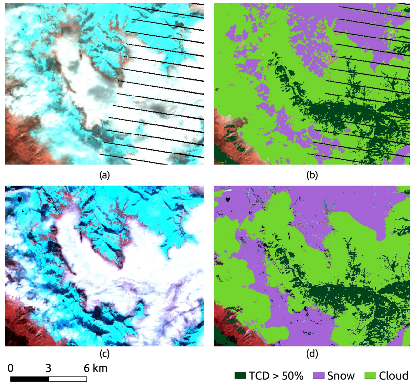
Figure C2. Alps 13 October 2005: 12x12 km 2 scene with a) Landsat 7 ETM+ image (Green, Red, SWIR); b) DLR-Landsat 2B product; c) SPOT 4 HRVIR image (Green, Red, SWIR); d) SWH 2B product.
