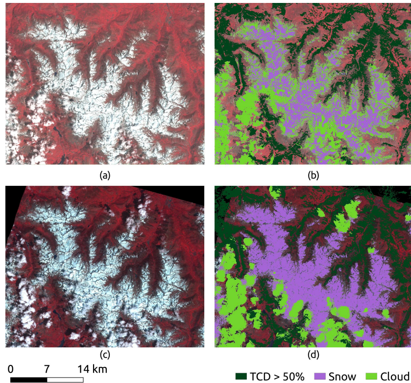
Figure C1. Pyrenees 25 May 1987: 30x30 km 2 scene with a) Landsat 5 TM image (Green, Red, SWIR); b) DLR-Landsat 2B product; c) SPOT 1 HRV image (Green, Red, NIR); d) SWH 2B product.
