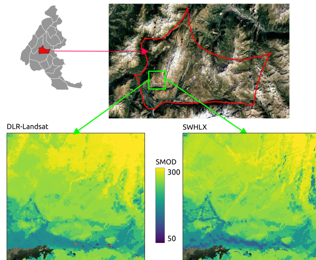
Figure 13. Alpe d'Huez, hydrological year 1997: comparison between the 20 m resolution SMOD maps from DLR-Landsat (left) and from SWHLX (right).
