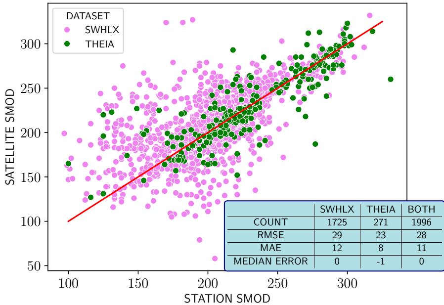
Figure 5. Scatterplots between satellite-based SMODs and station SMODs at HS_0 = 1 for the combination of Theia and SWHLX between the HY 1986 and 2018.
