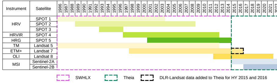
Figure 2. Satellite products distribution in the time series across the hydrological years. Dotted rectangles represent the datasets SWHLX (pink), Theia (green) and Landsat 7 products from DLR-Landsat (black) added to Theia.
