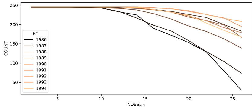
Figure D2. For every HYs below 1995, number of available SMOD medians from every combinations of massif and elevation bands as a function of NOBS min . A loss of data was observed for NOBS min thresholds above 10, with a stronger effect before 1989. For later periods, a NOBS min of 26 still allows to maintain most of the available combinations of massif and elevation. For 1986, a NOBS min of 26 reduces the available combinations of massif and elevation bands to 28.
