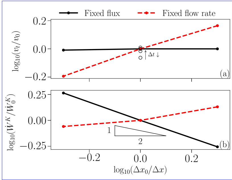
Figure E1. Mesh-dependency test for fixed-flux (solid black lines) and fixed-flow rate (dashed red lines) cases. The domain width is held constant while varying cell size of the mesh. (a) Variation of propagation speed ( v_t ) versus cell size ( \Delta x ). Solid circles represent variations in cell size with a fixed time step of \Delta t = 0.5 yr. Open circles that are aligned vertically represent variations in the time step ( \Delta t = 2, 1, 0.5, and 0.25 yr, from bottom to top). Decreasing \Delta t values leads to an increase of v_t until a convergence is achieved, as indicated by the arrow. The reference case uses \Delta x = \Delta z = 40 m and \Delta t = 0.5 yr. (b) Variation of the viscoplastic dissipation rate ( \dot{W}^K ) versus cell size ( \Delta x ). The inset triangle illustrates the approximate power-law relationship, \dot{W}^K \sim \Delta x^{1/2} , for the fixed flux case (black line).
