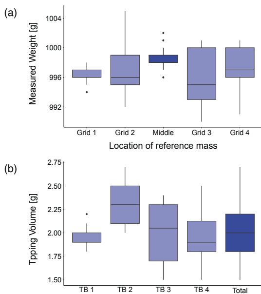
Figure 3: (a) Weighing precision of load cells, depending on the location of the reference mass (1000 g) in the container and (b) tipping volume of four single tipping buckets below one lysimeter.
