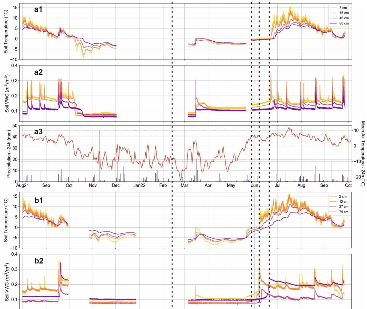
315 Figure 4: Point sensor data from Sites 1 and 2 showing soil temperature (a1, b1) and soil VWC (a2, b2) between Aug 2021 and Oct 2022, together with air temperature and precipitation (a3) recorded by the Ny-Ålesund weather station (Seklima, 2023). Dotted lines mark the four ERT timesteps shown in Fig. 1.
