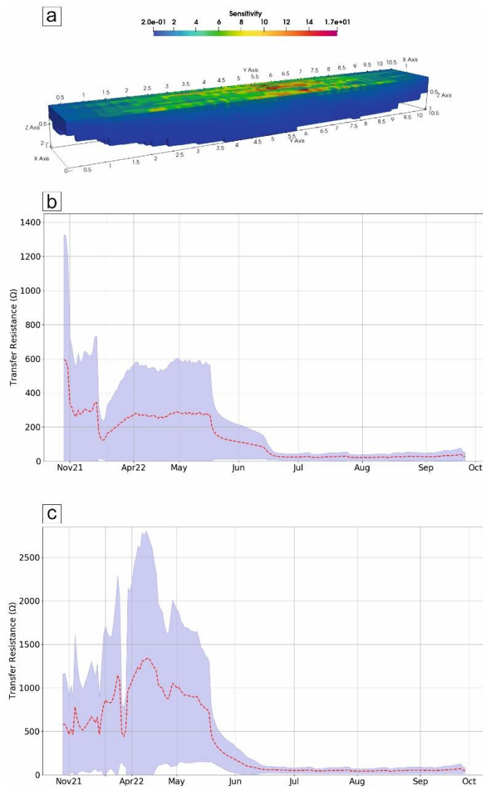
280 Figure 2: (a) 3D Sensitivity plot corresponding to the measurement sequence used at both sites. Evolution of transfer resistance ( \Omega ) at (b) Site 1 and (c) Site 2. Red dotted line represents the mean transfer resistance, and the shaded purple area represents the transfer resistance data distribution within one standard deviation.
