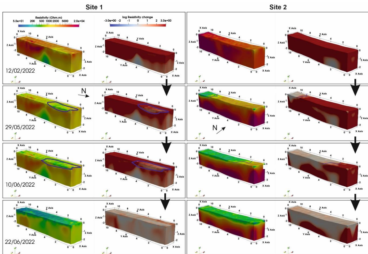
300 Figure 3: Inversion results for four selected ERT timesteps. A 3D model of absolute electrical resistivity values is shown on the left-hand side of the subplots and resistivity change relative to ERT data recorded on 2 nd Aug 2021 on the right-hand side. Axes are in metres. Purple line delineates zones of interest where changes in resistivity are detected.
