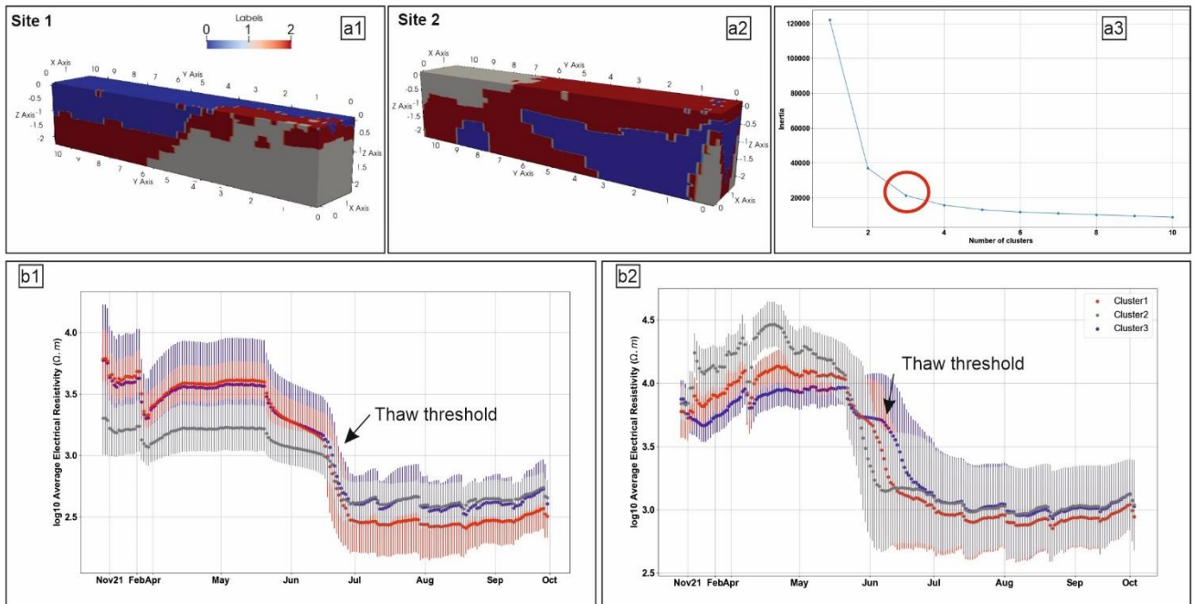
450 Figure 12: Spatial cluster division of ERT model cells in reference to their CV value corresponding to (a1) Site 1 and (a2) Site 2. (a3) Results of the elbow method with the chosen number of clusters highlighted by the red circle. Average resistivity and standard deviation values recorded between November 2021 and October 2022 corresponding to (b1) Site 1 and (b2) Site 2 clusters.
