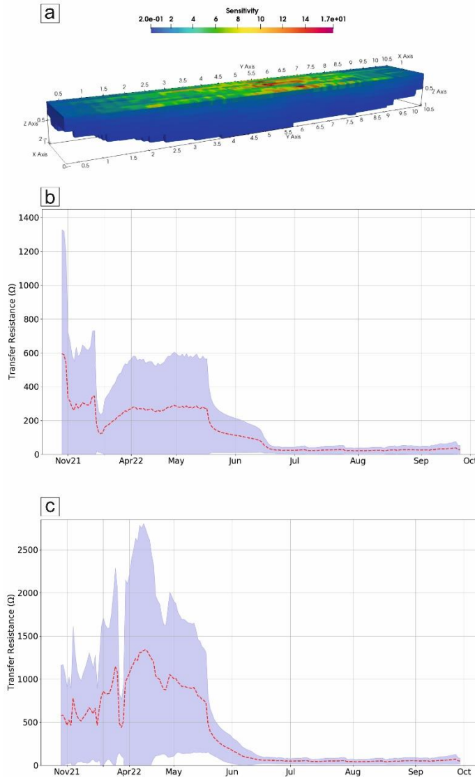
275 Figure 2: (a) 3D Sensitivity plot corresponding to the measurement sequence used at both sites. Evolution of transfer resistance ( \Omega ) at (b) Site 1 and (c) Site 2. Red dotted line represents the mean transfer resistance, and the shaded purple area represents the transfer resistance data distribution within one standard deviation.
