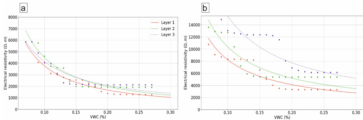
370 Figure 8: Best fit of Archie's law (curves) to in-situ measurements of electrical resistivity and soil VWC (dots). (a) Site 1 layers 1-3, (b) Site 2 layers 1-3.
