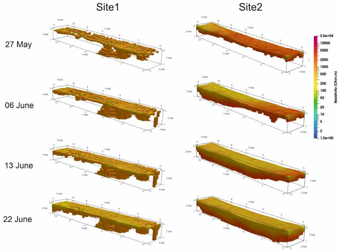
415 Figure 9: Four selected ERT timesteps showing only model cells with resistivities below the site-specific thaw threshold values.
