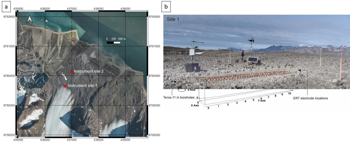
175 Figure 1: (a) Topographic map of the study area (© NPI, 2023) (b) Photograph of Site 1 showing the instrumental set-up and the corresponding schematics of the underground sensor installation and the ERT investigation volume (axes units are metres).
