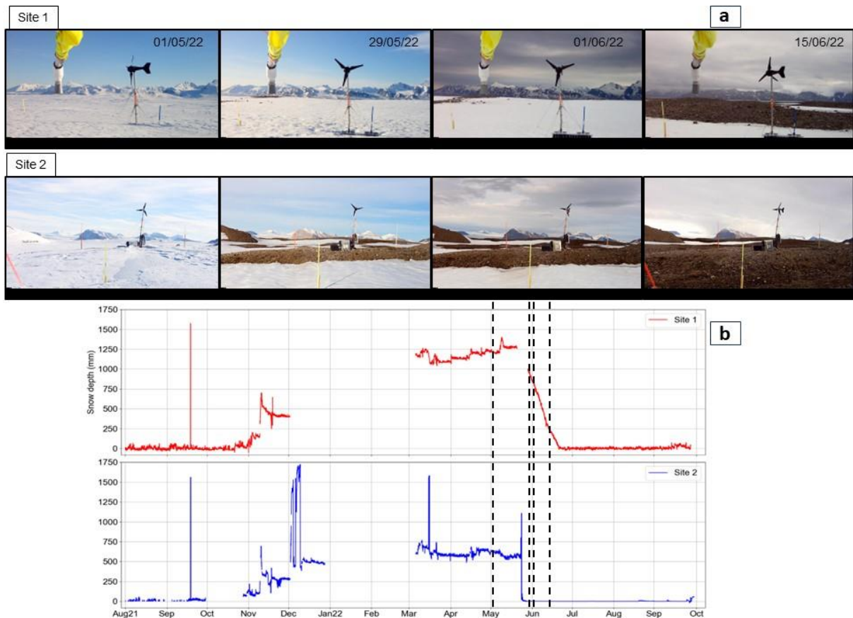
335 Figure 6: (a) Nature camera photographs of the two sites. (b) Snow depth measurements corresponding to Sites 1 and 2. Dotted lines in B indicate the dates the photographs were taken.
