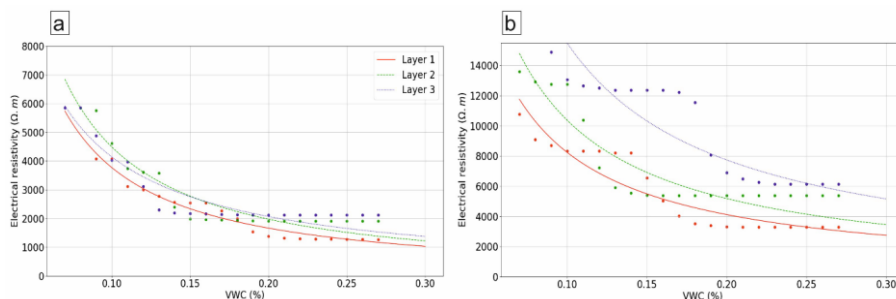
Figure 8: Best fit of Archie's law (curves) to in-situ measurements of electrical resistivity and soil VWC (dots). (a) Site 1 layers 1-3, (b) Site 2 layers 1-3.
