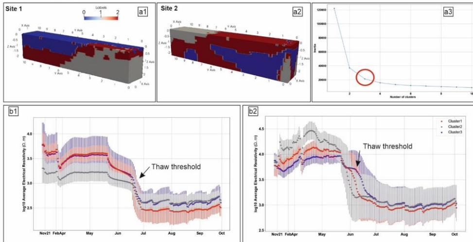
470 Figure 12: Spatial cluster division of ERT model cells in reference to their CV value corresponding to (a1) Site 1 and (a2) Site 2. (a3) Results of the elbow method with the chosen number of clusters highlighted by the red circle. Average resistivity and standard deviation values recorded between November 2021 and October 2022 corresponding to (b1) Site 1 and (b2) Site 2 clusters.
