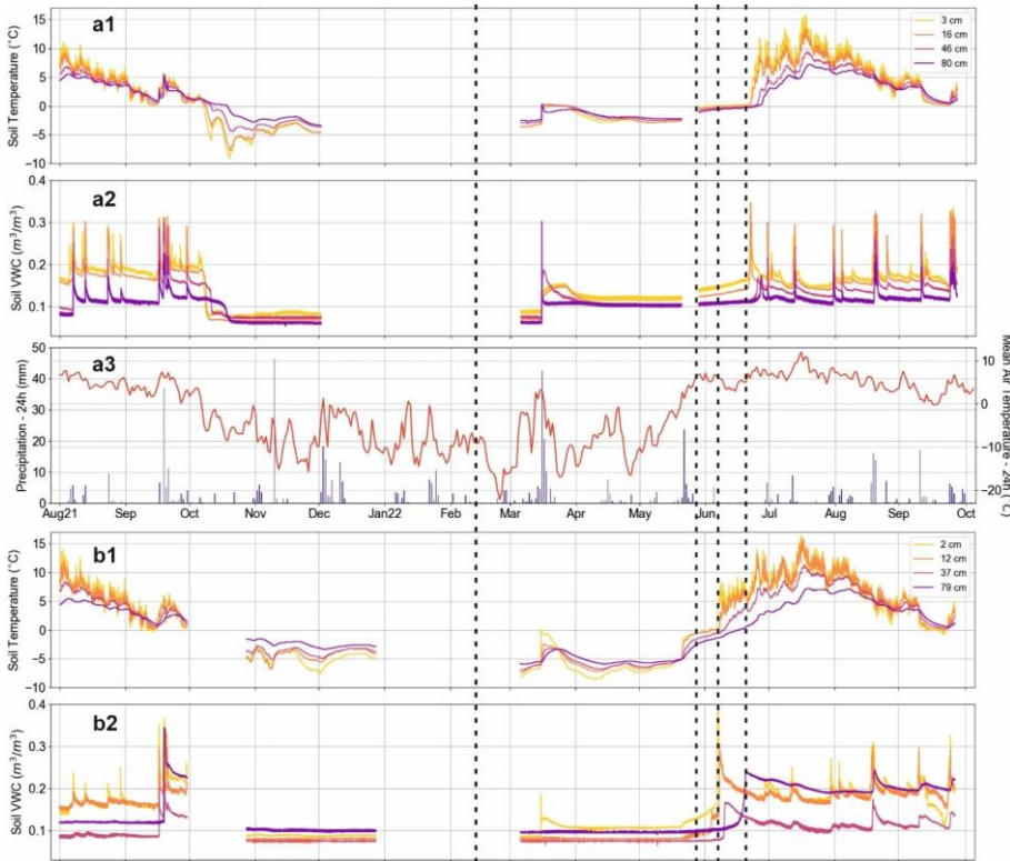
335 Figure 4: Point sensor data from Sites 1 and 2 showing soil temperature (a1, b1) and soil VWC (a2, b2) between Aug 2021 and Oct 2022, together with air temperature and precipitation (a3) recorded by the Ny-Ålesund weather station (Seklima, 2023). Dotted lines mark the four ERT timesteps shown in Fig. 1.
