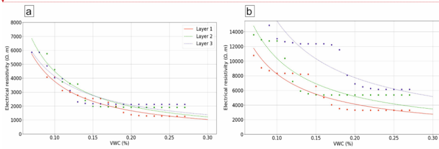
Figure 8: Best fit of Archie's law (curves) to in-situ measurements of electrical resistivity and soil VWC (dots). (a) Site 1 layers 1-3, (b) Site 2 layers 1-3.
