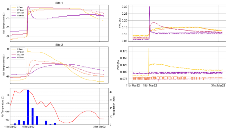
355 Figure 5: Soil temperature and soil VWC at Sites 1 and 2 during the mid-March thaw event, shown together with corresponding air temperature (red line) and precipitation (blue bars) records (Seklina, 2023).
