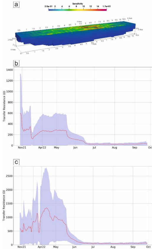
295 Figure 2: (a) 3D Sensitivity plot corresponding to the measurement sequence used at both sites. Evolution of transfer resistance ( \Omega ) at (b) Site 1 and (c) Site 2. Red dotted line represents the mean transfer resistance, and the shaded purple area represents the transfer resistance data distribution within one standard deviation.
