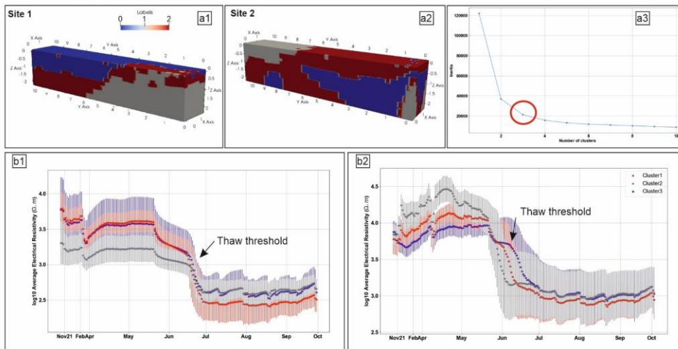
Figure 12: Spatial cluster division of ERT model cells in reference to their CV value corresponding to (a1) Site 1 and (a2) Site 2. (a3) Results of the elbow method with the chosen number of clusters highlighted by the red circle. Average resistivity and standard deviation values recorded between November 2021 and October 2022 corresponding to (b1) Site 1 and (b2) Site 2 clusters.
