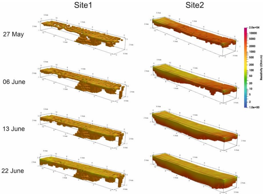
Figure 9: Four selected ERT timesteps showing only model cells with resistivities below the site-specific thaw
