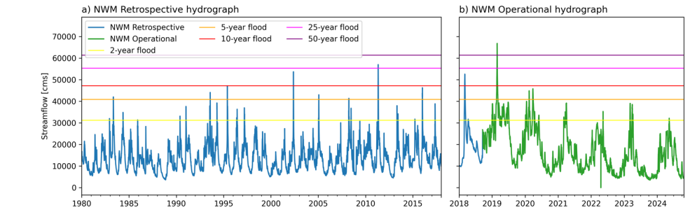
350 Figure 3: Streamflow hydrograph from the National Water Model (NWM) for the representative reach showing (a) retrospective simulations from 1980-2017 and (b) operational simulations from the analysis Assim run from 2018-2024. Horizontal lines indicate the 2-, 5-, 10-, 25-, and 50-year flood recurrence interval discharge values for the stream reach.
