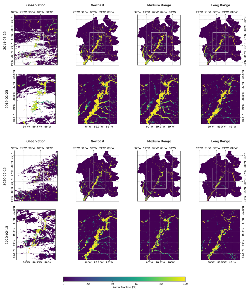
Figure 6. Comparison of observed and FIER-predicted water fraction maps for the two selected flood events: 2019-02-25, the 50-year flood (top two rows), and 2020-02-15, the 50-year flood (bottom two rows) The lower rows are a zoomed view for the baseline area to highlight local differences in the predictions. Predictions use the nowcast, medium-range (7-day lead time) and long-range (15-day lead time) streamflow from the NWM. White areas are missing data due to clouds, cloud shadows and other poor-quality data.
