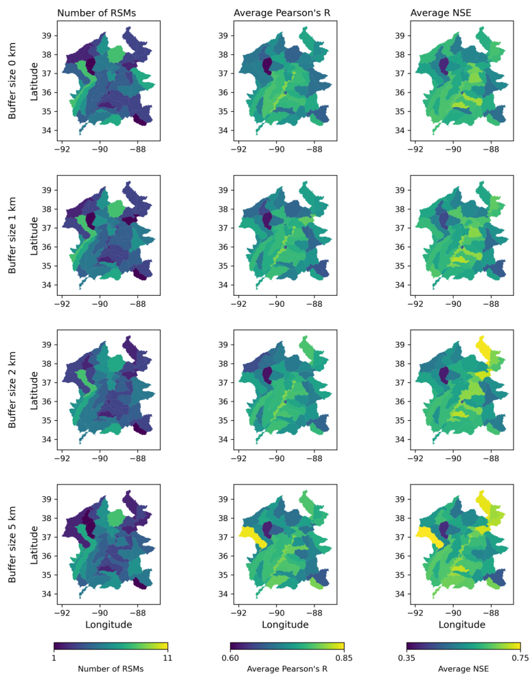
855 Figure A2: Spatial distribution of FIER model performance metrics for varying buffer sizes. The figure displays maps showing (left) the number of significant RSMs identified by the Monte Carlo test, (middle) the average Pearson's correlation coefficient between the RTPCs and streamflow, and (right) the average Nash-Sutcliffe Efficiency (NSE) of the fitted regression models for each watershed, across different buffer sizes (0 km, 1 km, 2 km, 5 km).
