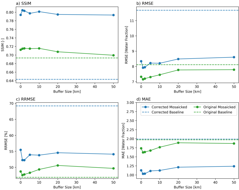
Figure 4: Graphs illustrating the impact of varying buffer sizes on the performance of the FIER method for flood inundation mapping, assessed using the areal average of four different metrics: (a) Structural Similarity Index Measure (SSIM), (b) Root Mean Squared Error (RMSE), (c) Relative Root Mean Squared Error (RRMSE), and (d) Absolute Error. The green lines represent the original FIER outputs, while the blue lines depict the corrected outputs after applying a CDF matching post-processing step. The dashed lines indicate the baseline performance metrics obtained from applying FIER to a single, larger AOI.
