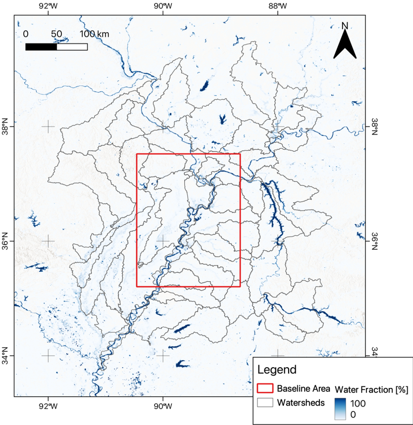
205 Figure 2: Study area map showing the average surface water fraction derived from the VIIRS sensor from 2012-2020 along with two subregions, the baseline region for FIER in red and the surrounding watersheds in black.
