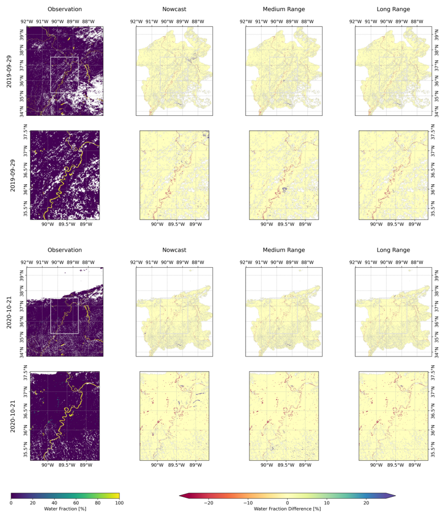
870 Figure B2: Same as Fig. B1 except for the two selected low-flow dates: (top two rows) 2019-09-29 and (bottom two rows) 2020-10-21. To be used as comparison with Fig. 7
