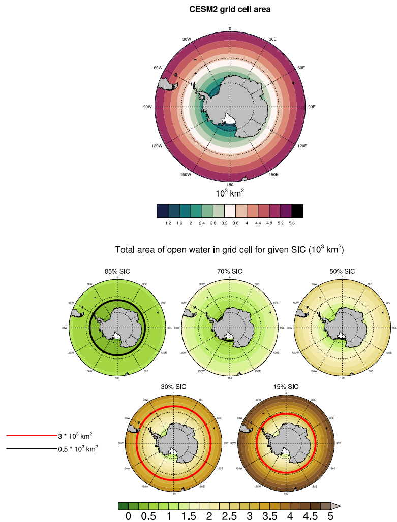
740 Figure B1. Area of the ocean grid cells in the CESM2 ( \times 10^3 \text{ km}^2 ; top) and total area ( \times 10^3 \text{ km}^2 ) of open water for a given SIC threshold in the CESM2 grid (bottom). Red/black contours indicate 3 \times 10^3 \text{ km}^2 / 0.5 \times 10^3 \text{ km}^2 of open water, respectively.
