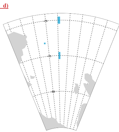
Figure B2. Sea ice concentration required to result in 312.5 km 2 of open water within a grid cell: a) SIC 50% on a 25 km x 25 km equal area grid cell, b) 94.8% SIC on a 1°x1° lat/lon grid cell at 70°S (approximately 111km x 51km), and c) 93.7% SIC on a 1°x1° lat/lon grid cell at 75°S (approximately 111km x 44.4km). Panel d shows the area occupied by grid cells (in blue) in a, b, c in the Ross Sea as an illustration. Panels a-c are shown as rectangles for illustration even though 1° lat/lon grid cells are not exactly rectangular.
