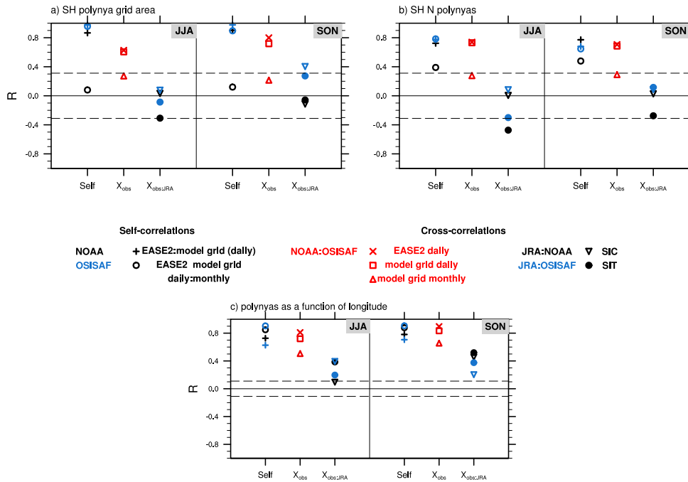
Figure 5. Correlation coefficients for integrated SH polynya areas (a), number of polynyas (b) and polynyas as a function of longitude (c) for each JJA (left) and SON (right). Self-correlations are calculated between different grids (“regridding”) for same observational product (NOAA black; OSISAF, blue); cross-correlations between the two observational products (NOAA:OSISAF, red) and between the observational products and the JRA-CESM (obs:JRA; NOAA black; OSISAF, blue). Symbols show correlations between time/longitude polynya time series from the daily observational data on the original EASE grid vs daily (+) and monthly (o) regridded on the model grid; NOAA:OSISAF on the EASE grid (x) and then regridded daily (□) and monthly (open triangles); and between JRA-CESM polynyas identified using SIT 0.4 m (*) and SIC 85% metric (inverted open triangles). Dashed horizontal lines in a-c indicate the 95% significance level based on the Mann-Kendall non-parametric trends significance (Mann 1945; Kendall 1975; and Gilbert 1987).
