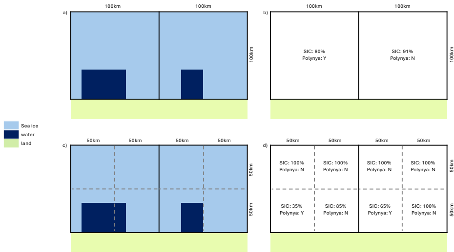
760 Figure B3. Examples of grid cells classified as polynyas using an 80% SIC threshold on a larger resolution grid (a-b) and a smaller resolution grid (c-d). Coloured panels (a, c) indicate areas of ice (light blue), water (navy) and land (light green). Text in panels b, d indicate SIC for the grid cell and whether or not it would be identified as a polynya using an 80% SIC threshold. The top example has one polynya grid cell and double the integrated polynya area (10000 km 2 ) over the entire region compared to the second example (2 grid cells and 5000 km 2 ).
