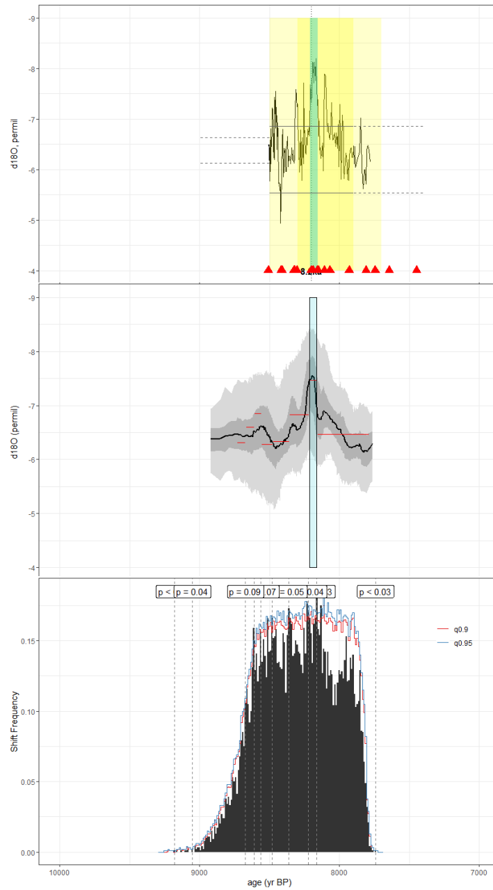
1240 Figure C5. As in Fig. C1, but for the speleothem record of Cheng et al., 2009 (PAD07). The original age modeling method used in the construction of the published time series is unknown. Here, we present an age ensemble using the BACON algorithm provided by geoChronR.
