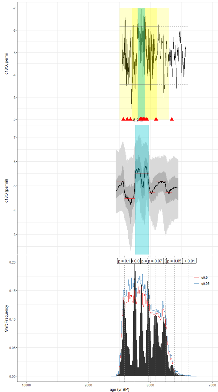
Figure C1. A stackplot from the speleothem record of Duan et al., 2021 (ABC1). The top panel shows the raw oxygen isotope time series with 7.9 ka-8.3 ka highlighted in darker yellow and 7.7 ka-8.5 ka highlighted in lighter yellow, with the ages of radiometric dates represented by red triangles (see schematic in Fig. B1 for more information). The middle panel shows the same time series with age and
