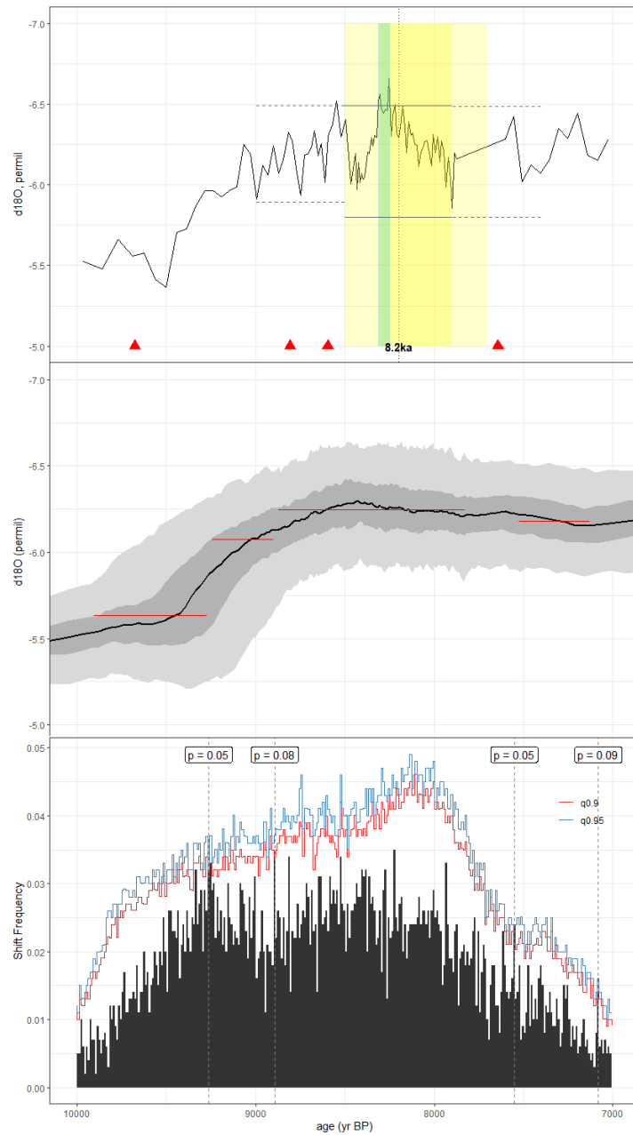
1390 Figure C40. As in Fig. C1, but for the speleothem record of Winter et al., 2020 (GURM1). The published age model was constructed using the copRa algorithm, while we use the BACON ensemble produced for SISALv2 here.
