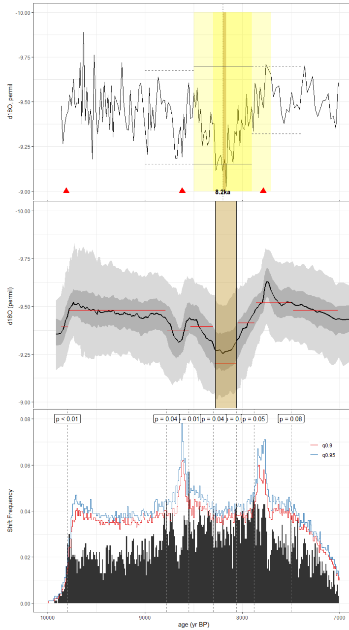
Figure C14. As in Fig. C1, but for the speleothem record of Jiang et al., 2012 (SG1). The published age model was constructed by linear interpolation between U/Th dates. Here, we leverage the BACON ensemble from SISALv2 for our analyses.
