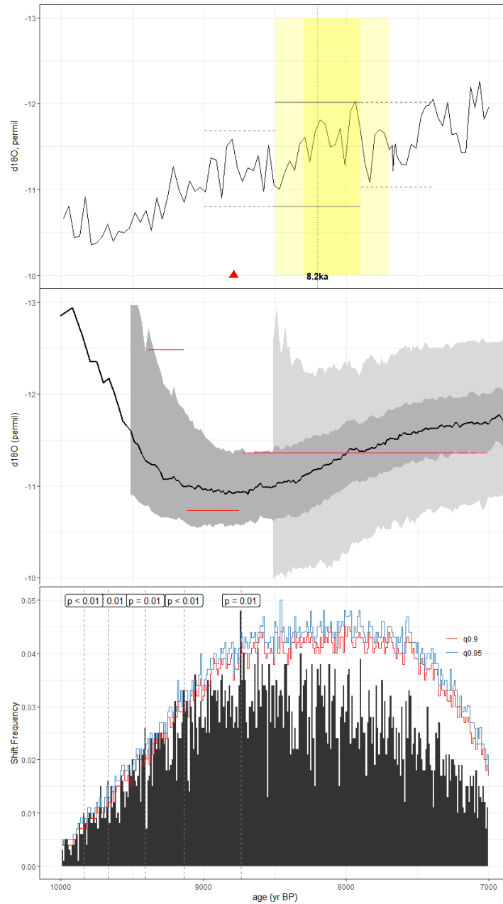
Figure C26. As in Fig. C1, but for the lacustrine sediment record of Bird et al., 2011 (LP). The published age model was created using CALIB 5.0 with an unreported calibration curve. Here, we construct our age ensemble in geoChronR using the BACON algorithm and SHCal20.
