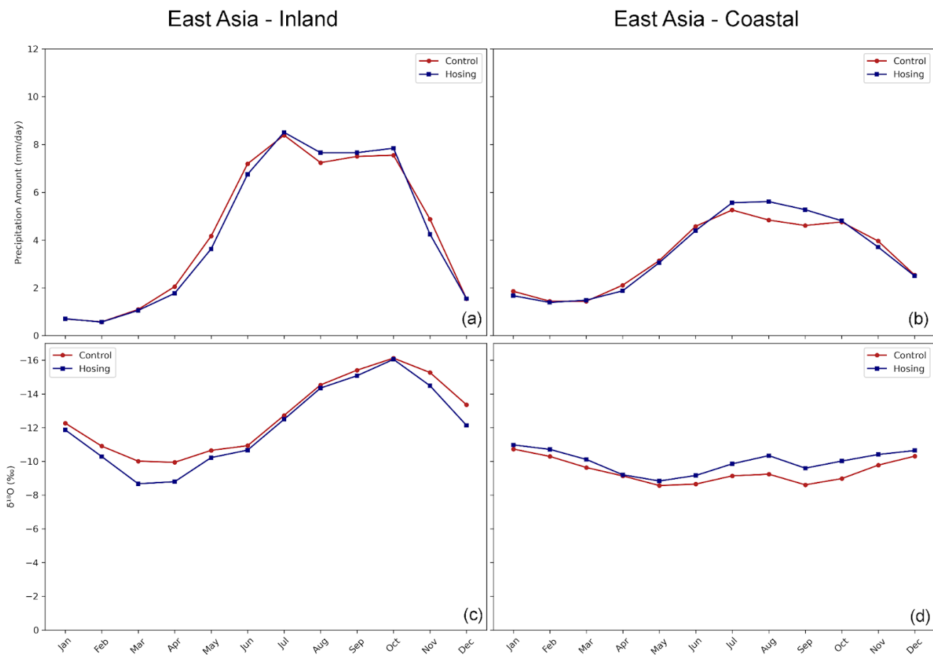
Figure 12. The monthly climatology of the area-weighted precipitation amount (top row) and \delta^{18}O_p (bottom row) for the “ctrl” (red) and “hose” (blue) simulations for East Asia. Data from the western (inland) subregion defined by the positive \Delta\delta^{18}O_p anomaly in Fig. 10a are plotted in the left column. Data from the eastern (coastal) subregion defined by the negative \Delta\delta^{18}O_p anomaly are plotted on the right.
