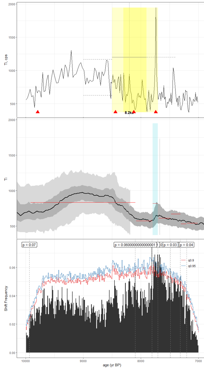
Figure C53. As in Fig. C1, but for the lake sediment titanium content record of Woods et al., 2020 (PLJUN15). The published age model was created using the BACON algorithm with IntCal13 calibration curve. Here, we reconstruct a BACON ensemble using the IntCal20 curve in geoChronR.
