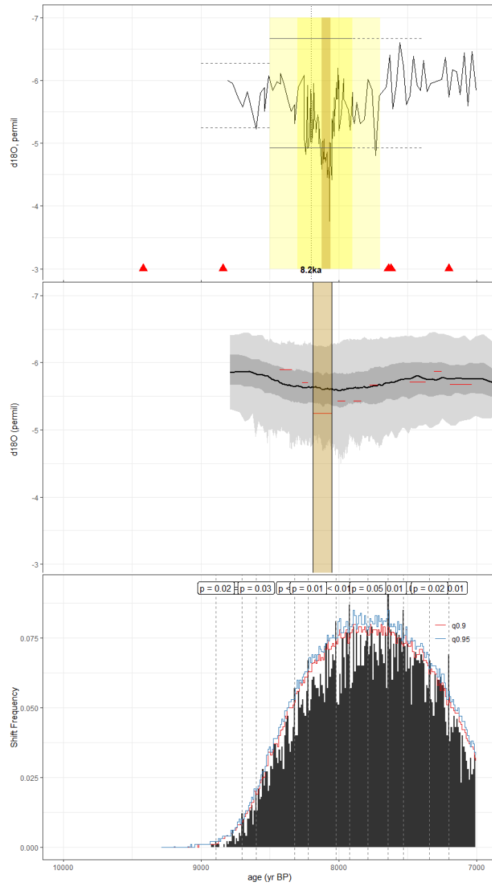
1290 Figure C17. As in Fig. C1, but for the speleothem record of Lachniet et al., 2004 (V1). The published time series was aligned to a fifth-order polynomial best-fit age model between isochron dates. We employ the BACON ensemble provided by SISALv2 for our analyses.
