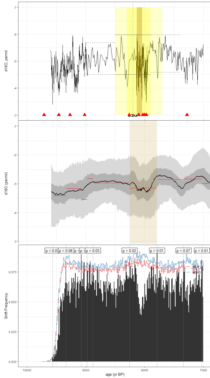
Figure C10. As in Fig. C1, but for the speleothem record of Neff et al., 2001 (H5). While the method used in the construction of the published time series was unreported, we leveraged the SISALv2 BACON ensemble for our analyses.
