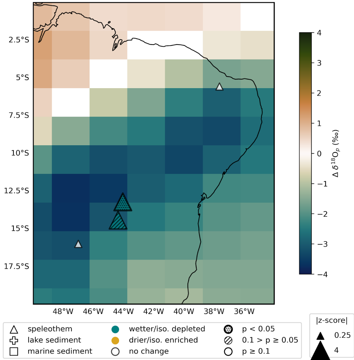
1020 Figure 6. As in Fig. 5, but for IPCC region 11: northeastern South America (box). Model shading represents the precipitation amount-weighted \delta^{18}\text{O} anomaly between the last 50 years of the “hose” and “ctrl” simulations.
