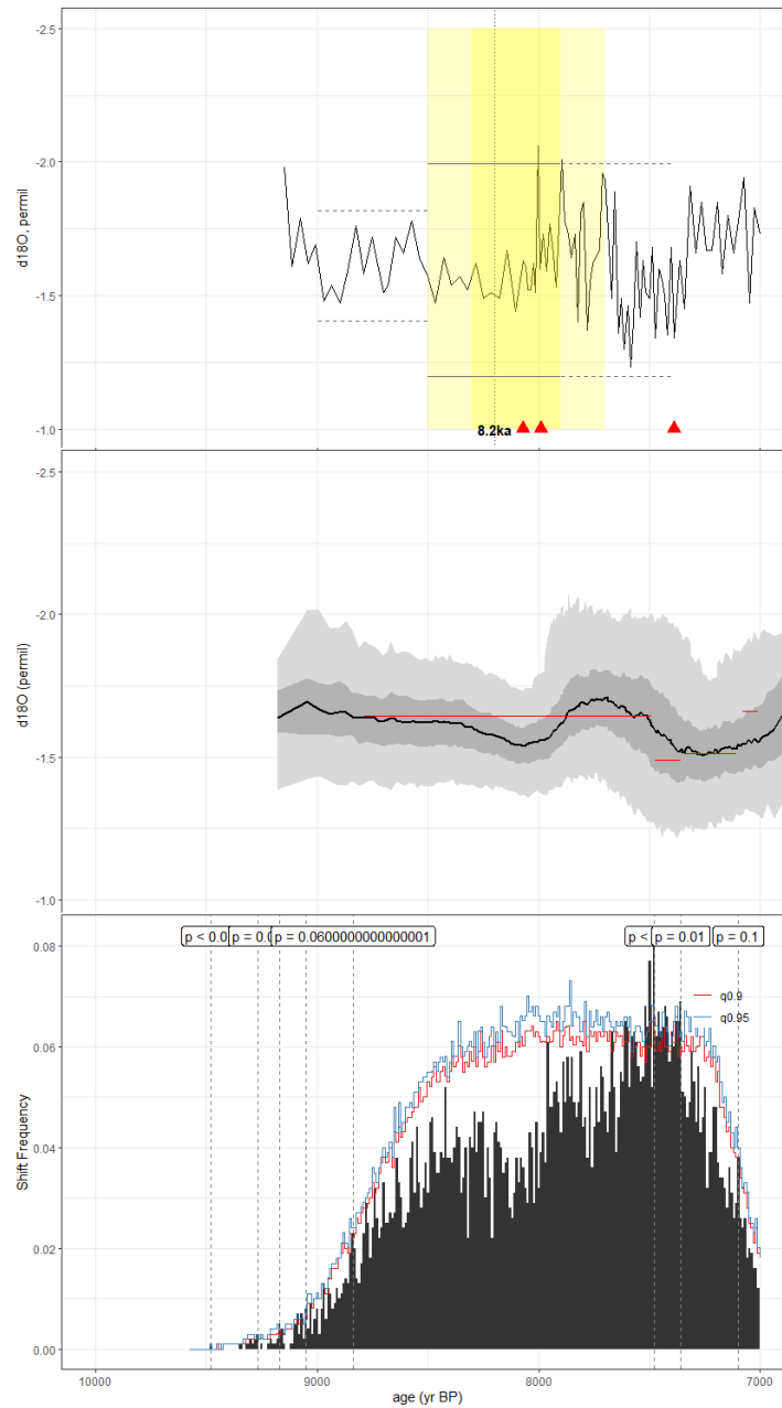
Figure C22. As in Fig. C1, but for the foraminifera record of Schmidt et al., 2012 (JPC51). The published age model was created using CALIB 6.0, with a standard -400-year reservoir age correction for surface waters. Here, we use the BACON algorithm included in geoChronR to produce our age ensemble.
