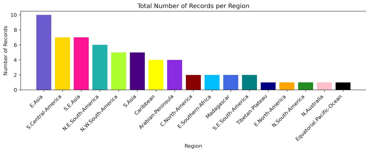
1165 Figure B2. Locations of proxy records within climate reference regions defined in Iturbide et al. (2020).
