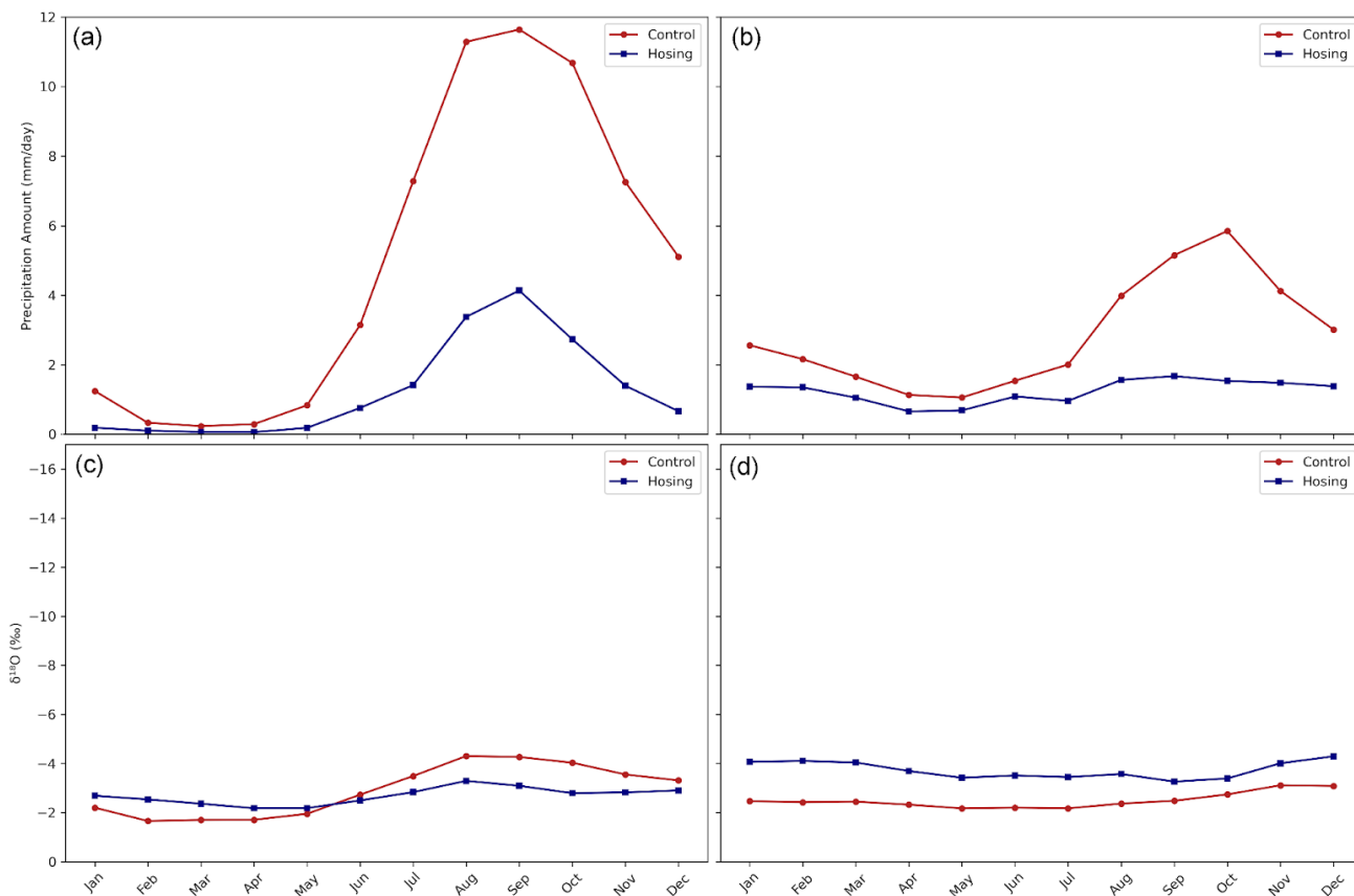
1080 Figure 13. As in Fig. 12, but for Southern Central America. Data from the southern subregion (northeastern tropical Pacific) defined by the positive \Delta\delta^{18}\text{O}_p anomaly in Fig. 10g are plotted in the left column, while data from the northern subregion (Caribbean) defined by the negative \Delta\delta^{18}\text{O}_p anomaly in Fig. 10g are plotted in the right column.
