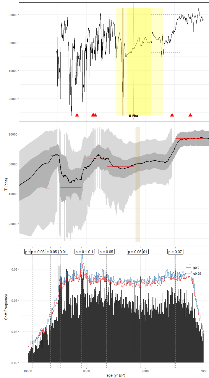
1245 Figure C6. As in Fig. C1, but for the lacustrine titanium content record of Duarte et al., 2021 (Core5LI). The published age model was constructed using BACON using the IntCal20 calibration curve, and here, we construct our age ensemble using the BACON algorithm included with geoChronR.
