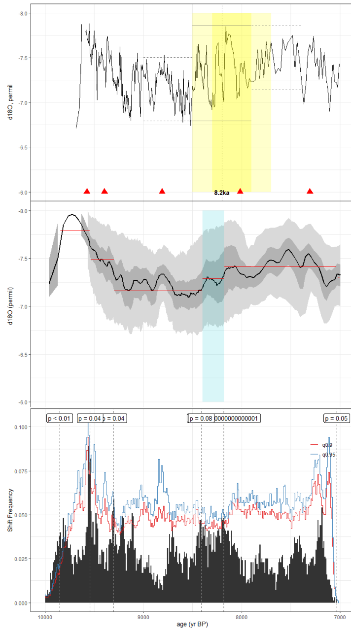
Figure C48. As in Fig. C1, but for the speleothem record of Lechleitner et al., 2017 (MAW6). The published age model was constructed using copRa. Here, we employed the Bchron ensemble included in SISALv2.
