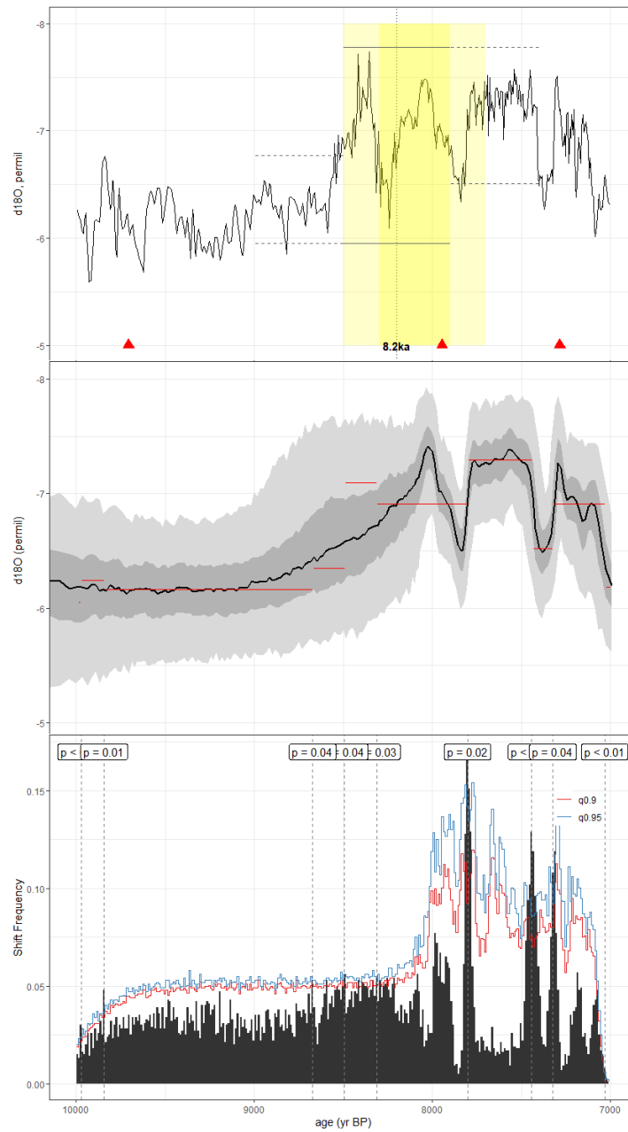
Figure C23. As in Fig. C1, but for the speleothem record of Berkelhammer et al., 2012 (KMA). The published age model was created using the StalAge algorithm. Here, we used the BACON age ensemble included in SISALv2.
