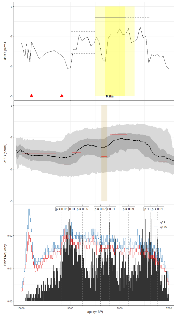
1430 Figure C49. As in Fig. C1, but for the speleothem record of Dutt et al., 2015 (MWS1). The published age model was created using the StalAge algorithm. Here, we use the Bchron ensemble from SISALv2.
