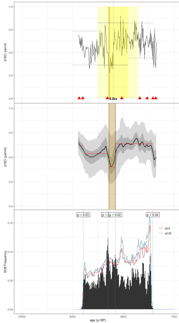
Figure C16. As in Fig. C1, but for the speleothem record of Chawchai et al., 2021 (TK20). The published age model was constructed using the BACON algorithm. Here, we used the BACON age ensemble supplied in the SISALv2 database.
