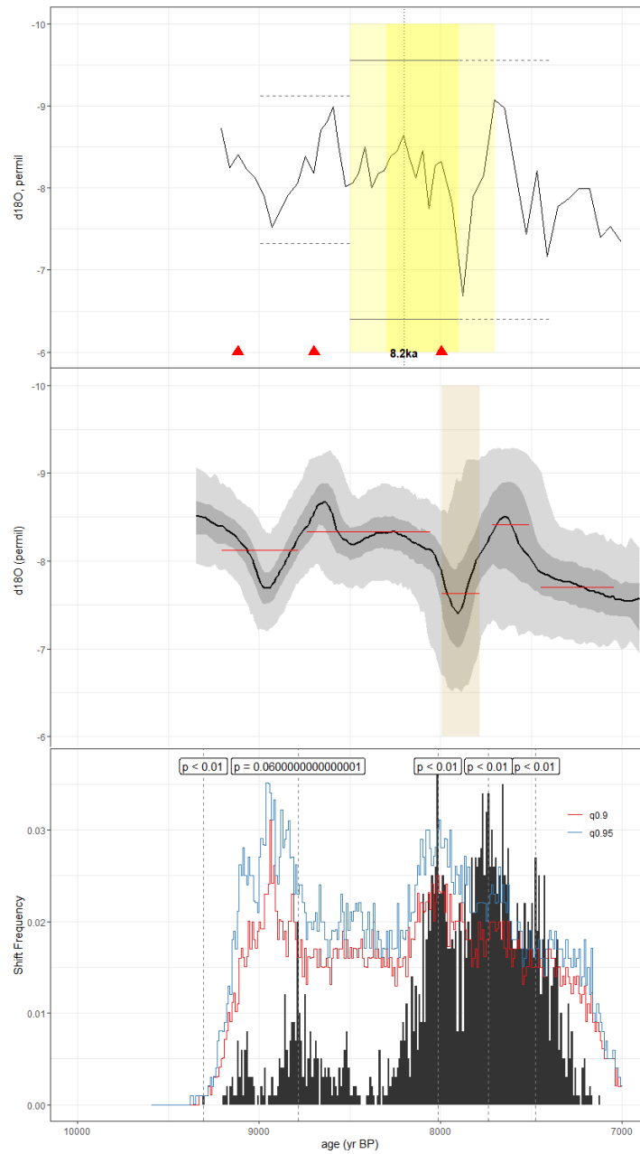
Figure C32. As in Fig. C1, but for the speleothem record of Bernal et al., 2016 (BTV21a). Information about the published age model was 1355 unreported. Here, we use the SISALv2 BACON age ensemble.
