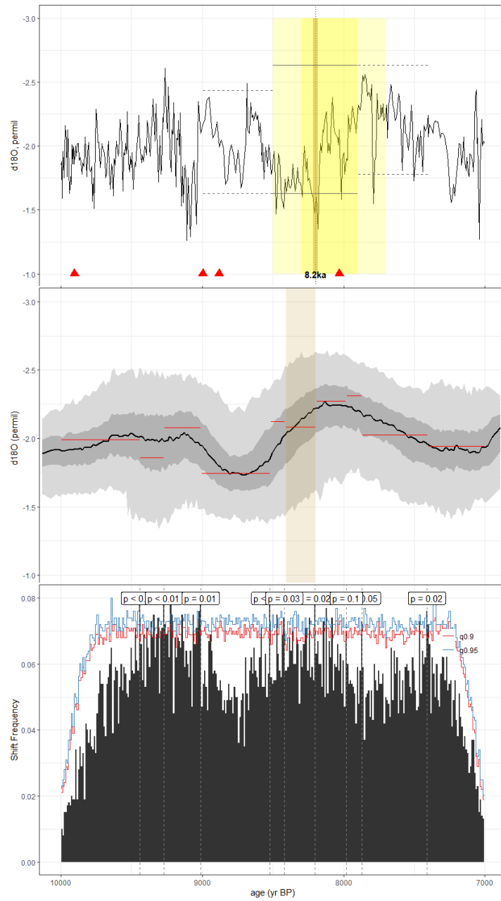
Figure C13. As in Fig. C1, but for the speleothem record of Fleitmann et al., 2007 (Q52007). The published age model was created via a polynomial fit to the age-depth curve of the Th–U data. Our age ensemble leverages the BACON algorithm included in geoChronR.
