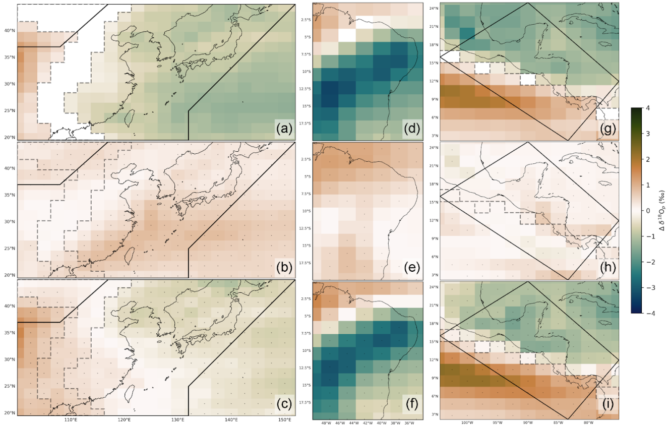
Figure 10. As in Fig. 9, but for East Asia (left column; a,b,c), northeast South America (middle column; d,e,f), and southern Central 1055 America (right column; g,h,i). The panels in the upper row show the annual amount-weighted \delta^{18}\text{O}_p anomaly of each region, as plotted in Fig. 4a. The panels in the middle and bottom rows depict the same data as in Fig. 9a and b, respectively, at the regional level. The unfilled black polygons (exterior) represent the boundaries of each region defined by the IPCC. The grey dotted lines subdivide East Asia and southern Central America into E-W and N-S subregions defined by the distinct \pm\Delta\delta^{18}\text{O}_p dipoles shown in panels a and g, respectively.
