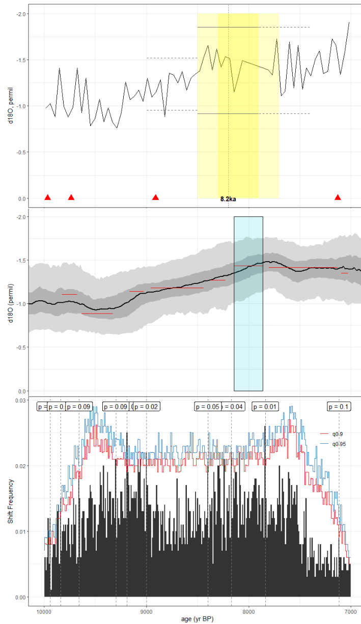
Figure C39. As in Fig. C1, but for the foraminifera record of Thirumulai et al., 2021 (GB2GC1). The published age model was developed using the BACON algorithm and Marine13 calibration curve, which we reconstructed using geoChronR.
