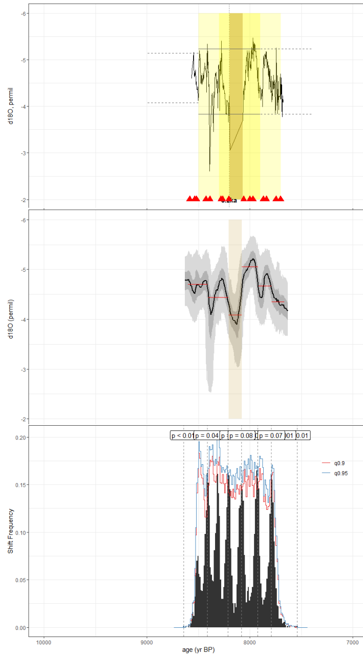
Figure C9. As in Fig. C1, but for the speleothem record of Cheng et al., 2009 (H14). The age modeling algorithm used to construct the original age model was unreported. Here, we constructed our age ensemble using BACON in geoChronR.
