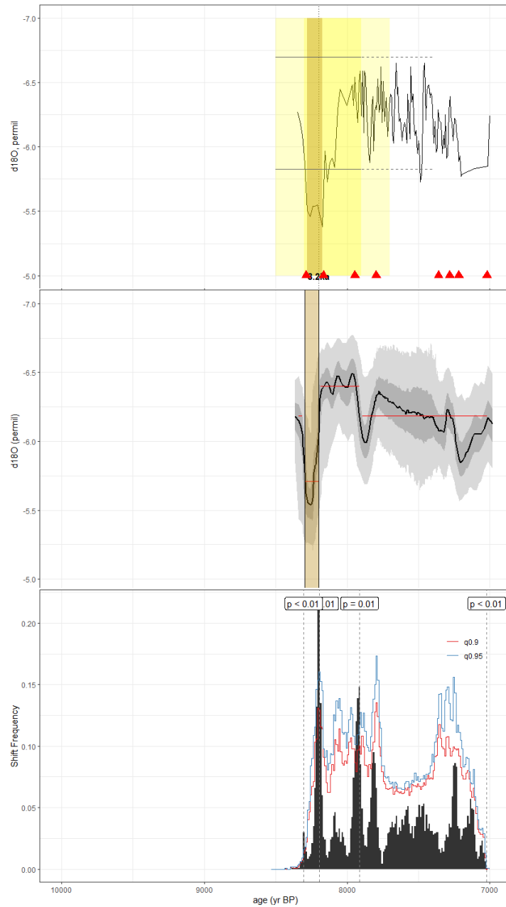
Figure C15. As in Fig. C1, but for the speleothem record of Chawchai et al., 2021 (TK07). The published age model was constructed using the BACON algorithm. Here, we used the BACON age ensemble supplied in the SISALv2 database.
