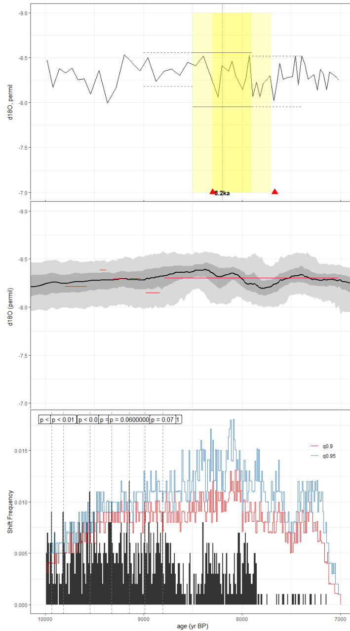
Figure C21. As in Fig. C1, but for the speleothem record of Li et al., 2011 (FR5). The age modeling algorithm used to construct the original age model was unreported, but leveraged the IntCal09 calibration curve. Here, we use the copRa age ensemble included in SISALv2.
