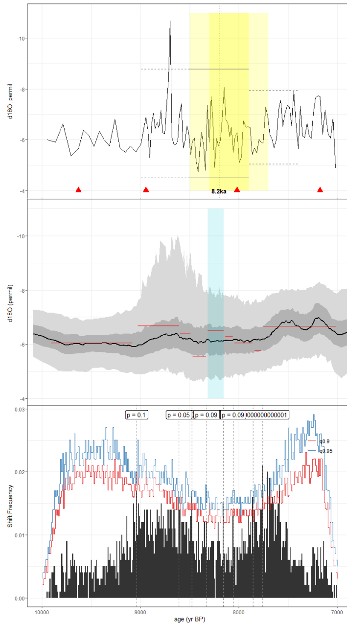
1460 Figure C55. As in Fig. C1, but for the speleothem record of Cruz et al., 2009 (RN4). The method used in the construction of the published age model was unreported, but we leverage the Behron ensemble supplied in version 2 of the SISAL database for our analyses.
