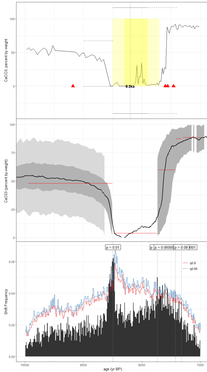
Figure C25. As in Fig. C1, but for the lake sediment record of Hodell et al., 1995 (LC1). The published age model was created using the 1325 decadal tree ring dataset in CALIB. Here, we use BACON with the IntCal20 calibration curve supplied by geoChronR.
