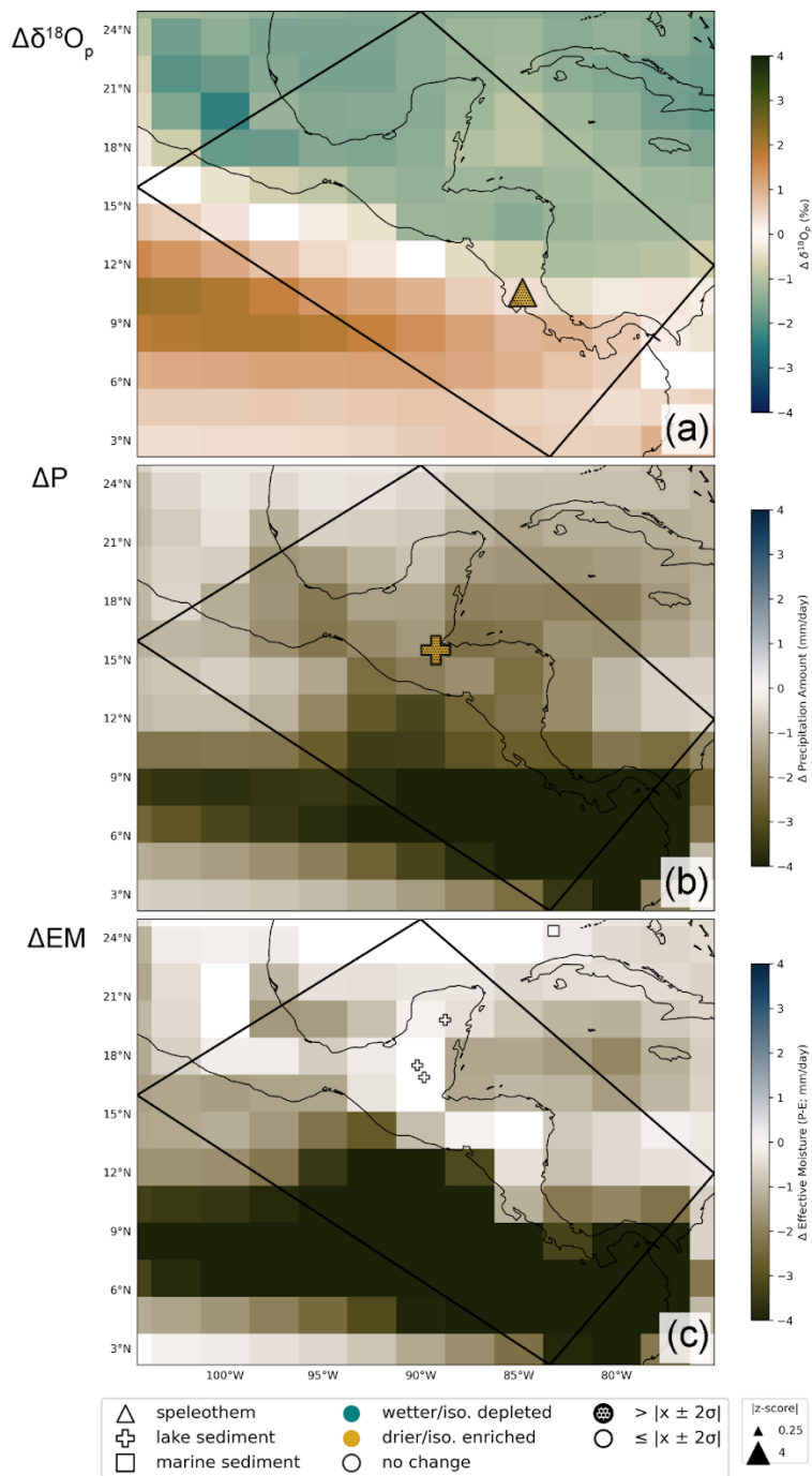
1195 Figure B7. As in Fig. B5, but for IPCC region 7: southern Central America (box), with the addition of (c) the effective moisture (precipitation minus evaporation) anomaly between the last 50 years of the “hose” and “ctrl” simulations.
