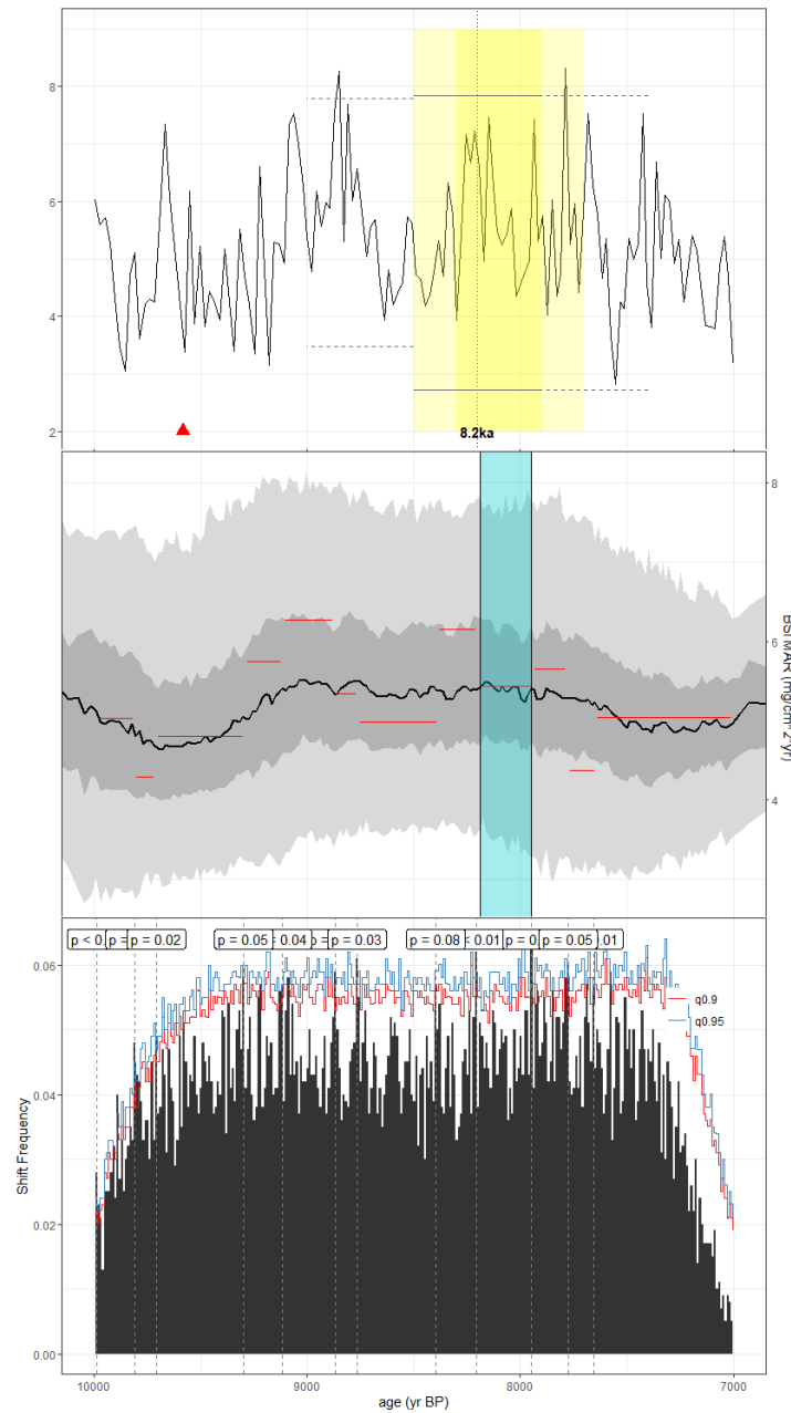
1420 Figure C47. As in Fig. C1, but for the lake sediment BSi MAR record of Johnson et al., 2003 (M981P). CALIB 4.3 was used in the construction of the published age model, with a reservoir age correction of -450 years applied to the radiometric dates. Here, we constructed the age ensemble using the BACON algorithm in geoChronR.
