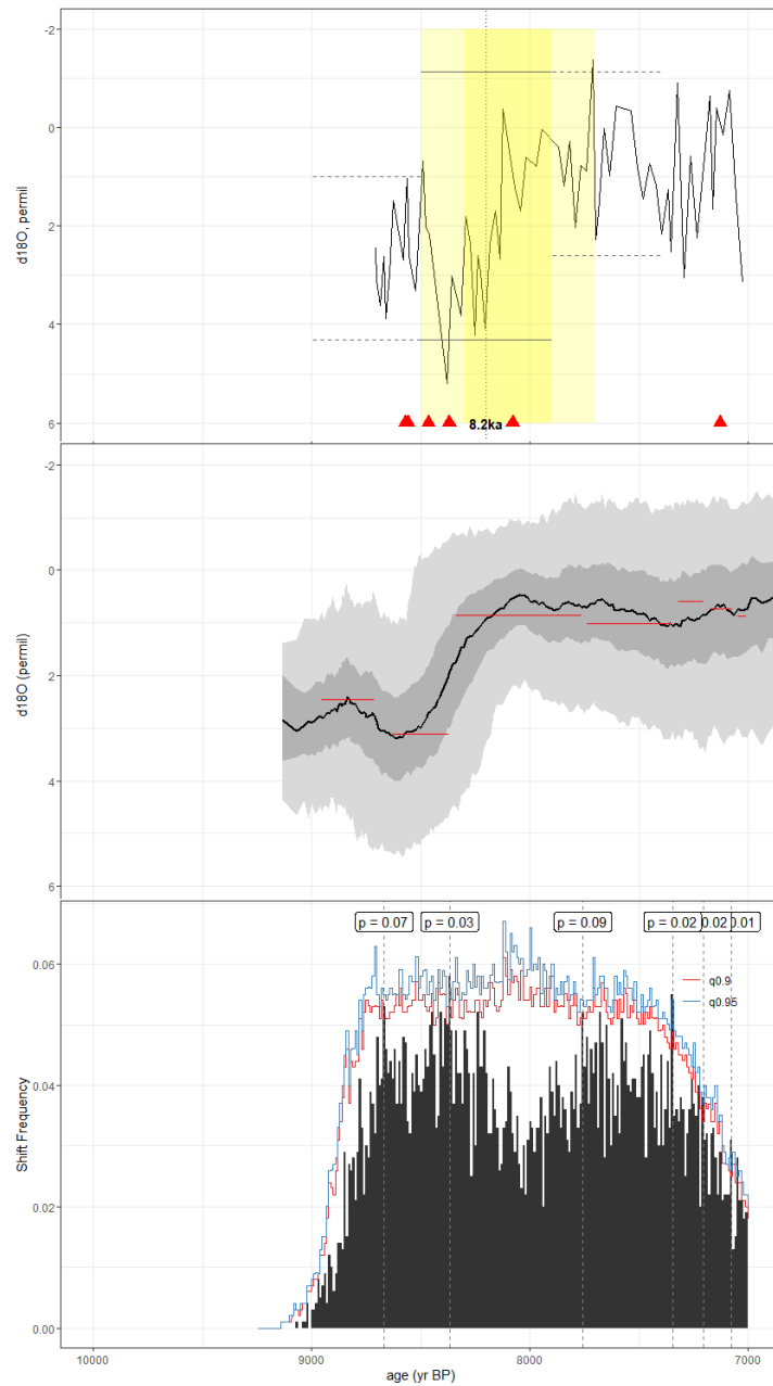
1320 Figure C24. As in Fig. C1, but for the lake sediment \delta^{18}\text{O} record of Wahl et al., 2014 (Lago Puerto Arturo). The published age model was constructed using CLAM 2.2 and the IntCal13 calibration curve. For our analyses, we reconstructed the age model using BACON and IntCal20 in geoChronR.
