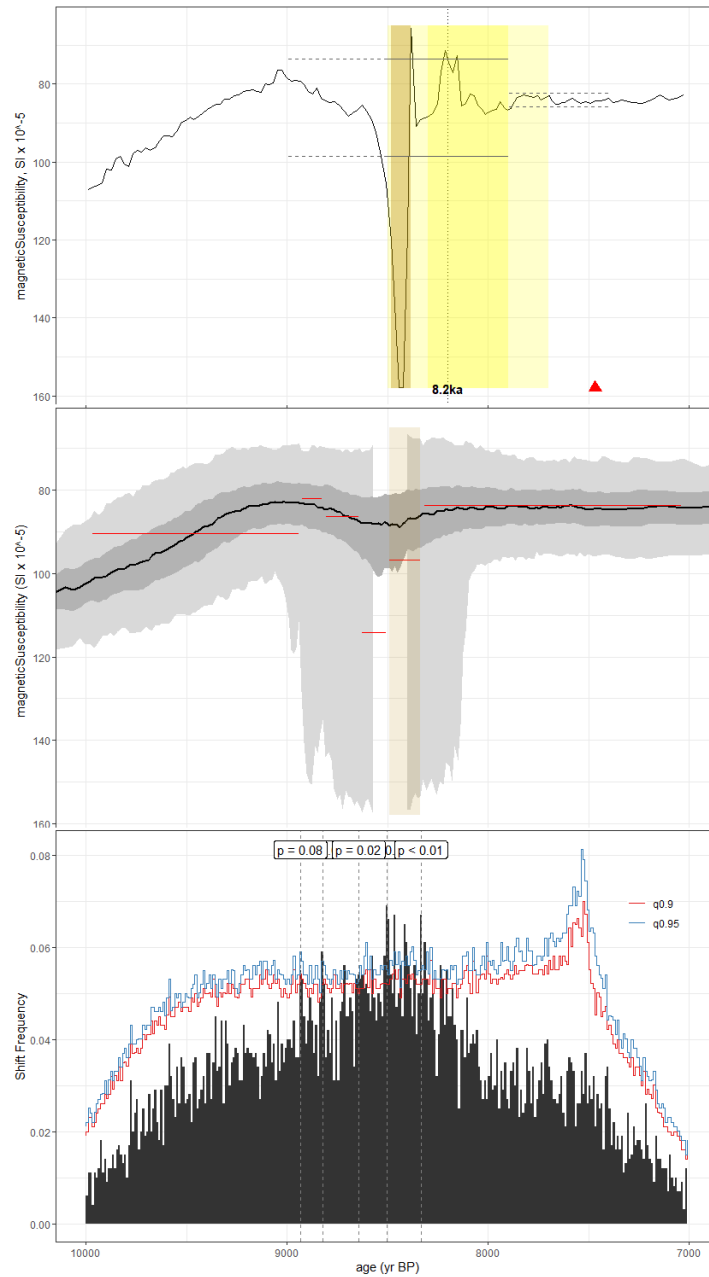
Figure C8. As in Fig. C1, but for the lake sediment magnetic susceptibility record of Hillman et al., 2021 (F14). The original age model was constructed using BACON with the IntCal20 calibration curve. Here, we have reconstructed it using the BACON algorithm in geoChronR.
