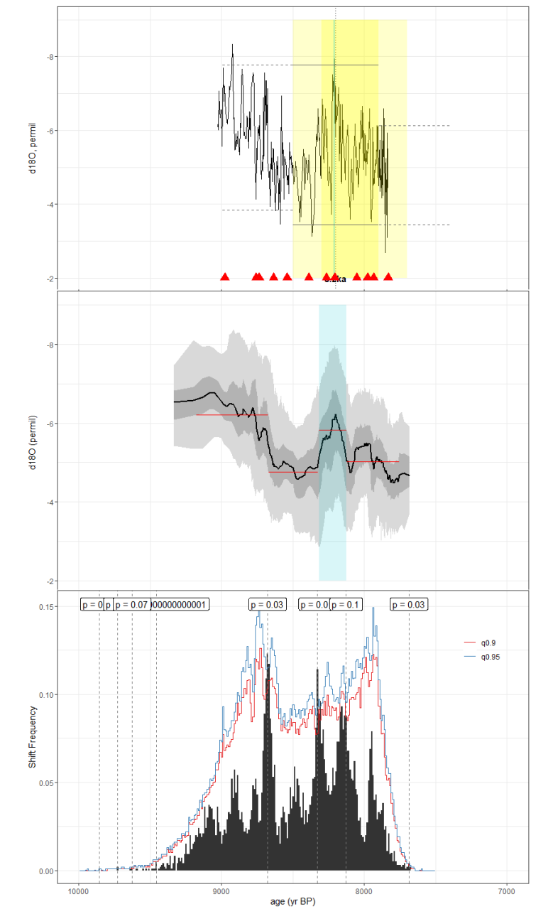
1230 Figure C2. As in Fig. C1, but for the speleothem record of Voarintsoa et al., 2017 (ANJB2). The age model of the original publication was constructed using StalAge. Here, we used the BACON age ensemble from SISALv2.
