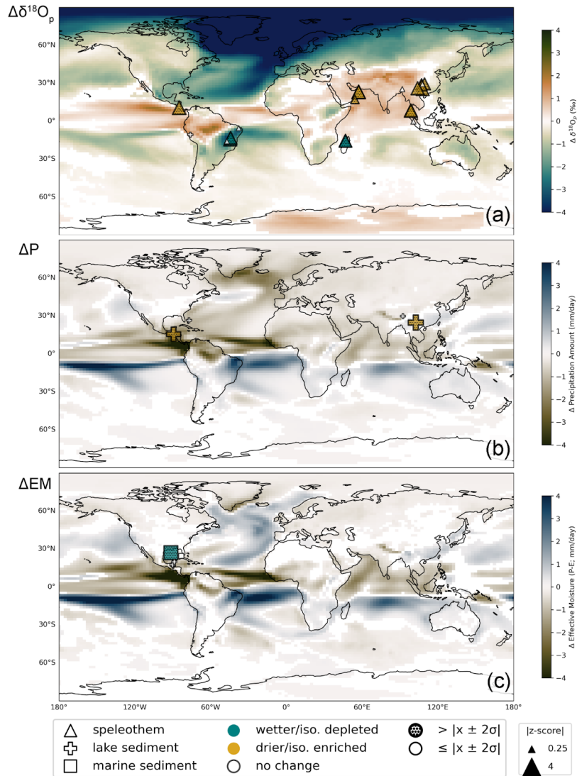
1175 Figure B4. Summary of the 8.2 ka events detected using our modified Morrill et al. (2013) method for the paleoclimate records showing agreement with actR (Fig. 4) in the direction of change. Blue symbols represent wetter (and/or isotopically depleted) conditions while brown symbols represent drier (and/or isotopically enriched) conditions relative to each record's mean climatology over the 7.4 ka-7.9 ka and 8.5 ka-9.0 ka windows described in the text. For records in which no event was detected, symbols are shown in white. The archive type is indicated by the symbol shape, and the symbol size is scaled by 250\ln(1+|z\text{-score}|) . The proxy symbols are overlaid on a contour map of the simulated anomalous (a) amount-weighted \delta^{18}O_p , (b) precipitation amount, and (c) effective moisture (P-E), calculated from the difference between the last 50 years of the iCESM "hose" and "ctrl" experiments, where only anomalies that exceed the 95% confidence level ( p < 0.05 ) are shown. 1180
