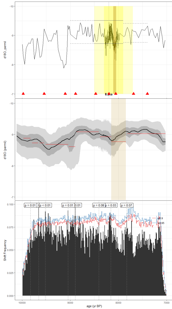
1250 Figure C7. As in Fig. C1, but for the speleothem record of Dykoski et al., 2005 (D4Dykoski). The published age model was constructed by linearly interpolating between U/Th dates. Here, we reconstruct the age model using the BACON algorithm in geoChronR.
