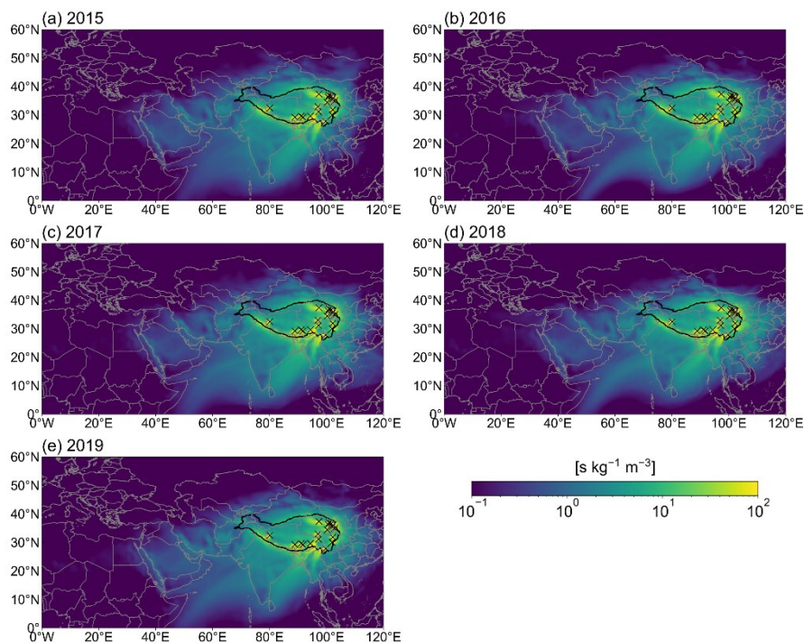
Figure 6 Distribution of the annual average residence time in the footprint layer for the 17 cities with MEE stations in (a) 2015, (b) 350 2016, (c) 2017, (d) 2018, (e) 2019. The crosses denote the locations of 17 cities.
