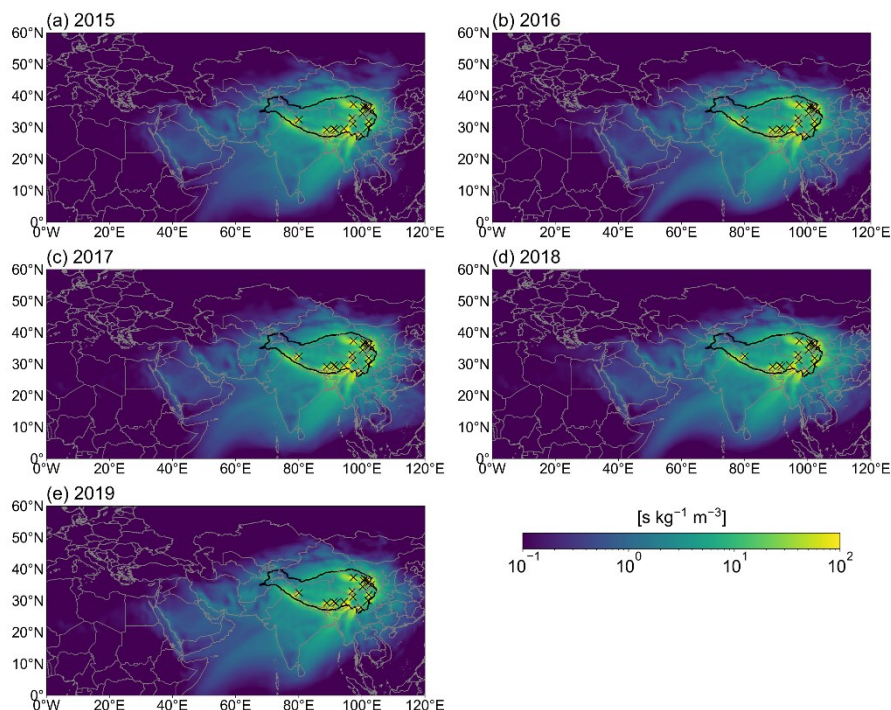
335 Figure 6 Distribution of the annual average residence time in the footprint layer for the 17 cities with MEE stations in (a) 2015, (b) 2016, (c) 2017, (d) 2018, (e) 2019. The crosses denote the locations of 17 cities.
