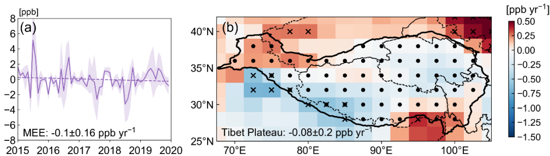
315 Figure 5 Changes in ozone mixing ratios due to changes in meteorology over 2015–2019 simulated by GEOS-Chem. (a) Deseasonalized monthly mean ozone averaged over the 17 cities with MEE measurements. (b) Spatial distribution of deseasonalized ozone trends over the plateau. In (b), the dots denote the grid cells belonging to the TP, and the crosses denote statistically significant ozone trends (p-value < 0.05).
