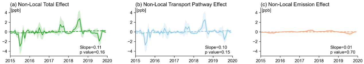
Figure 7 Deseasonalized monthly variation of non-local QNR averaged over the 17 cities. (a) Non-local QNR changes due to the combined effect of changes in anthropogenic emissions and in transport pathway. (b) Non-local QNR changes due to transport pathway alone. (c) Non-local QNR changes due to anthropogenic emissions alone. The shaded area represents the standard deviation of the data across 17 cities.
