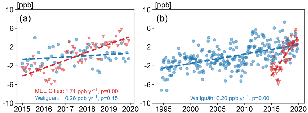
235 Figure 2 Monthly variation of deseasonalized ozone mixing ratios over the TP during (a) January 2015 to December 2019 and (b) August 1994 to December 2019 based on ground measurements. The results of MEE cities represent the mean of ozone mixing ratios in 17 cities. The data points represent deseasonalized ozone in individual months, and the dashed lines represent linear regression fit. The slope of linear regression and the p-value are also shown.
