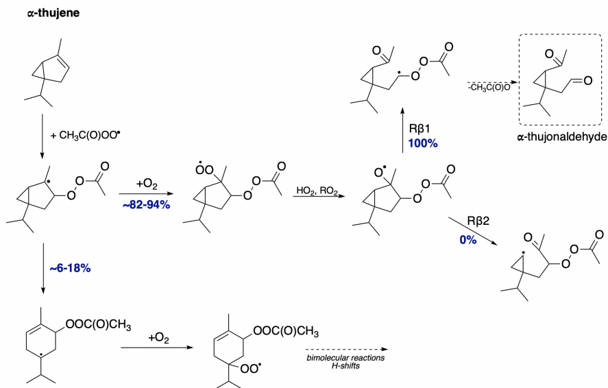
Figure 13. Proposed fate of \alpha -thujene + \text{CH}_3\text{C}(\text{O})\text{OO}\cdot . Dashed box present closed-shell product that terminates oxidation pathway.
