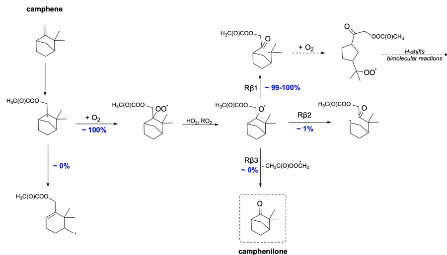
Figure 12. Proposed fate of camphene + \text{CH}_3\text{C}(\text{O})\text{OO}\cdot . Dashed box present closed-shell product that terminates oxidation pathway.
