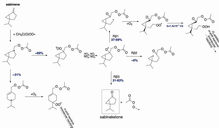
Figure 14. Proposed fate of sabinene + CH 3 C(O)OO·. Dashed box present closed-shell product that terminates oxidation pathway. The indicated yields for β-scission reactions depend on the stereoisomer (see Table 4)
